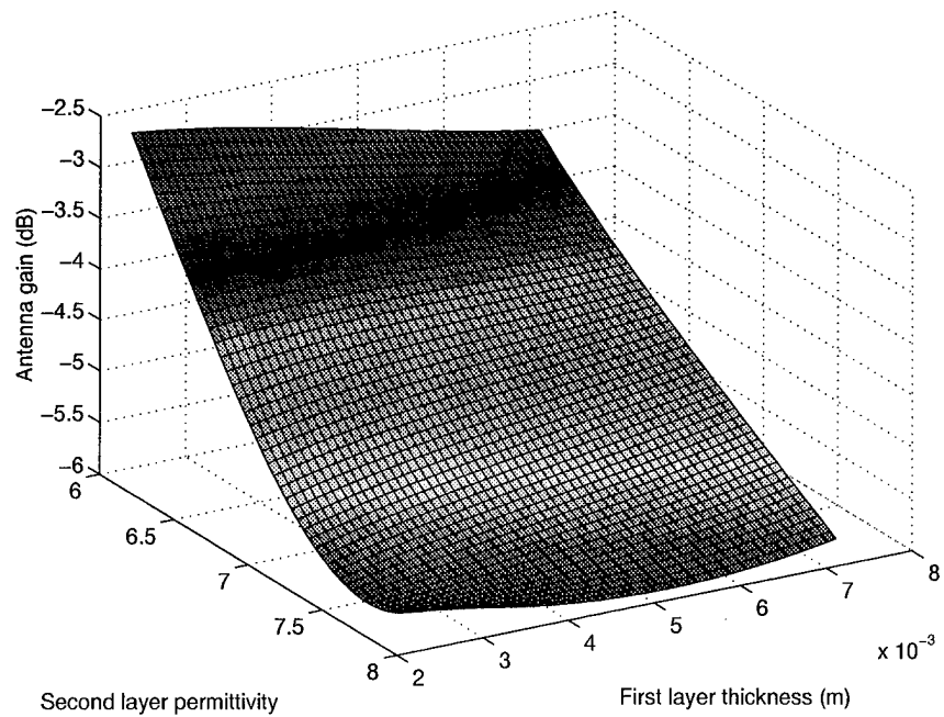
Figure 4.16 First Layer Thickness and Second Layer Relative Permittivity Effects Near the Optimized Location
