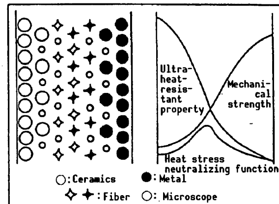
Figure 27. Depiction of Gradient Functions
