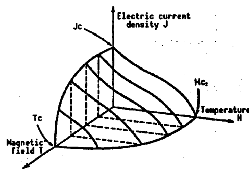
Figure 1. Superconducting T-J-H Critical Surface Plane
