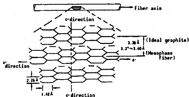
Figure 1. Approximate Orientation of Crystal Structure for Carbon Fiber (D.D. Edie 14 )
