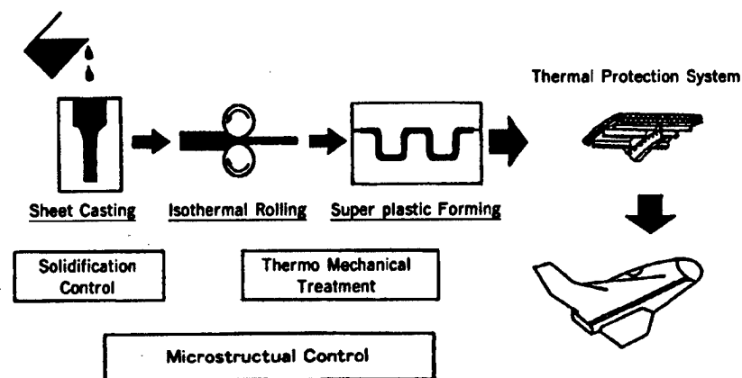
Figure 3. General Outline of Process To Make Thin Sheets Directly From Melt
