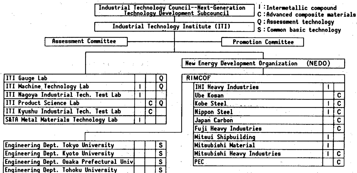
Figure 2. R&D Organization
