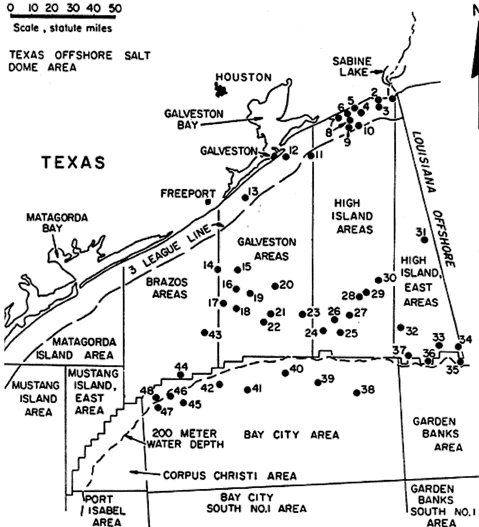
Figure 2 - Location of Texas Offshore Salt Domes (from Jirik and Weaver 1976)
