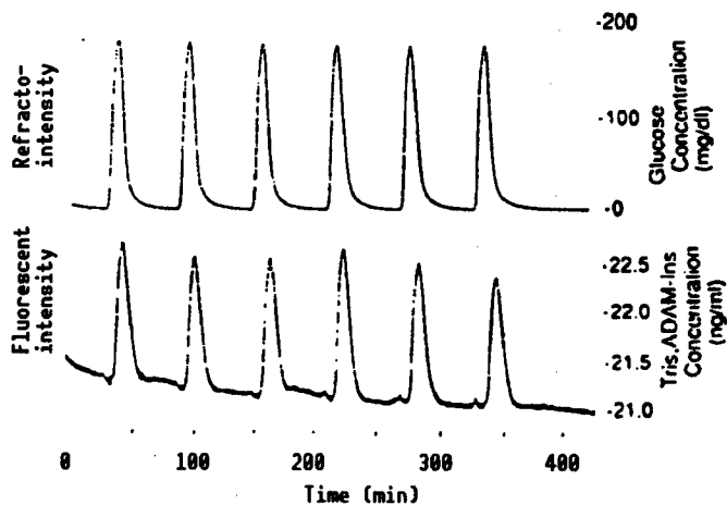
Figure 4. Release of Tris,ADAM-Insulin From Boronic Acid Gel
