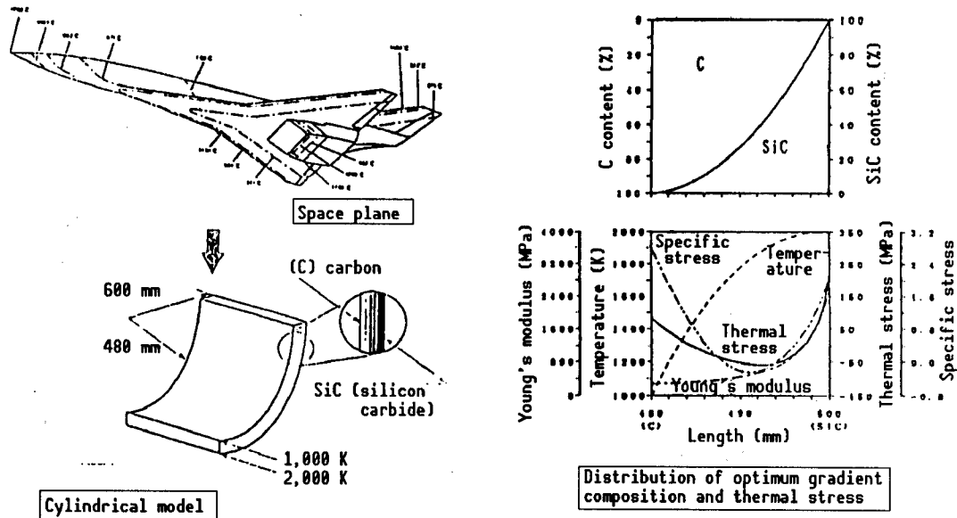
(Design example) Example of designing functionally gradient materials for external airframe wall of a space plane. The temperature of the external walls of the airframe is about 2,000 K, with a temperature difference from the internal surface of more than 1,000 K. The materials combined are SiC and C. The right-hand drawing shows gradient compositional distribution to minimize thermal stress generated in airframe external wall materials.
