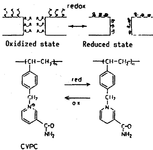
Figure 4. Oxidation/Reduction Responsive Grafted Membrane
