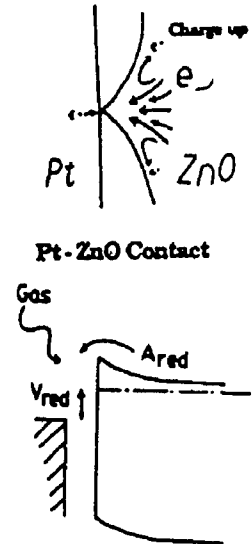
Figure 3. Presumed Short-Circuit Current Generating Mechanism
