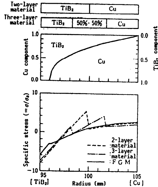
Figure 5. Effect of Thermal Stress Relaxation by Gradient Controlled Materials
