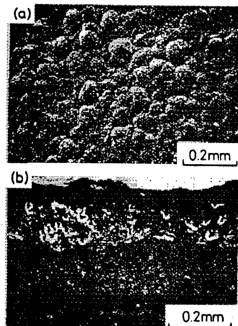
Figure 11. Texture Photograph of SiC/C-FGM After High-Temperature Difference Test
