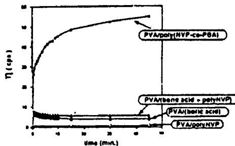
Figure 3. Time Dependence of Viscosity of PVA(88000)/Poly(NVP)-co-PBA(●), PVA(88000)/(Boric Acid + PolyNP)(●) PVA(88000)/Boric Acid(●) and PVA(88000)/PolyNVP(o) Complex System
