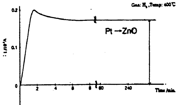
Figure 2. Short-Circuit Current Generated in Pt-ZnO Interface (Pt→ZnO is positive)
