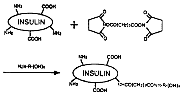
Figure 3. Schematic Structure of Insulin Hydroxylation
