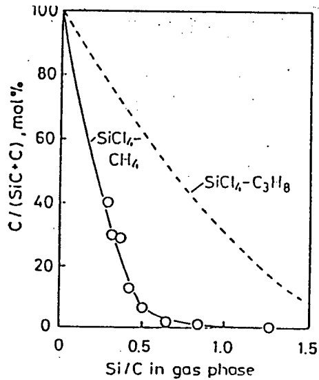
Figure 4.1.1. Relationship between the C content in SiC+C·NFGM and the density of material gas SiCl 4 -CH 4 : 1773K, 1.3 kPa SiCl 4 -C 3 H 8 : 1773K, 40 kPa
