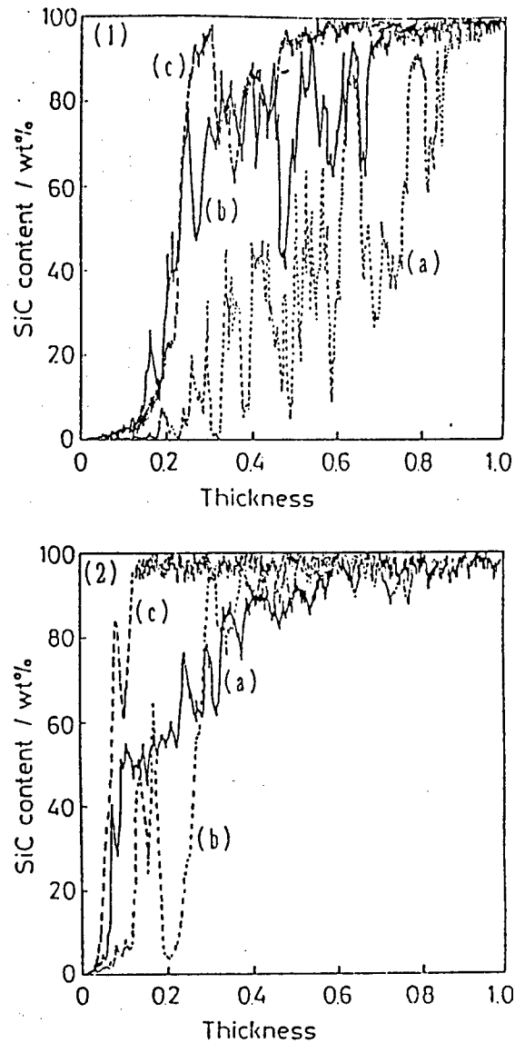
Figure 4.3.1. Composition distribution in the cross section of SiC/C-FCM
