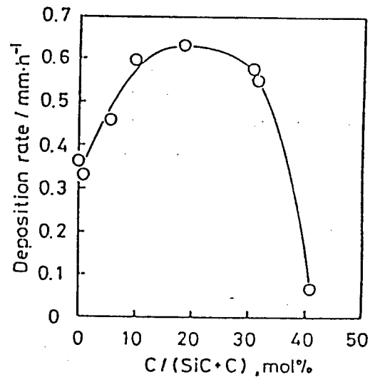
Figure 4.1.2. Growth speed of thickness of SiC+C·NFGM SiCl 4 -CH 4 : 1773K, 1.3 kPa
