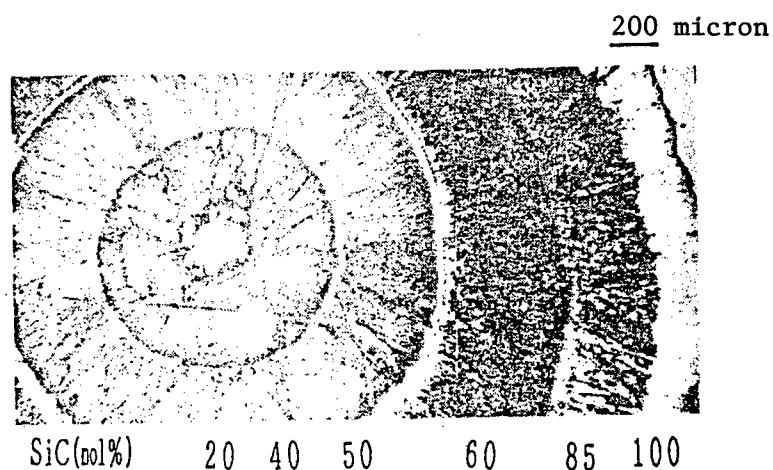
Figure 3.4.3. Six-step FGM formed on carbon fiber
