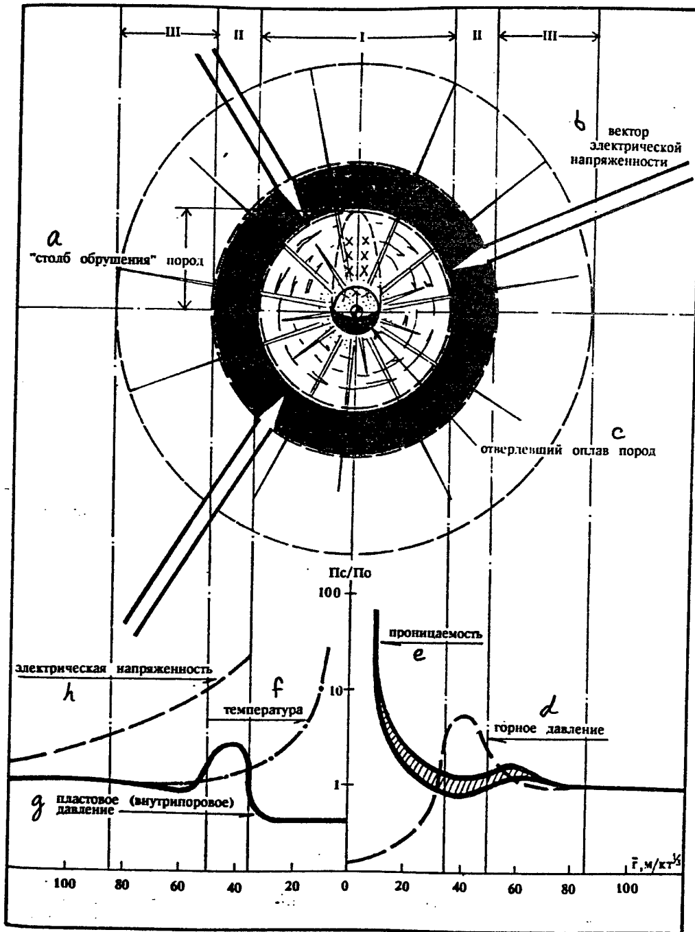
Above: schematic of physical and mechanical transformation of homogeneous porous rock affected by a camouflaged nuclear explosion. Three zones are isolated (central I, intermediate II, and external III) which differ in the degree of rock transformation, and which are used to achieve various technological ends. The arrows show the vectors of electric voltage in the region of anomalous electric polarization of the rock generated in the explosion. Below: graph reflecting the change in the basic properties of a porous medium (x-axis, effective radius, m/kt^{1/3} , y-axis, ratio of the "stimulated" parameter to the initial parameter).
