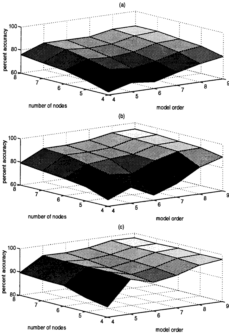
Figure 5.3: Accuracies of the neural net classifier versus model order and node count: (a) mean (b) median (c) maximum
