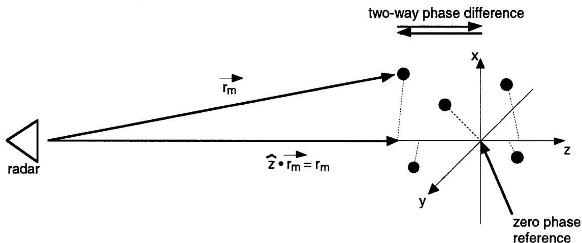
Figure 3.1: Diagram of the scattering centers in the far field
