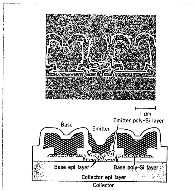
Figure 11. Cross Section of EBT (Epitaxial Base Transistor)
