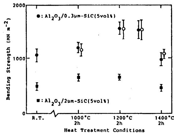
Figure 1. Effects of Heat Treating on the Breaking Strength of \text{Al}_2\text{O}_3/\text{SiC} Composites ■: in air ○: in Ar
