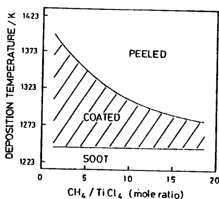
Figure 1. Area of TiC Formation
