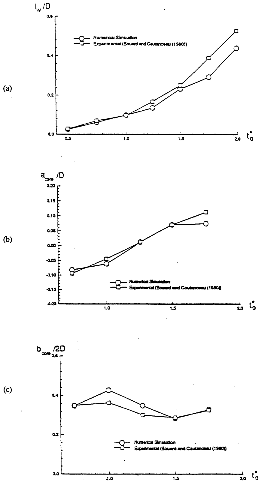
Figure 8 Graphical comparison of computed and experimental measurements of wake quantities for the case of Re_D = 9500 ; (a) l_w / D , (b) a_{core} / D , and (c) b_{core} / 2D .
