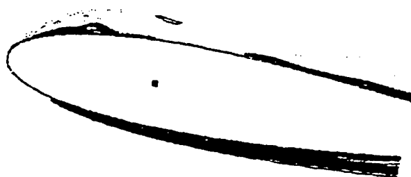
a) Initial leading edge separation
