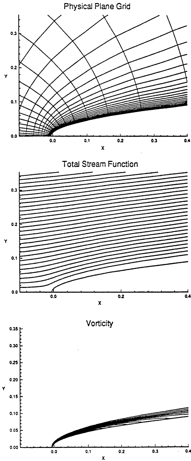
Figure 5: Physical Plane Results for Re_\tau = 100 .
