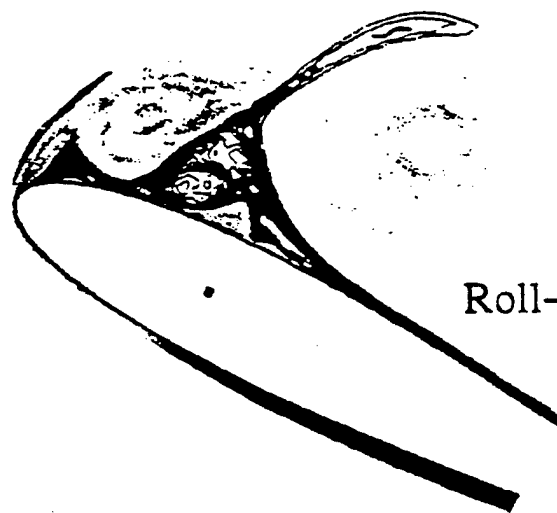
d) Inviscid Interaction
