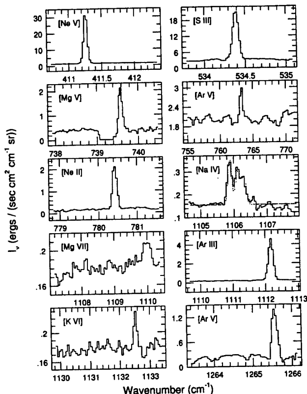
FIG. 2.—Dereddened spectra for the 12 emission lines detected in NGC 7027. Wavenumbers are presented in Table 1, and uncertainties are discussed in § 3. The dotted line in the [Na iv] plot denotes our model fit for the hyperfine splitting. The [Na iv] energy splittings were determined by scaling from the hyperfine measurements of [^{17}\text{O} \text{ I}] by Harvey (1965) and from the fine-structure splittings of [\text{O} \text{ I}] and [\text{Na} \text{ IV}] . Relative line intensities were calculated using the formulae of Townes & Schawlow (1955). The spectrum has been convolved to have the same resolution as the [Na iv] data.
