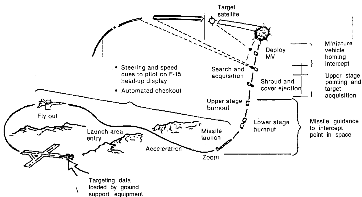
Figure 4-10.—ASAT Mission Profile
