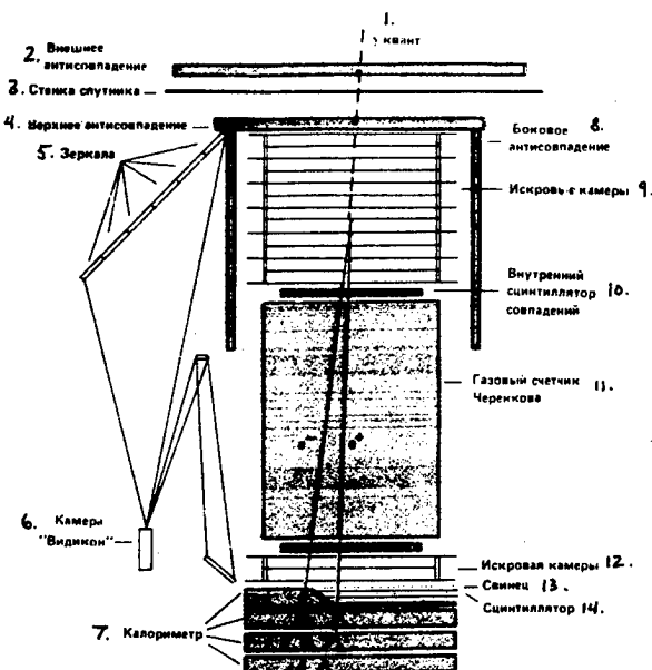
Diagram of structure and operating principle of "Gamma-1" telescope.
