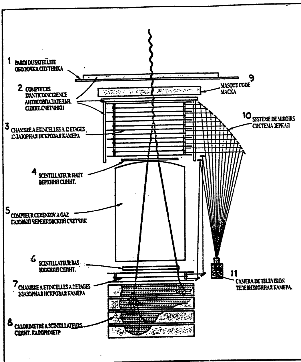
Diagram of Gamma telescope.
