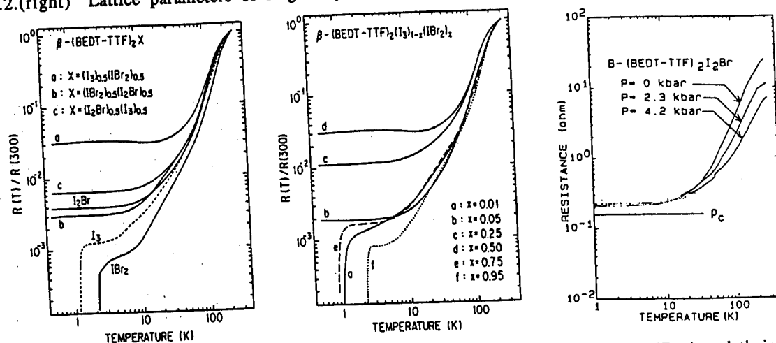
Fig.3. Temperature dependence of resistance. (a) \beta-(\text{BEDT-TTF})_2\text{X} ( \text{X}=\text{I}_3, \text{I}_2\text{Br}, \text{IBr}_2 ) and their 1:1 mixed crystals. (b) \beta-(\text{BEDT-TTF})_2(\text{I}_3)_{1-x}(\text{IBr}_2)_x . (c) pressure effect on \beta-(\text{BEDT-TTF})_2\text{I}_2\text{Br} .
