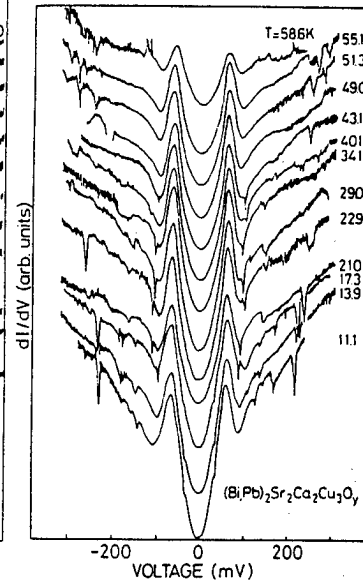
Fig.2 Temperature variation of dI/dV raw data for (\text{Bi,Pb})_2\text{Sr}_2\text{Ca}_2\text{Cu}_3\text{O}_y up to T=58.6\text{K} .
