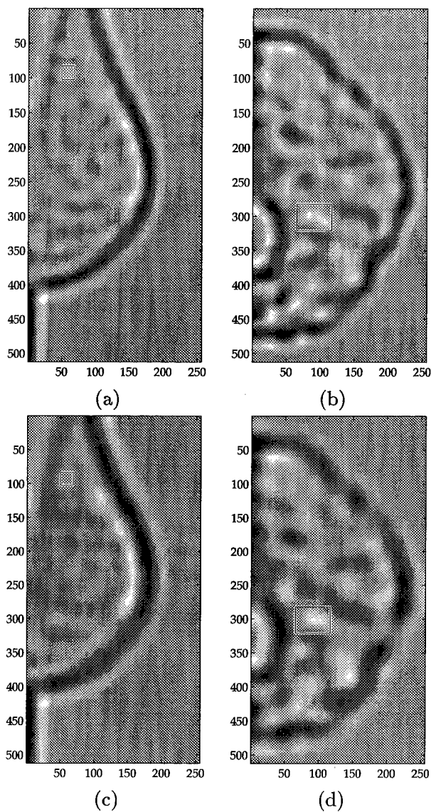
Figure 13 (a) and (b) are the result of DOG filtering with a dogsized of 20. (c) and (d) were created by filtering with a dogsized of 30. Through the course of these two figures, the size restriction of a DOG filter can be seen. The mass in a001d00m was best found using a smaller DOG kernel. The mass in a002b00m needed a larger DOG kernel to be properly identified.
