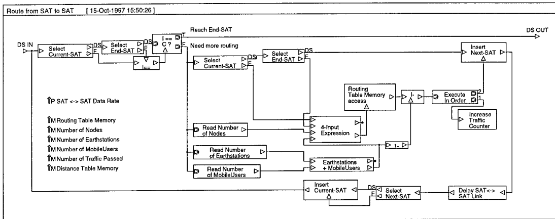
Figure 24 Route from SAT to SAT
