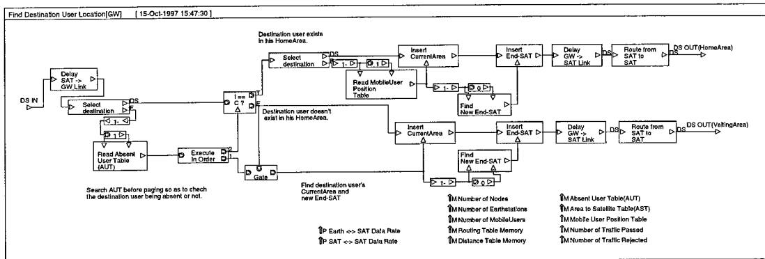
Figure 36 Find Destination User Location[GW]
