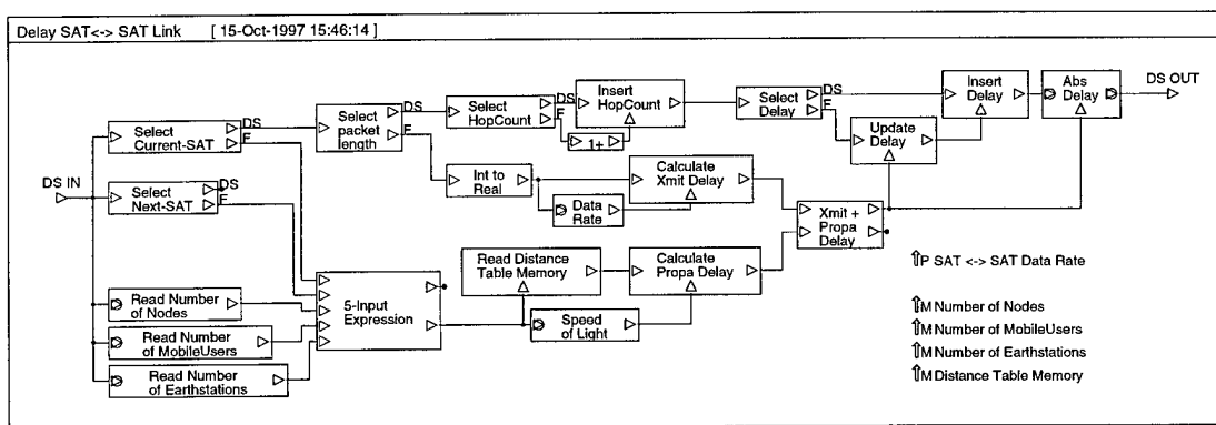
Figure 25 Delay SAT ↔ SAT Link
