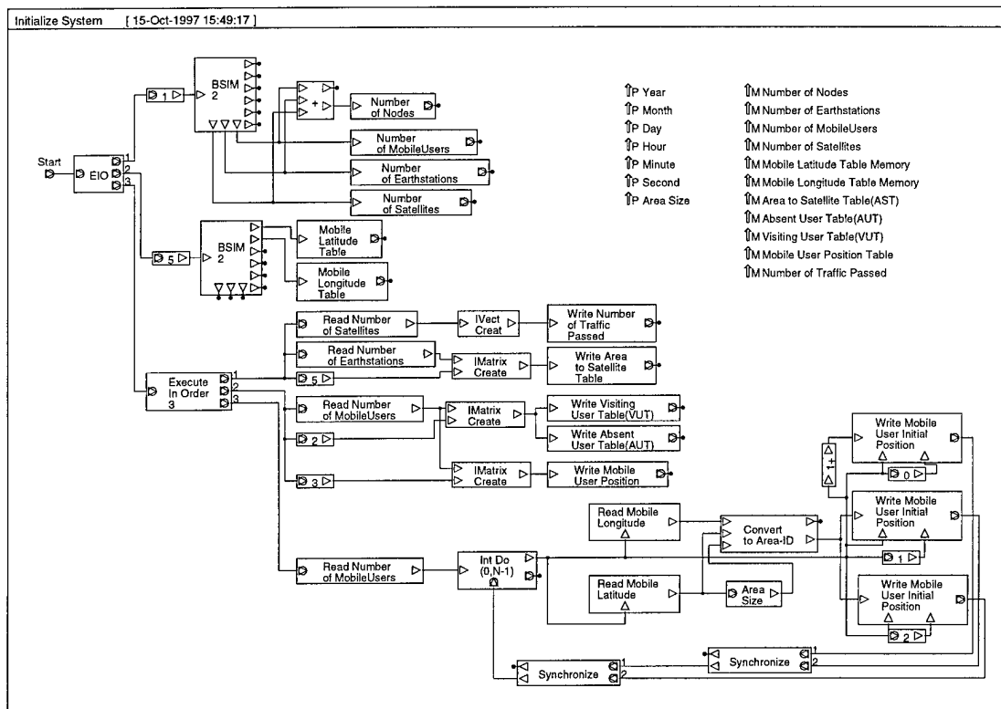
Figure 5 Top level block diagram of the Gateway Approach.
