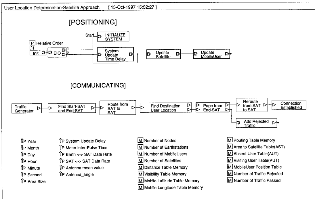
Figure 13 User Location Determination-Satellite Approach
