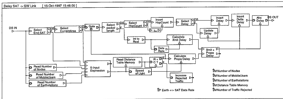
Figure 37 Delay SAT→GW Link
