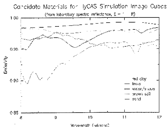
Figure 13. Emissivity values for selected endmember materials. The emissivity values are derived from the spectral reflectance values shown in Figure 12. Only the 8–12 \mu\text{m} spectral region is displayed.
