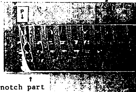
Figure 5. Damages Produced by W.O.F.-Test for 3DCM
