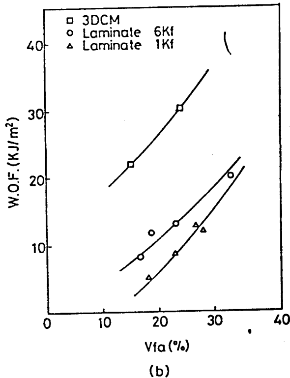
Figure 4. W.O.F. Measurement by a Chevron-Notch Three-Point-Bending Test—(a) Comparison between 3DCM and a flatwise laminate; (b) Comparison between 3DCM and an edgewise laminate
