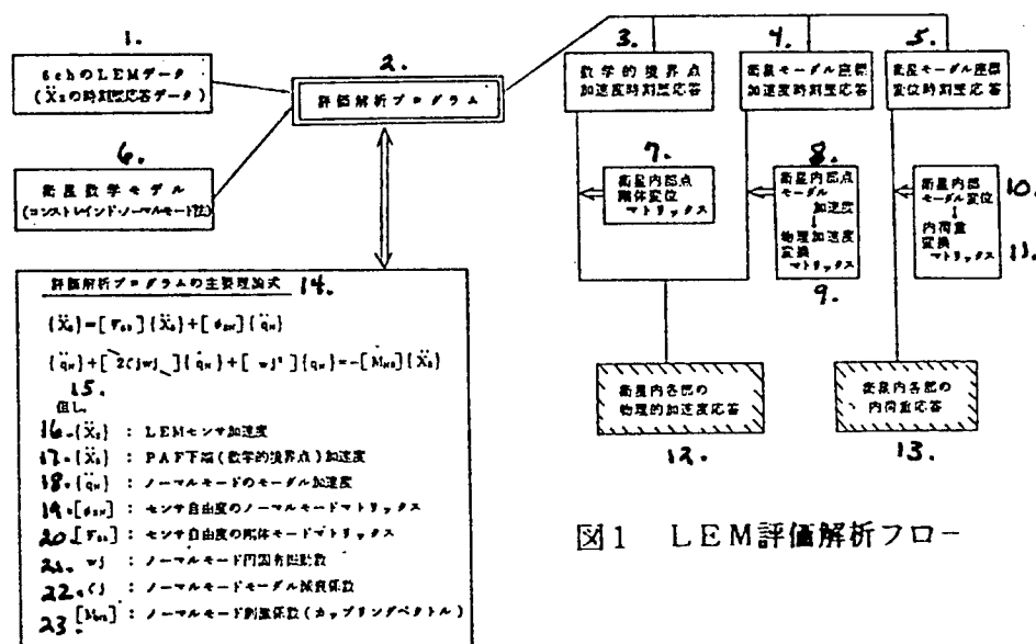
Figure 1. LEM Evaluation and Analysis Flow
