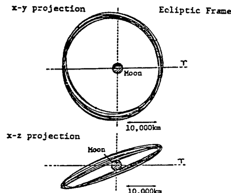
Figure 2. Example of Orbit of Lunar Orbiter
