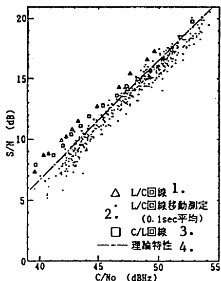
Figure 5. ACSSBC/No to S/N Characteristics Key: 1. L/C line 2. Measurement of movement of L/C line (0.1 sec on average) 3. C/L line 4. Theoretical characteristics
