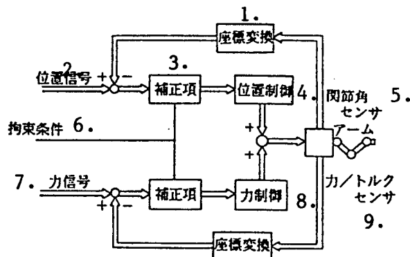
Figure 2. Hybrid Control System
