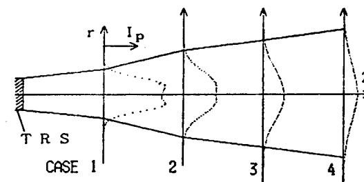
Figure 4. Results of Measuring Angle of Beam Divergence
