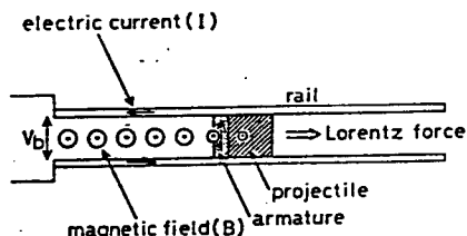
Figure 1. Principle of Rail Gun
