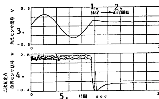
Figure 3. Time History of Capture Tracking
