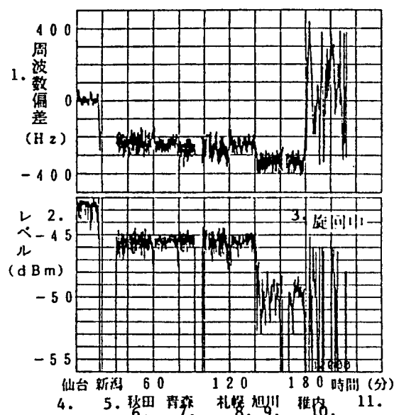
Figure 4. Change in Signal Level and Frequency (B99)
