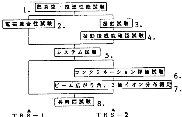
Figure 1. Test Flow
