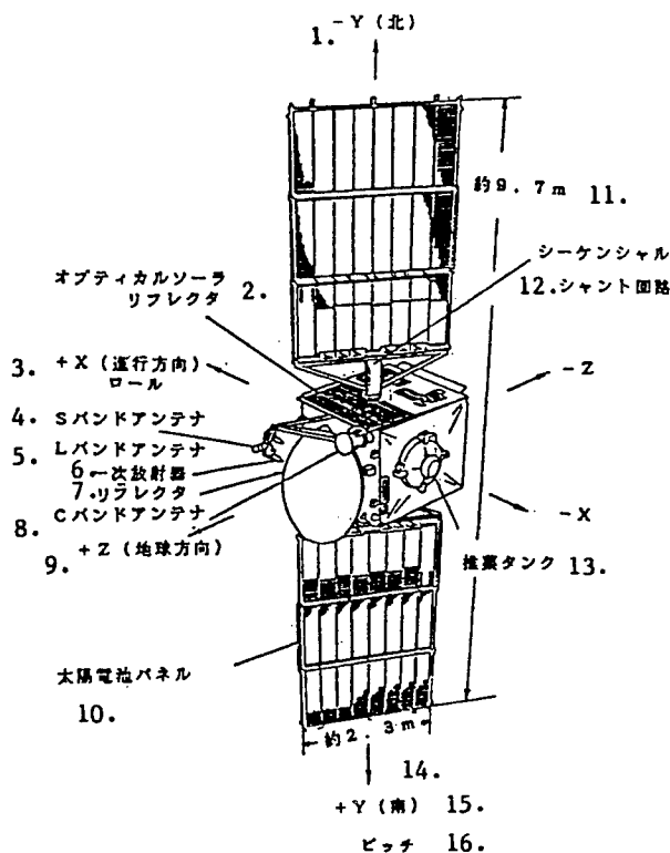
Figure 1. View of ETS-V
