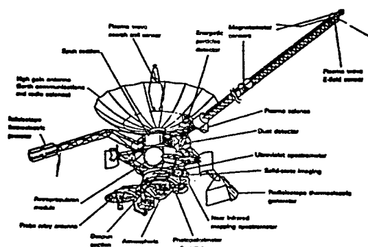
Figure 3. Galileo Spacecraft from NASA SP-479
