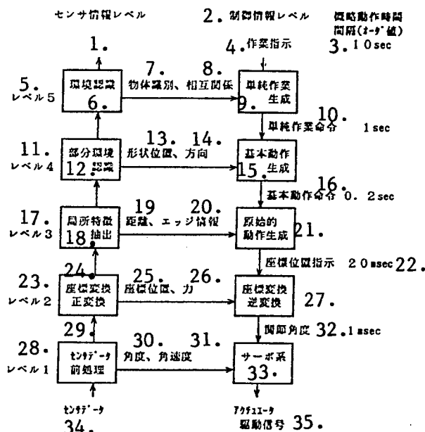
Figure 1. Sensor Information and Control Level Hierarchy
