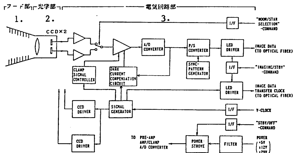
Figure 1. Schematic Flow Diagram of ONS
