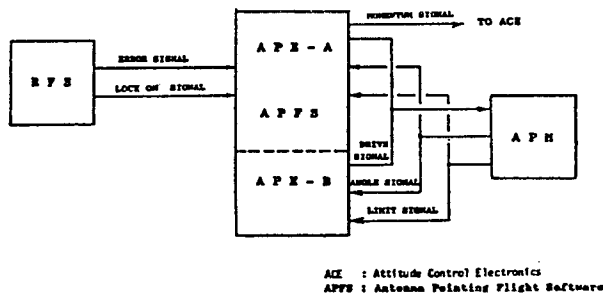
Figure 1. Subsystem Configuration
