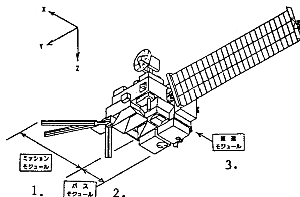
Figure 2. Example of Configuration in Orbit
