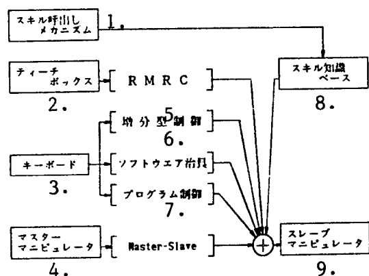
Figure 1. Skillfulness Superposition Mechanism
