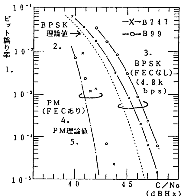
Figure 6. BER Characteristics
