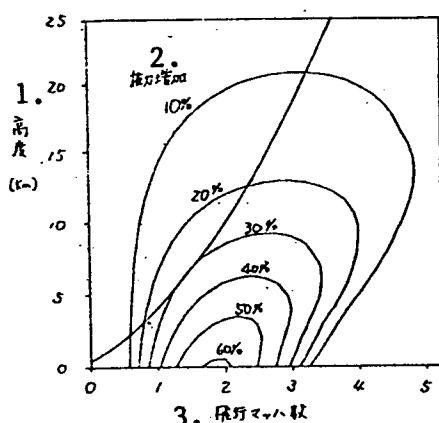
Figure 3. Launch Orbit and Increase in Thrust
