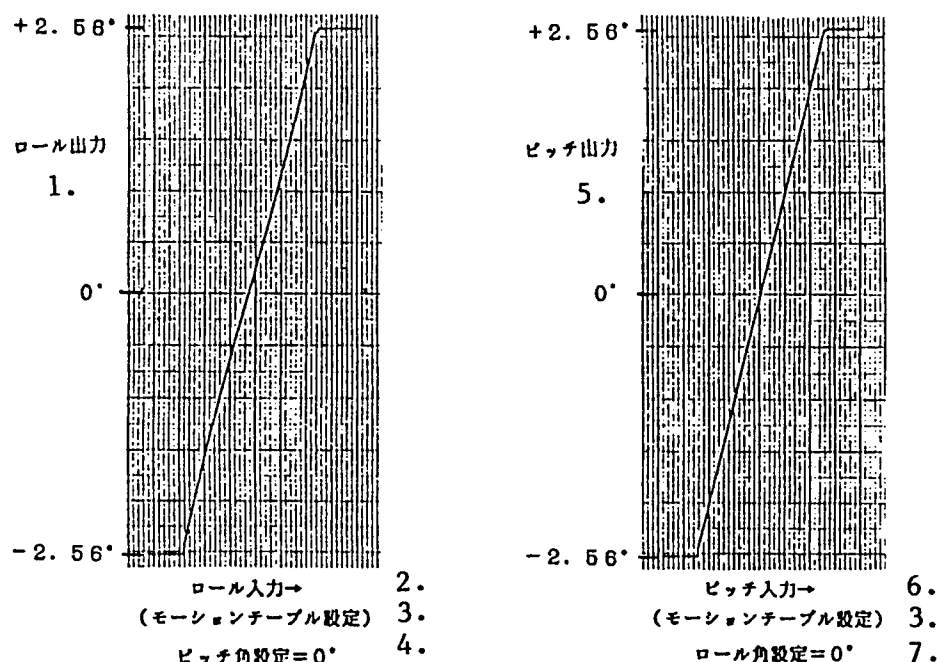
Figure 3. Roll/Pitch Transfer Characteristics (Geostationary Altitude)
