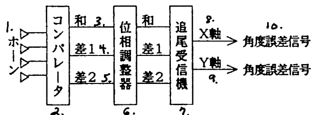
Figure 1. RF Sensor System
