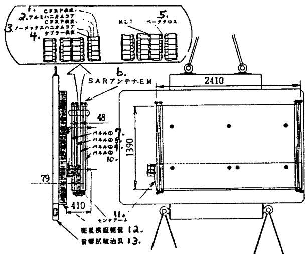
Figure 1. Specimen
