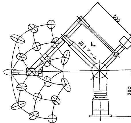
Figure 1. Distribution of Mass Ellipsoids (Space Master Arm)
