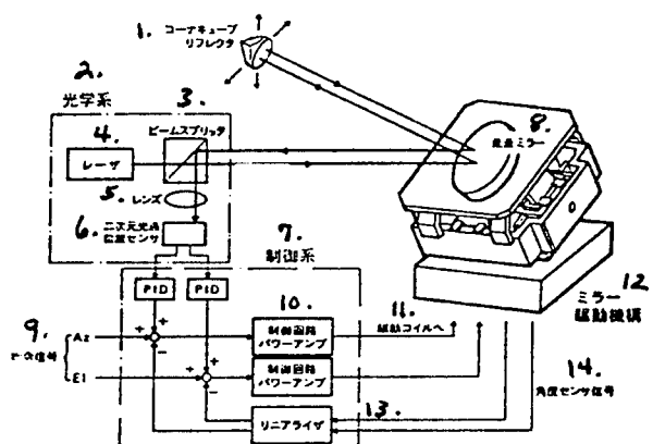
Figure 1. Configuration of Capture Tracking System
