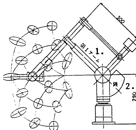
Figure 2. Distribution of Mass Ellipsoids (Ground Master Arm)
