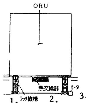
Figure 3. Cross-sectional Structure
