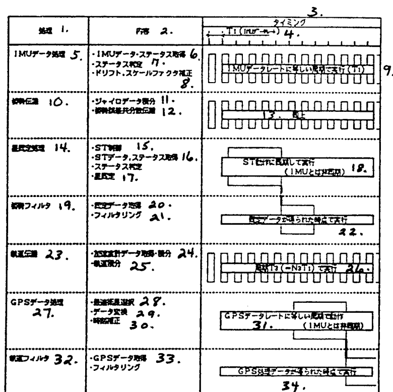
Figure 2. Navigation Software Contents
