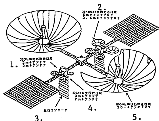
Figure 2. An Example of 16-Ton-Class GPF (5)
