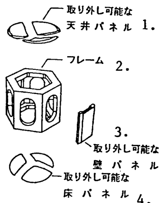
Figure 1. Module Shape
