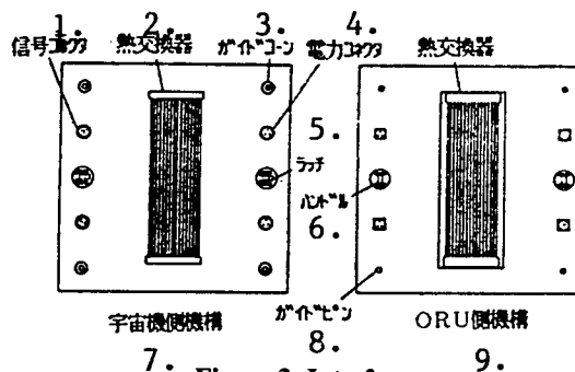
Figure 3. Interface
