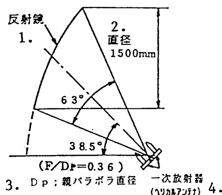
Figure 1. Configuration of Antenna
