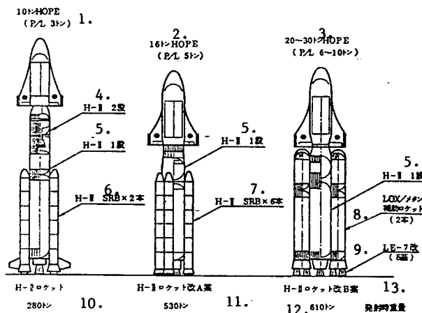
Figure 1. Examples of H-II Rocket (Including Improved Model) and HOPE
