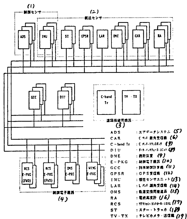
Figure 1. Guidance and Control Equipment
