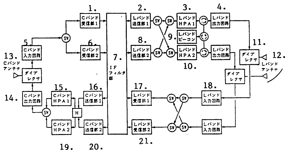
Figure 1. Block Diagram of AMEX
