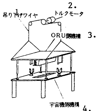
Figure 4. Test Configuration
