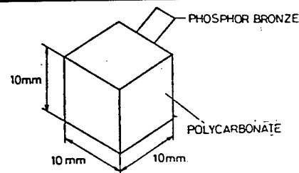
Figure 3. Projectile
