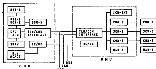
Figure 1. TEDA Functional Block Diagram
