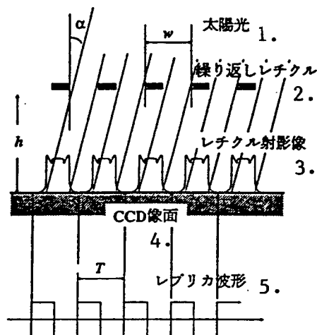
Figure 1. Principle Drawing
