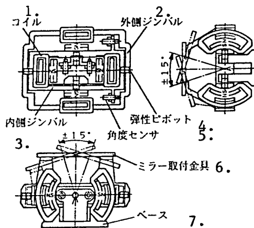
Figure 2. Outline of Mirror Driving Mechanism Structure
