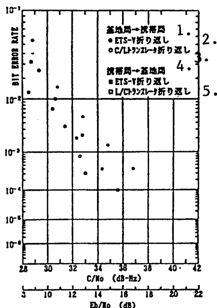
Figure 4. BER of Message Communications System Key: 1. Base station to portable mobile station 2. Turn of ETS-V 3. Turn of C/L translator 4. Portable mobile station to base station 5. Turn of L/C translator
