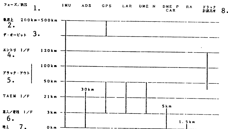
Figure 2. Navigation Support Equipment Use Phase
