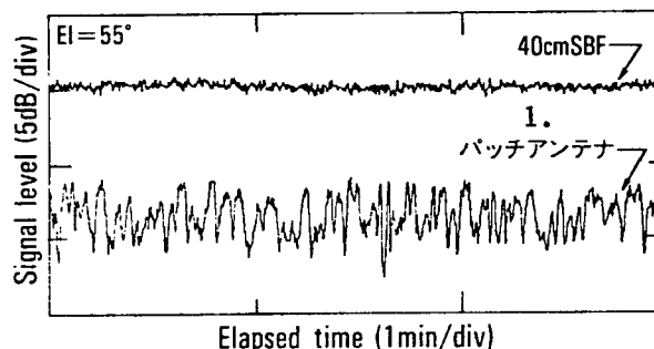
Figure 2. Example of Propagation Characteristics Obtained from Use of Circular Patch Antenna (Ship Experiment)
