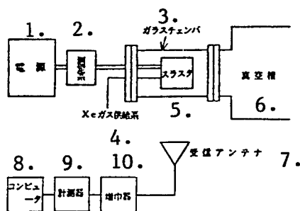
Figure 3. Electromagnetic Adaptability Test Configuration
