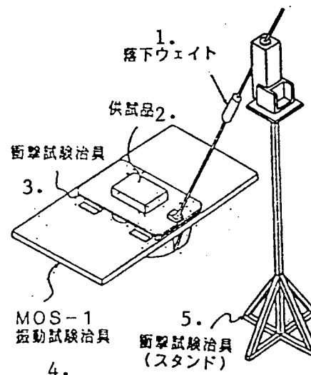
Figure 2. Impact Test
