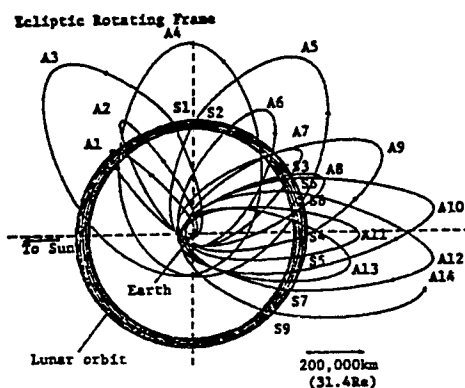
Figure 1. Example of Orbit of MUSES-A
