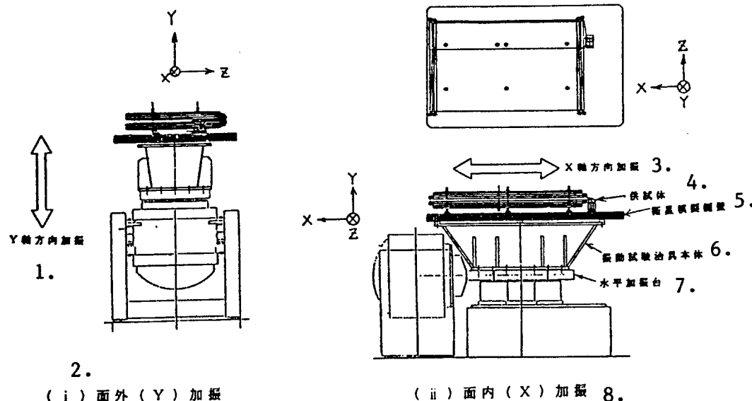
Figure 1. Vibration Test Configuration
