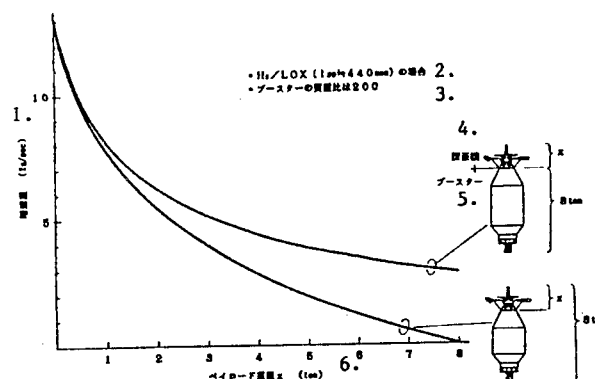
Figure 1. Relationship Between Speed Increase and Weight of Probe According to Launch System
