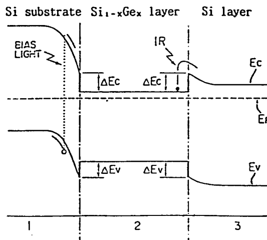
Figure 1. Principle of Operation of Hetero-type Device
