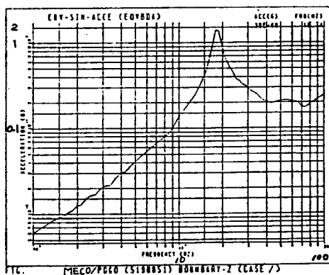
Figure 2. Axial Direction (Z Direction) at MECO/POGO. PAF lower end equivalent sine wave vibration conditions.
