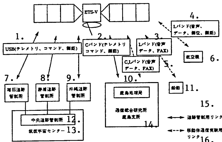
Figure 1. Tracking Control System of ETS-V
