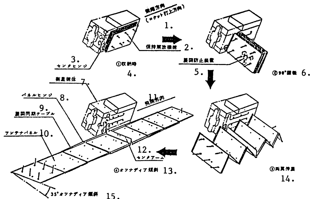
Figure 1. Unfolding Operation Sequence
