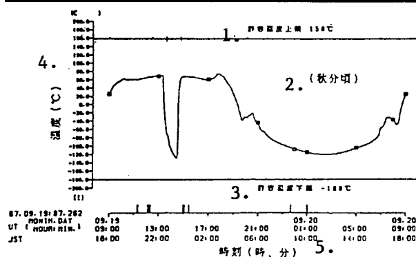
Figure 4. Actual Temperatures of Reflecting Mirror Measured at Check-Out
