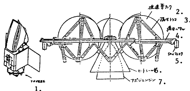
Figure 1. Sketch of Two-Liquid-Type Apogee Propulsion System
