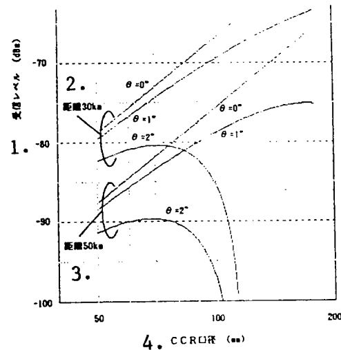
Figure 3. Optical Characteristics and Receiving Level of CCR
