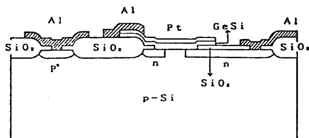
Figure 2. Cross-sectional Drawing of Element
