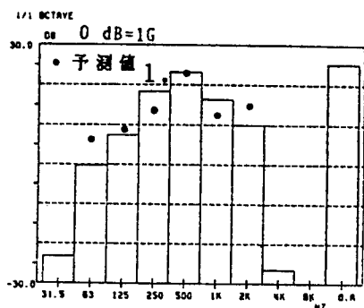
Figure 4. Panel (1) Response Acceleration
