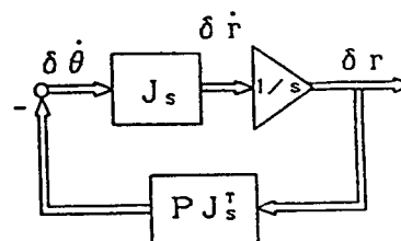
Figure 1. Example of Control Law Used in Experiment
