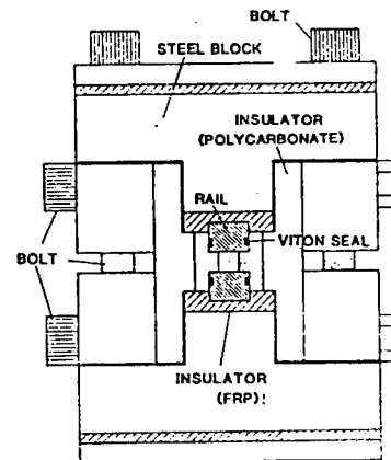
Figure 2. Cross Section of Rail Gun
