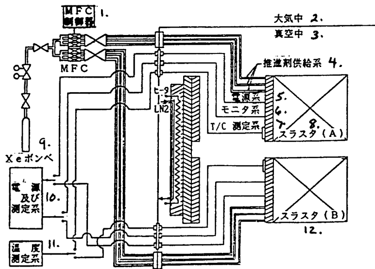
Figure 2. Test Configuration
