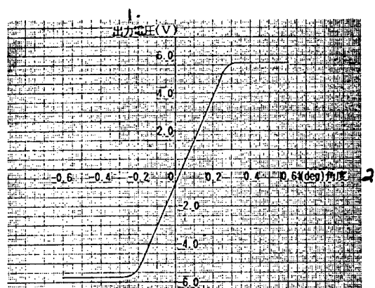
Figure 4. Output of Tracking Receiver
