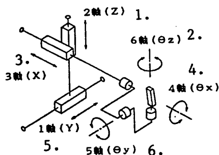
Figure 1. Configuration of Degree of Freedom of Master
