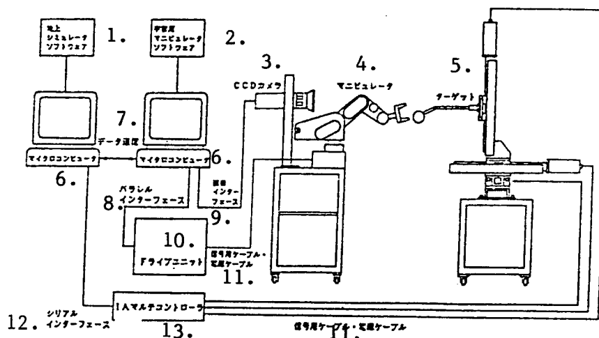
Figure 2. Block Flow Diagram of Ground Simulator System
