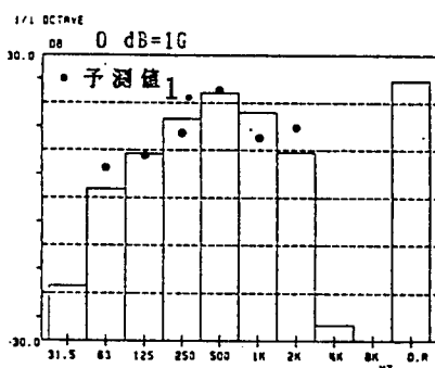
Figure 6. Panel (5) Response Acceleration
