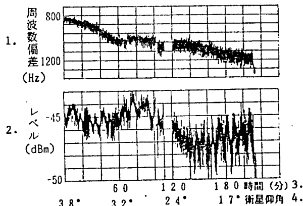
Figure 2. Change of Signal Level and Frequency (Boeing 747)
