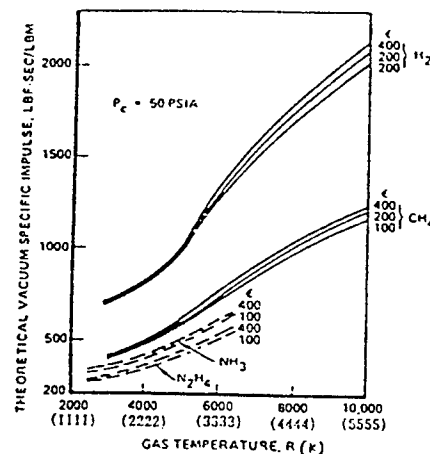
Figure 1. Theoretical Vacuum Specific Impulse Variation (1)
