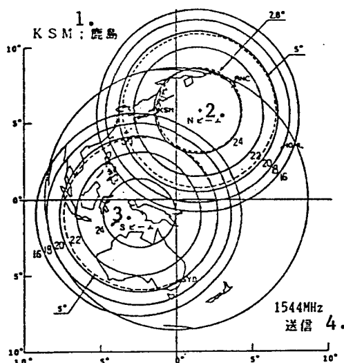
Figure 3. Secondary Radiation Pattern (Actual Measurement of Simple PFM Substance)
