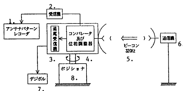
Figure 2. Measurement Configuration
