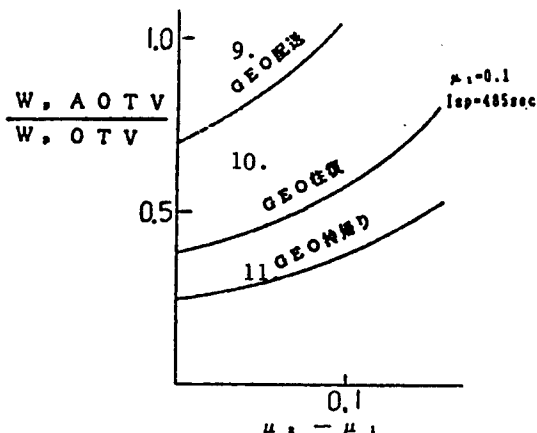
Figure 1. Fuel Weight Ratio of AOTV/OTV
