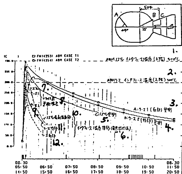
Figure 3. Temperature of Surface of Apogee Motor
