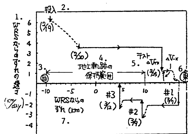
Figure 3. Change of Deviation from WRS
