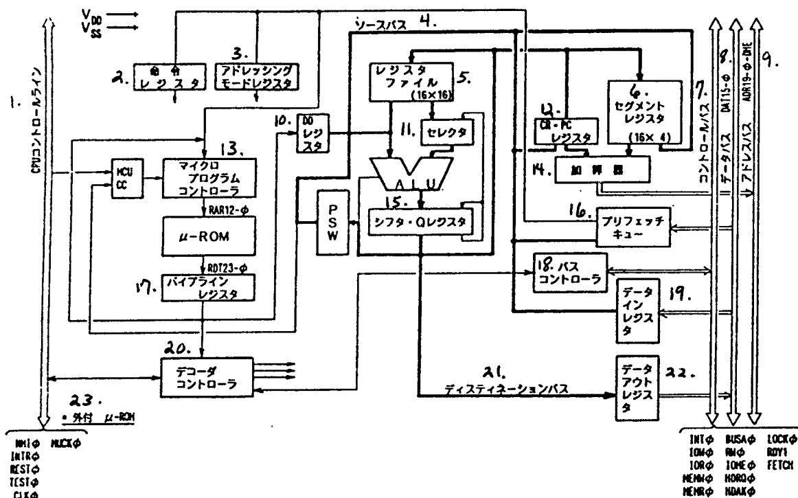
Figure 2. 16-Bit MPU Functional Block Diagram
