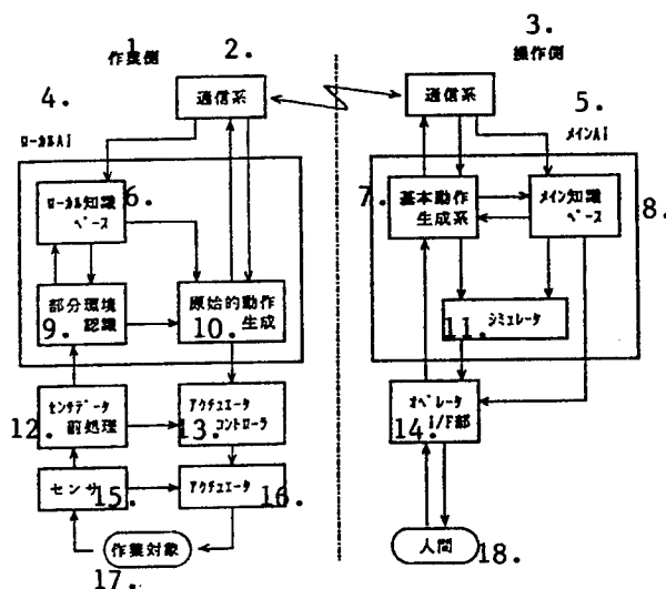
Figure 2. Example of Configuration of Autonomously Teleoperated System
