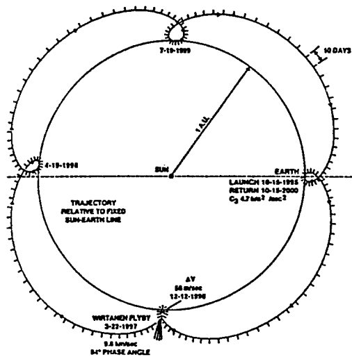
Figure 1. Orbit of Wirtanen Mission
