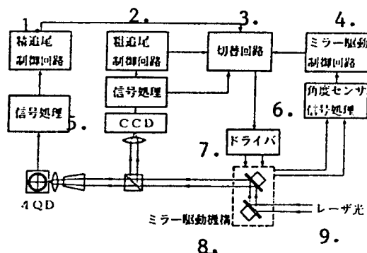
Figure 1. System Configuration of Tracking System Experimental Unit
