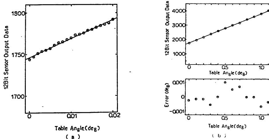
Figure 3. Transfer Characteristic Rate
