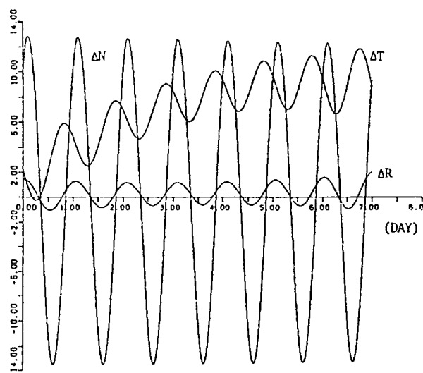
Figure 1. Orbit Positional Error (Estimated Value - True Value) (unit: meters)
