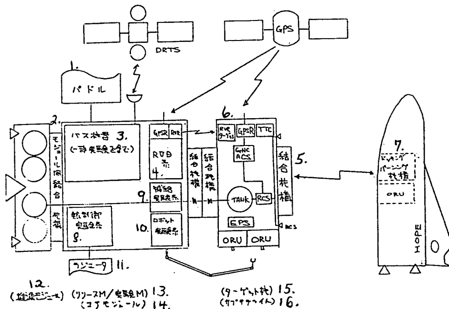
Figure 1. System Block Diagram of STEP
