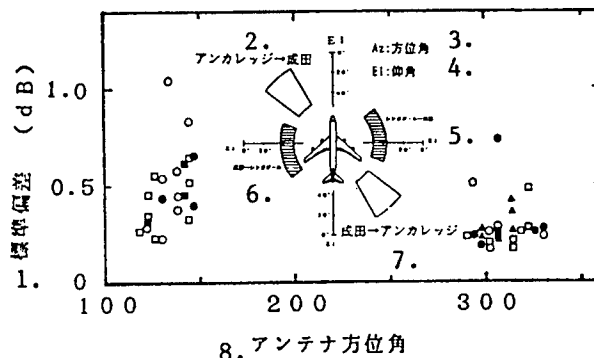
Figure 3. Standard Deviation of Electric Power Received by Aircraft Earth Station
