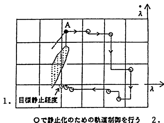
Figure 4. Plan for Geostationary Status When Point A Is Involved
