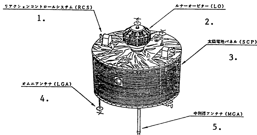
Figure 3. Appearance of MUSES-A
