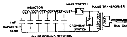
Figure 4. Circuit Diagram of Power Supply
