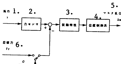
Figure 4. Hybrid Master Control System
