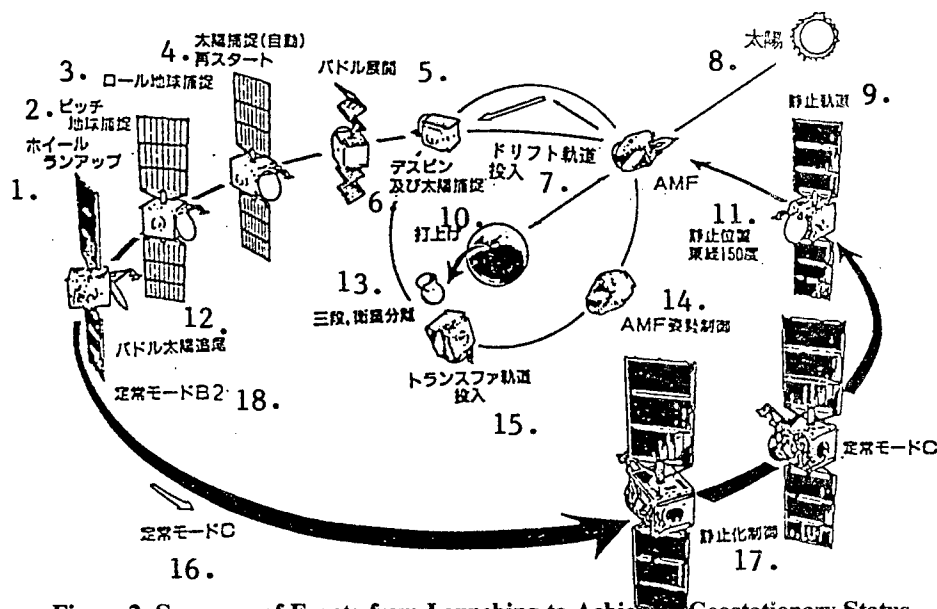
Figure 2. Sequence of Events from Launching to Achieving Geostationary Status
