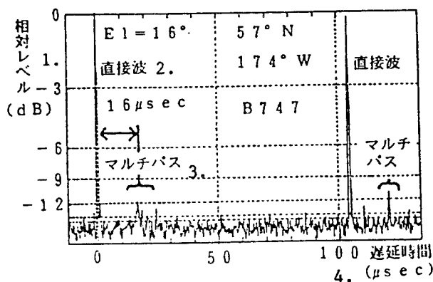
Figure 3. Example of Measurement of Multi-Pulse Electric Power Against Delay Time
