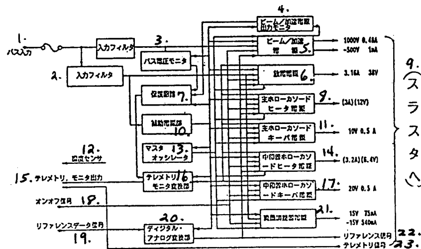
Figure 1. Block Diagram of Power Source Unit
