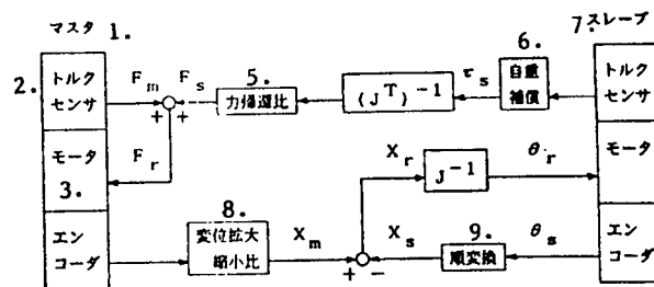
Figure 2. Control Block Diagram
