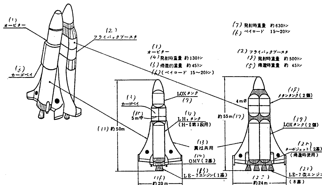
Figure 2. Vertical Take-off Reusable Two-Stage Rocket (Plan)
