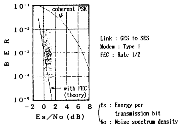
Figure 1. Example of Error Rate Characteristics of Communications Equipment with 64 Kbit/s (Ship Experiment)
