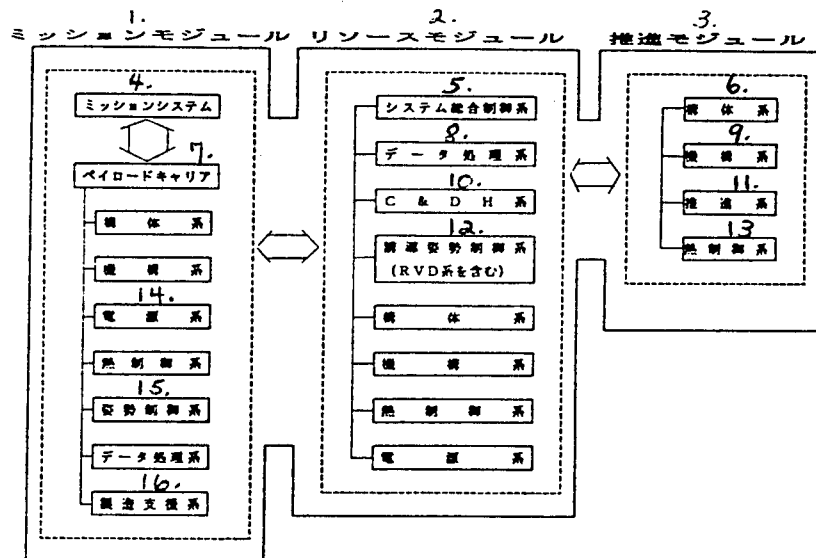
Figure 1. System Configuration of Space Factory
