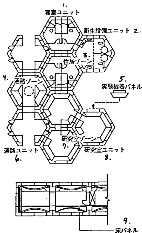
Figure 2. Module Layout
