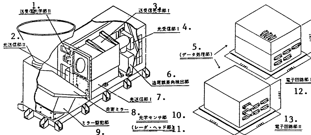
Figure 2. Conceptual Drawing of Laser and Radar Equipment
