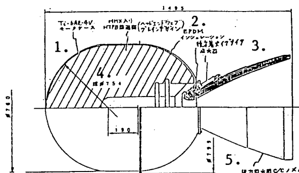
Figure 1. Sketch of Apogee Motor for ETS-V
