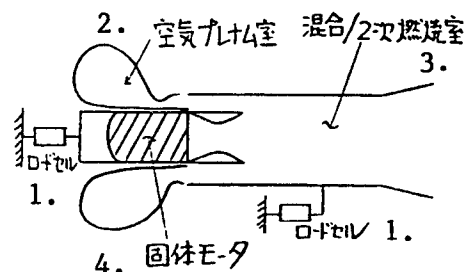
Figure 4. Conceptual Drawing of Basic Test
