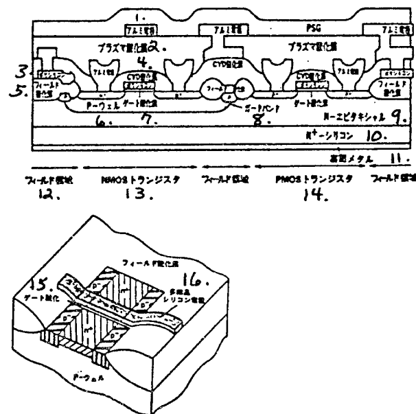
Figure 1. Cross-Sectional Drawing of 16-Bit MPU Pellet
