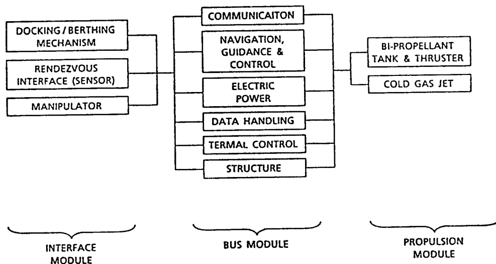
Figure 1. Block Diagram of the Initial OSV
