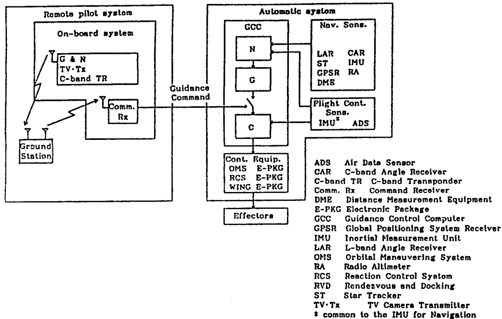
Figure 1. Guidance and Control System Configuration (Except for RVD Phase)
