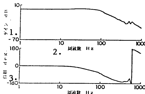
Figure 3. Frequency Response of Mirror Driving Mechanism
