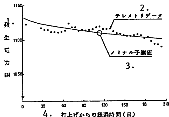
Figure 2. Electric Power Generated from Solar Cell Paddle
