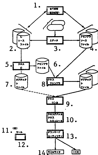
Figure 3. Software Development Procedure
