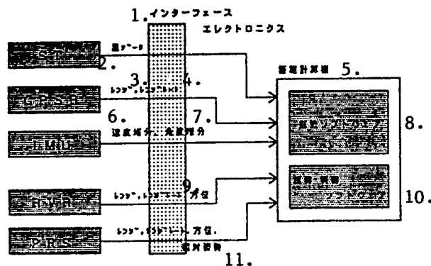
Figure 1. Configuration of Navigation System
