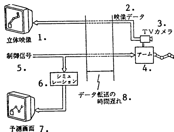
Figure 1. Indication on Predicted Screen
