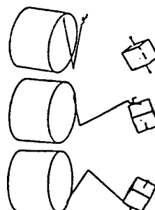
Figure 2. When System Has Angular Momentum
