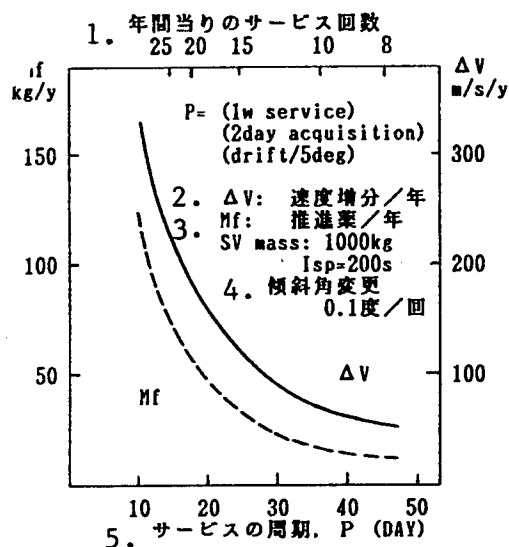
Figure 1. GEO-SV Service Capabilities
