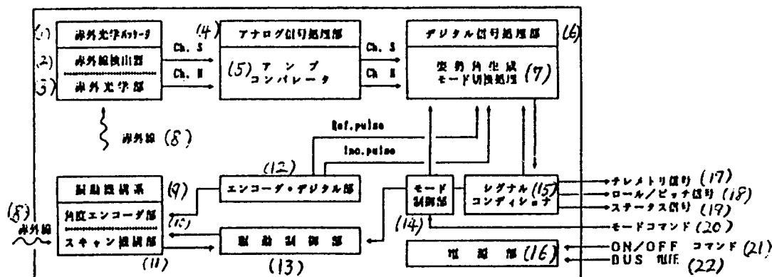
Figure 2. Functional Block Configuration
