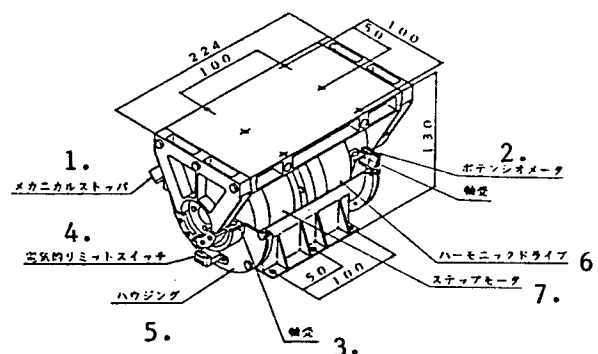
Figure 1. Sketch of APM's EM-1
