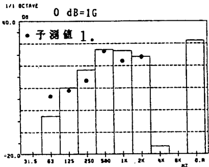
Figure 3. Panel (8) Response Acceleration Key: 1. Predictor
