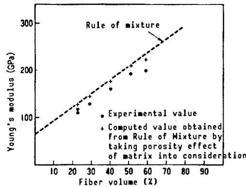
Figure 6. Fiber Volume Percentage Dependence of Young's Modulus of C Continuous Fiber Reinforced Glass 5
