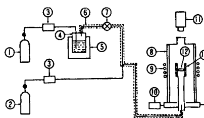
Figure 1. Chemical Vapor Deposition (CVD) Device Used for Functionally Gradient-izing the Composition
