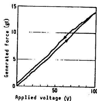
Figure 7. Generated Force
