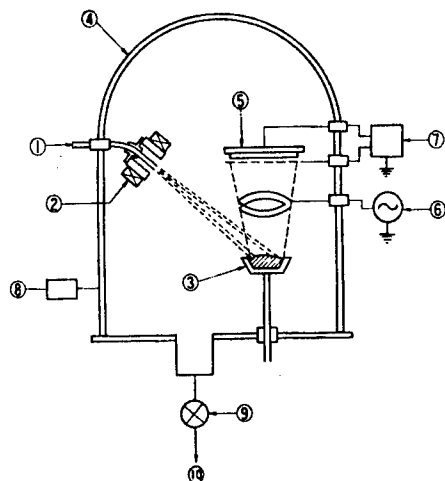
Figure 2. High Frequency Ion Plating (PVD) Device Used for Functionally Gradient-izing the Composition
