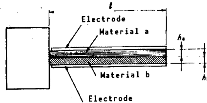
Figure 4. Calculation Model
