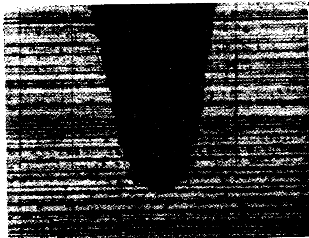
Fig.3. A feature of the V-notch for \text{Si}_3\text{N}_4 .
