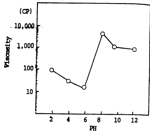
Fig. 2. Viscosity of mullite slip at constant shear rate of 3 sec -1 as a function of equilibrium pH.
