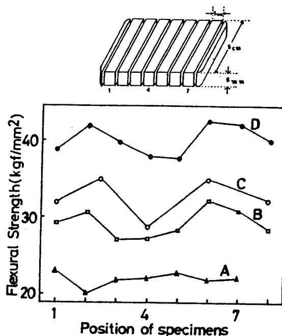
Fig. 4 Variation of the flexural strength of sintered \text{Al}_2\text{O}_3 with the positions of specimens. (A) stirrer (B) automatic agate mortar (C) ceramic three roll mill (D) ball mill
