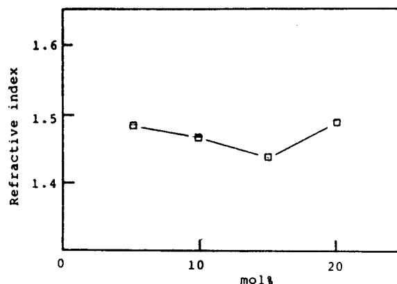
Fig. 7. Refractive index of B_2O_3-SiO_2 films as a function of the molar proportion of B_2O_3 .
