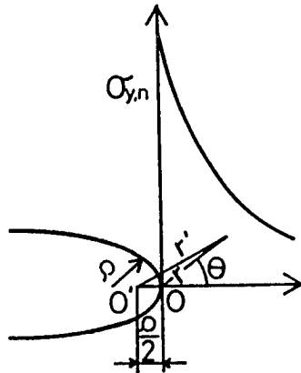
Fig.1. Coordinate around a notch tip.
