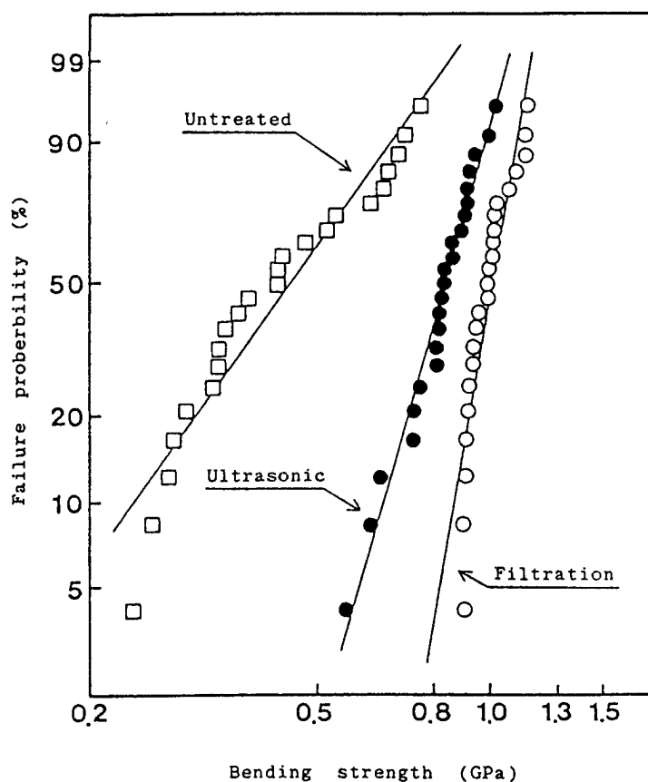
Fig. 2 weibull's plots of bending strength of 30 wt% SiC(w)-Al 2 O 3 composite with as-received(□), ultrasonic-treated(●) and 3 filtered(O) whisker.
