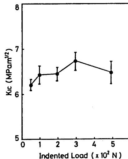
Fig.4. Indented load dependence on the fracture toughness.
