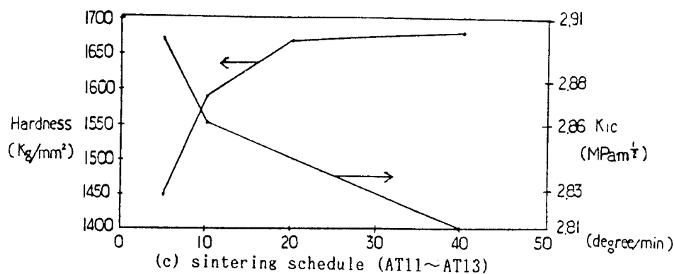
Fig. 8. Hv and K IC variations according to the sintering conditions.
