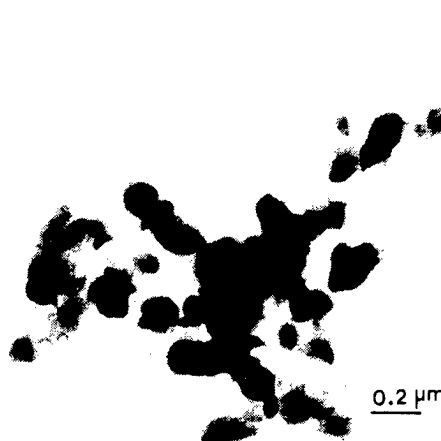
Fig.4 TEM micrograph of the \text{BaTiO}_3 powders obtained after hydrothermal-electrochemical treatment of Ti plate in 0.5N- \text{Ba}(\text{NO}_3)_2 solution at 250^\circ\text{C} .
