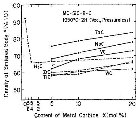
Fig. 1. Density for SiC-Metallic Carbides in 1950°C sintering.
