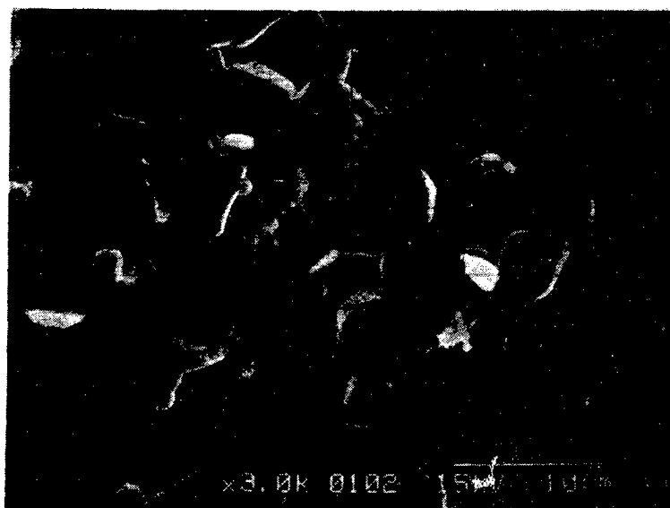
Photo.1. Fracture surface of the sample for CASE 1.
