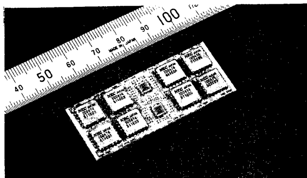
Fig.3 Multilayer AlN substrate with 3 metallized layer.
