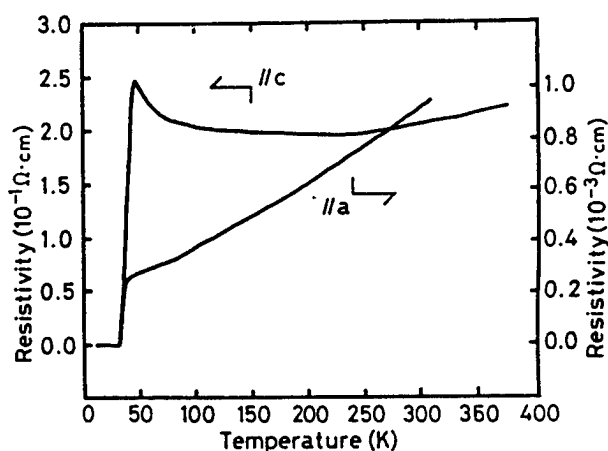
Fig.2 Electrical resistivities of \text{La}_{2-x}\text{Sr}_x\text{CuO}_4 grown crystals
