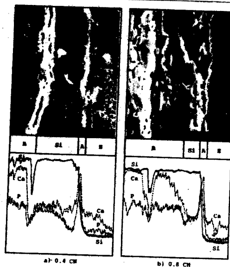
Fig.4 Line profiles of EDX and micrographs of cross sections of 0.4 CM and 0.8 CM bioglasses after 100 hours reaction in tris-buffer solution.
