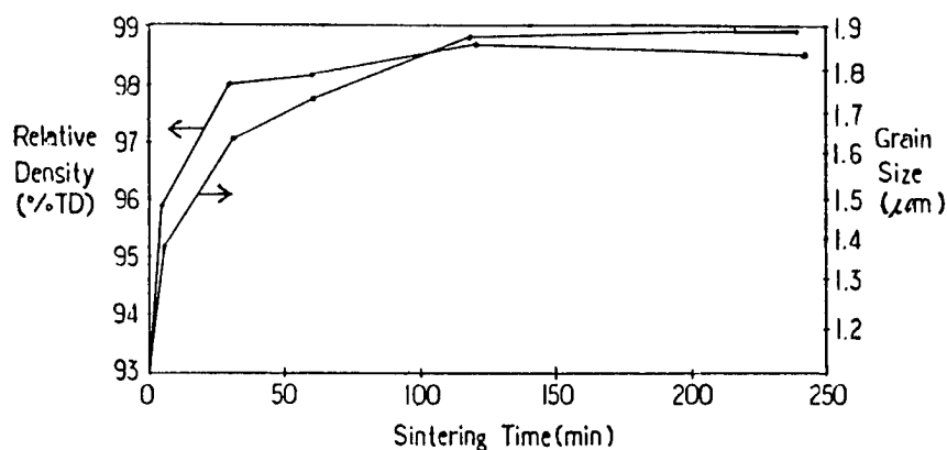
Fig. 4. Density and grain size of sintered \text{Al}_2\text{O}_3 -TiC according to the sintering time at 1850^\circ\text{C} (Table 1, AT6~AT10)
