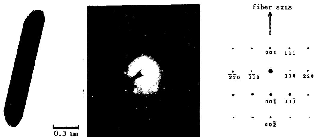
Fig. 3 Bright field image and electron diffraction pattern of needle-like mullite obtained at 1650°C.
