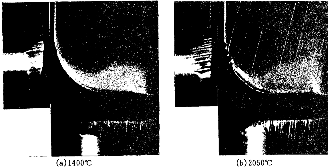
Photo.1 Wear pattern of cemented carbide insert after cutting C-20vol% (SiC+B 4 C) composite sintered at (a) 1400°C or (b) 2050°C.
