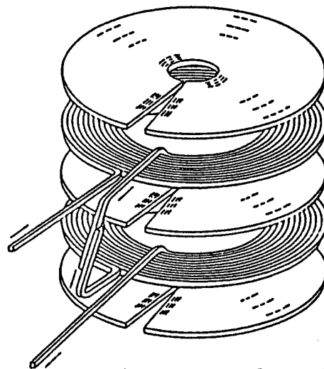
Fig.4 Laminated coil
