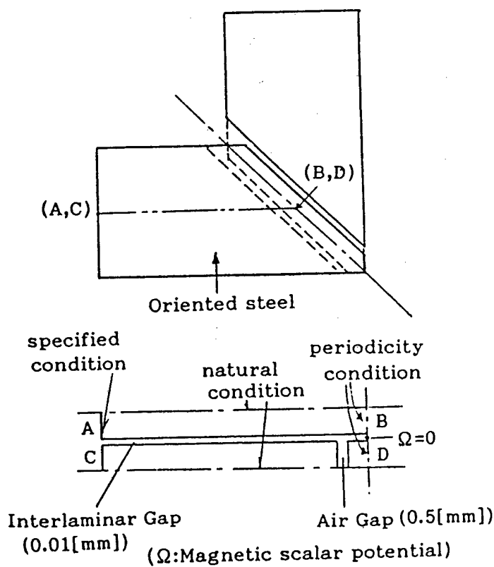
Fig. 3 Analyzed model.
