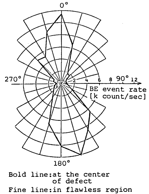
Fig.6 Event rate of Barkhausen noise. (Sensor assembly rotates at the center of the flaw, current descending process)
