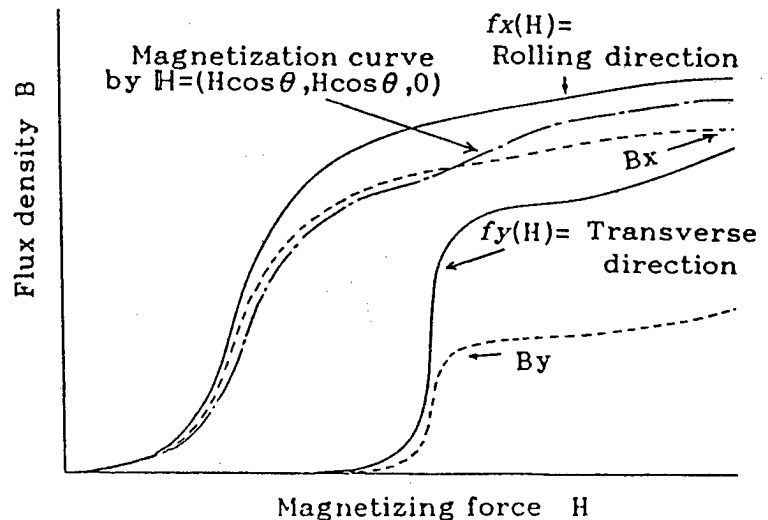
Fig. 2 The magnetization curve. (\theta=30^\circ)
