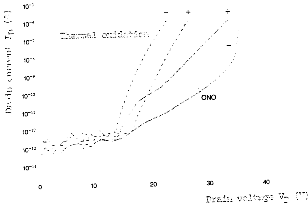
Figure 5. Low leakage current in the ONO film
