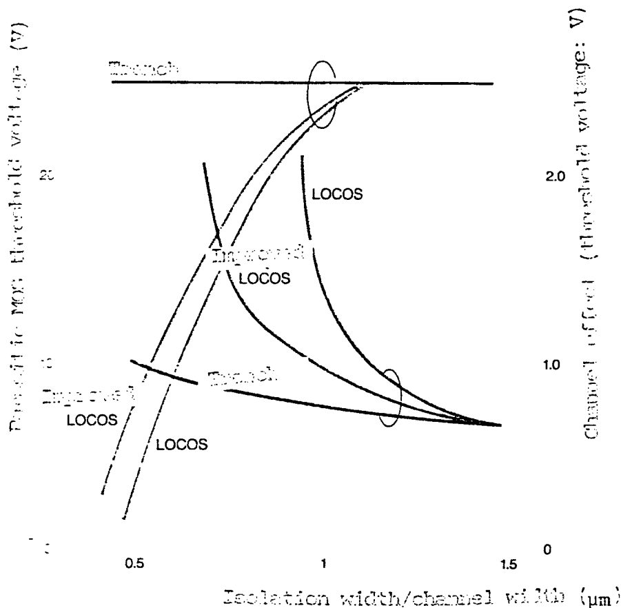
Figure 2. When trench isolation is used, the puncture resistant voltage is not degraded even at 0.6 \mu\text{m} separation
