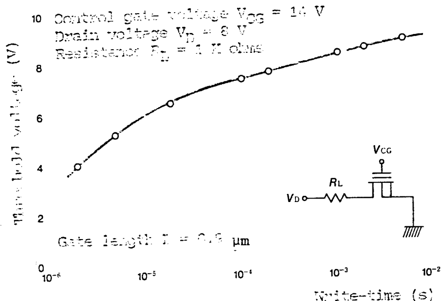
Figure 7. A 5 V shift can be carried out in 10 \mu\text{s}
