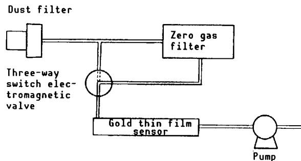
Figure 6. Block Diagram for Hydrogen Sulfide Meter Utilizing Gold Thin Film Sensor
