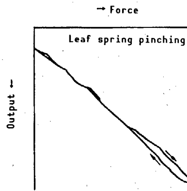
Figure 8. F-R Characteristic Within Leaf Spring
