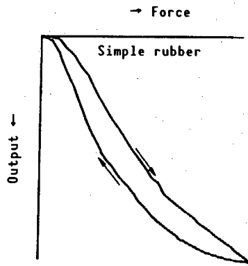
Figure 7. F-R Characteristic for Simple Rubber
