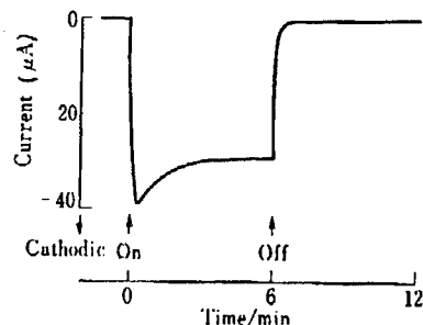
Figure 2. Photocurrent Induced by a Polythienylene Film ( 1.8 \text{ cm}^2 ) Immersion in an Electrolytic Solution ( 0.1 \text{ M LiClO}_4 ) (Electrode potential -0.2 \text{ V} vs. \text{Ag-AgCl} )
