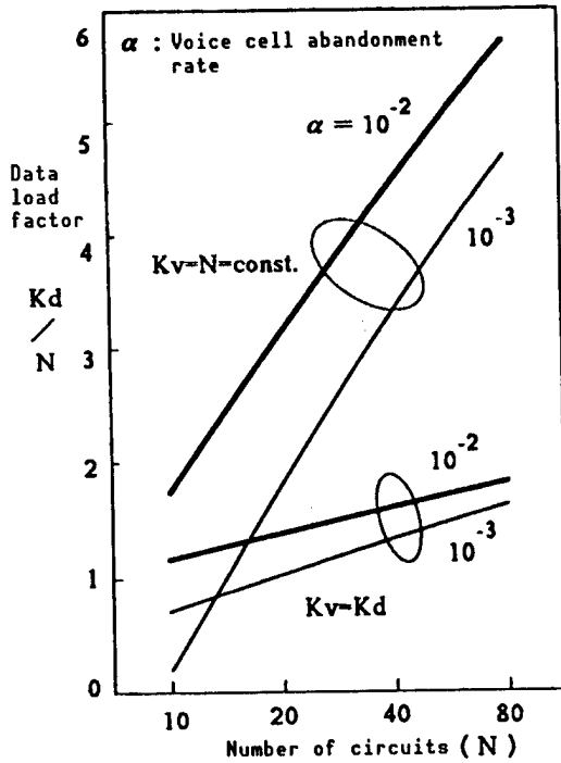
Figure 10. Data Load Factor (Case II)
