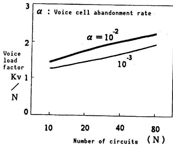
Figure 8. Relationship Between Load Factor and Number of Circuits (Case I)
