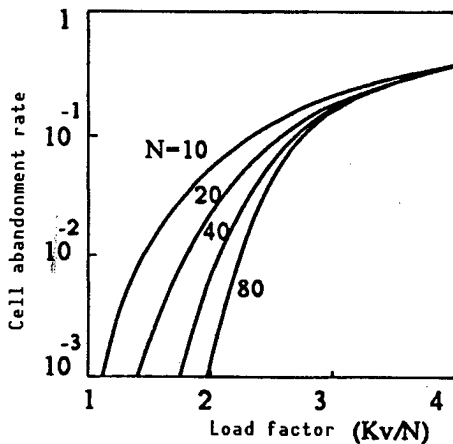
Figure 6. Circuit Usage Rate (Case I)
