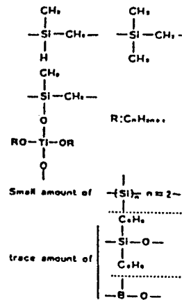
Figure 2. Unit structures of PTC
