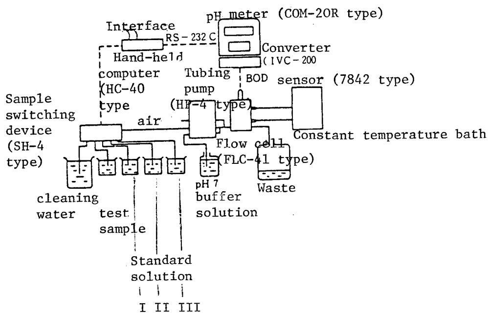
Figure 11. System Composition Diagram
