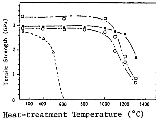
Figure 4. Heat-resistance of Carbon fiber (--- \Delta ---), SiC fiber (— \circ —), SiC/C fiber (--- \square ---) and Si-Ti-C-O fiber (— \bullet —)
