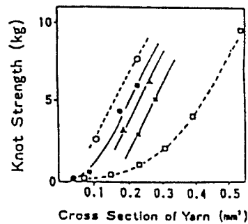
Figure 3. Knot strength of Carbon fiber (7 \mu\text{m} ; ---○---), Si-Ti-C-O fiber (8.5 \mu\text{m} ; —●—, 10 \mu\text{m} ; —▲—, 11 \mu\text{m} ; —■—) and SiC fiber (14 \mu\text{m} ; ---□---)
