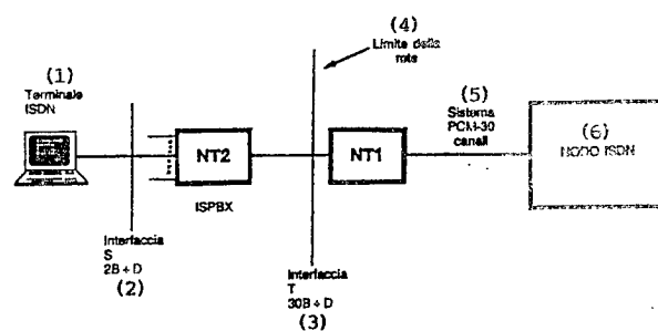
Figure 4. Line From ISPBX to ISDN Node
