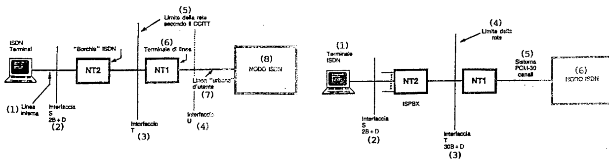
Figure 4. Line From ISPBX to ISDN Node
