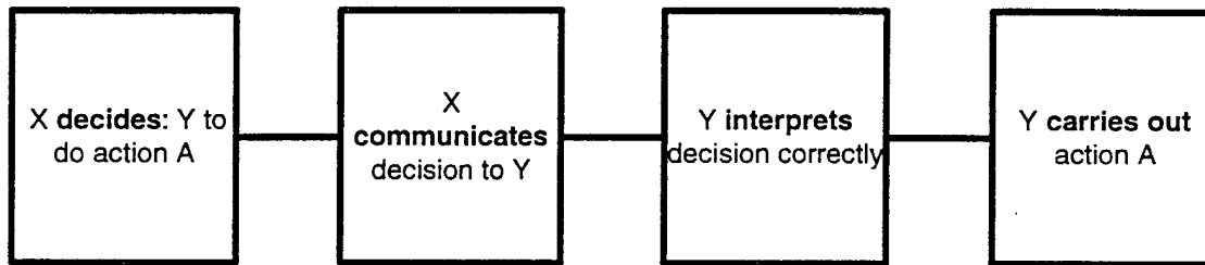
Figure 7. Command structure.
