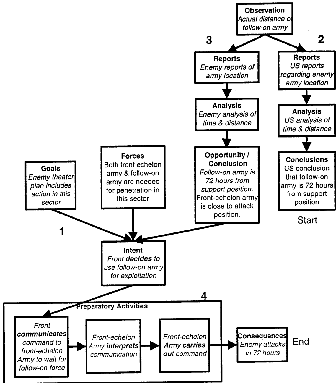
Figure 20. Combination of (1) an intent-to-attack structure, (2 & 3) two evidence-interpretation structures, and (4) a command structure. Note that the observation node is part of both evidence-interpretation structures; the intent node in the intent-to-attack structure also serves as the decide node in the command structure; and the remainder of the command structure is a set of preparatory activities within the intent-to-attack structure. The chain of argument goes from the node labeled “start” to the node labeled “end.”
