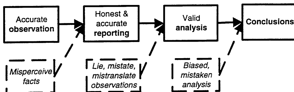
Figure 18. Evidence-interpretation structure with illustrative alternative causes. Since the argument goes from effects (the conclusion on the right) to causes (the accurate observation on the left), it can be derailed by any of these alternative causes.
