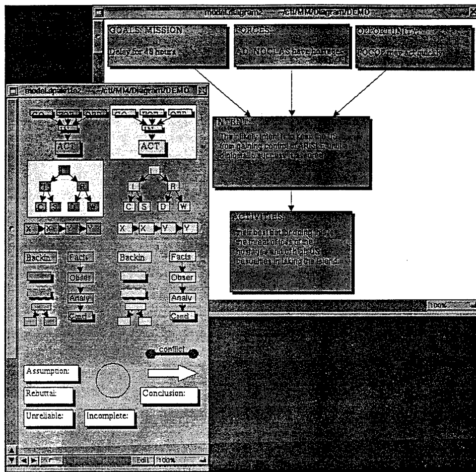
Figure 41. Candidate completions.
