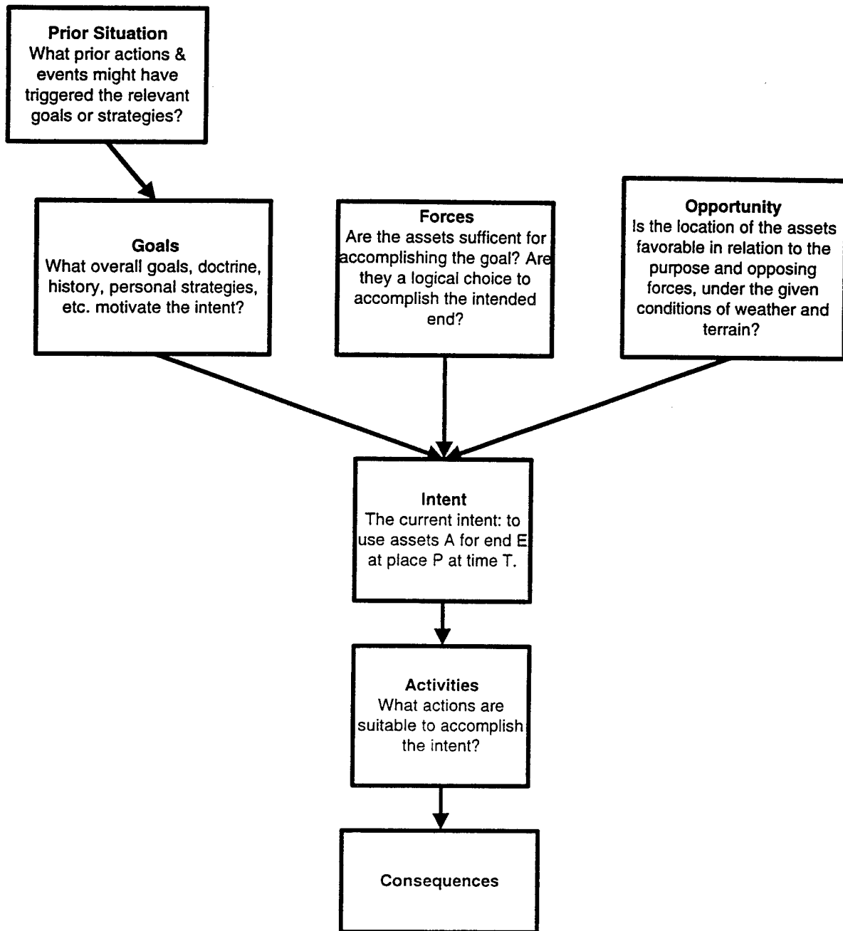
Figure 2. Intent model.
