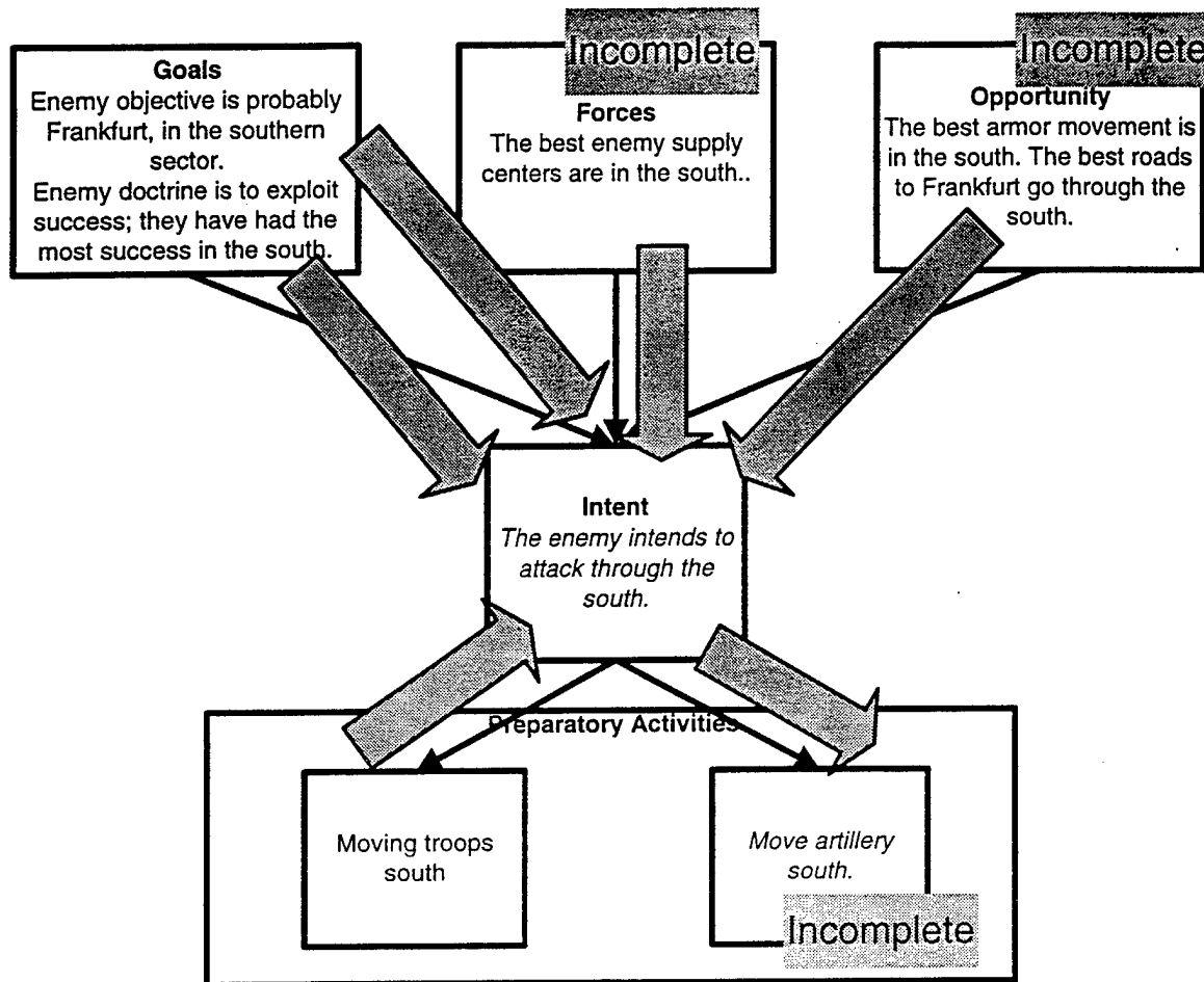
Figure 10. Large shaded arrows represent arguments in the original intent-to-attack story. Four arguments support attack in the south, and one argument yields a prediction regarding artillery movements based on attack in the south. Italicized items are inferred, i.e., they are the conclusions of arguments.
