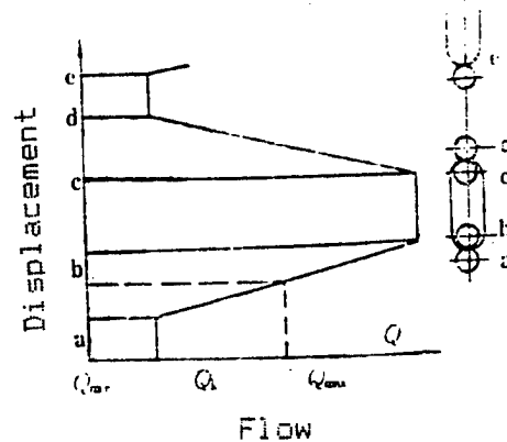
Figure 2. Static Characteristics of Hydraulic Stepping Cylinder
