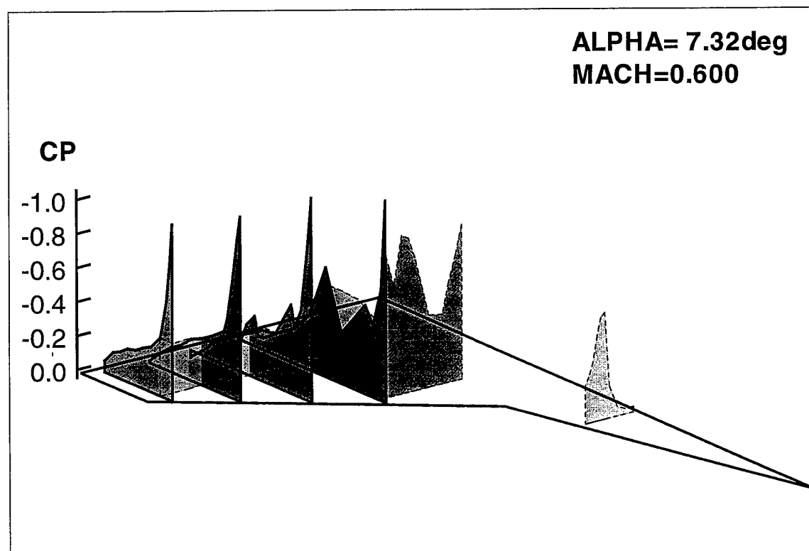
Figure 2.63 - Unsteady Pressure Distributions During Pitching Motion from 7.2 deg to 37.7 deg to 7.1 deg at Phase Angles of 348.75 deg and 354.38 deg
