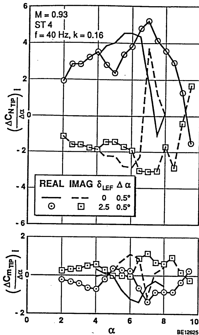
Figure 8 - Integrated Unsteady Pressures at Section 4 Showing the Effect of Leading Edge Flap Deflection at M = 0.93 for the Wing/Body With Tip Launcher Configuration (Reference 8)
