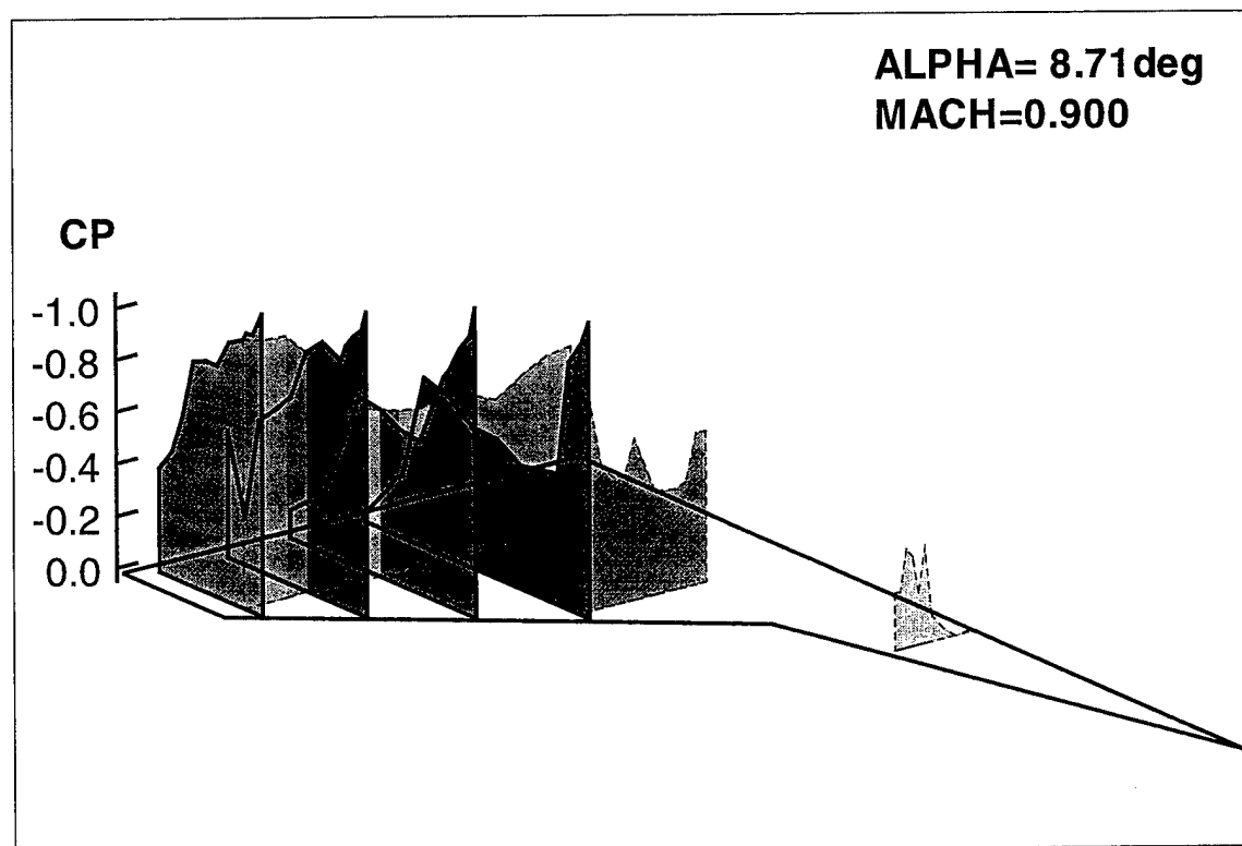
Figure 4.59 - Unsteady Pressure Distributions During Pitching Motion from 7.2 deg to 37.7 deg to 7.1 deg at Phase Angles of 326.25 deg and 331.88 deg
