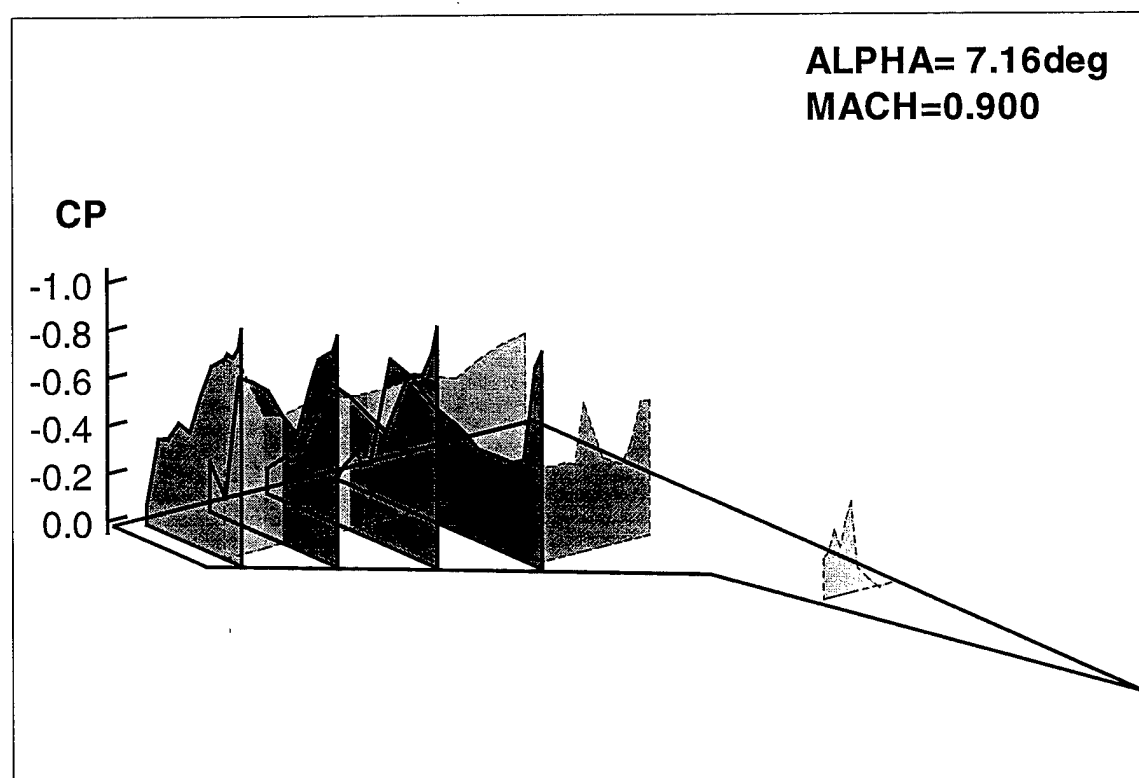
Figure 4.63 - Unsteady Pressure Distributions During Pitching Motion from 7.2 deg to 37.7 deg to 7.1 deg at Phase Angles of 348.75 deg and 354.38 deg
