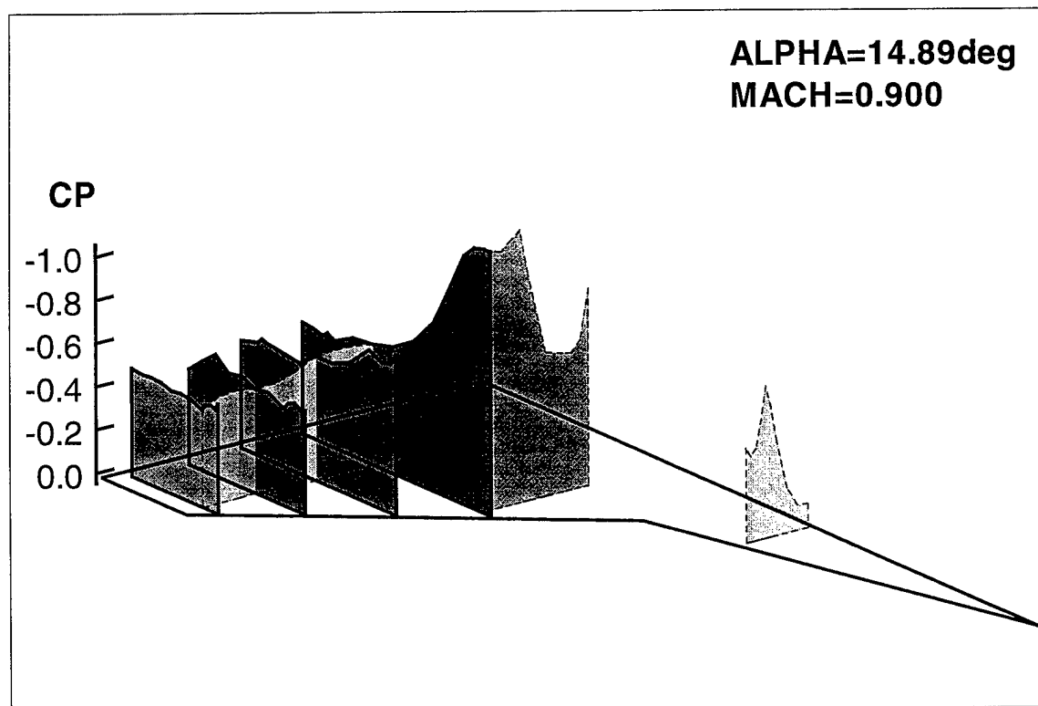
Figure 4.53 - Unsteady Pressure Distributions During Pitching Motion from 7.2 deg to 37.7 deg to 7.1 deg at Phase Angles of 292.50 deg and 298.12 deg
