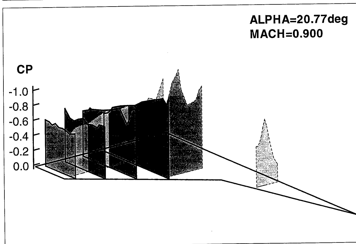
Figure 4.49 - Unsteady Pressure Distributions During Pitching Motion from 7.2 deg to 37.7 deg to 7.1 deg at Phase Angles of 270.00 deg and 275.62 deg
