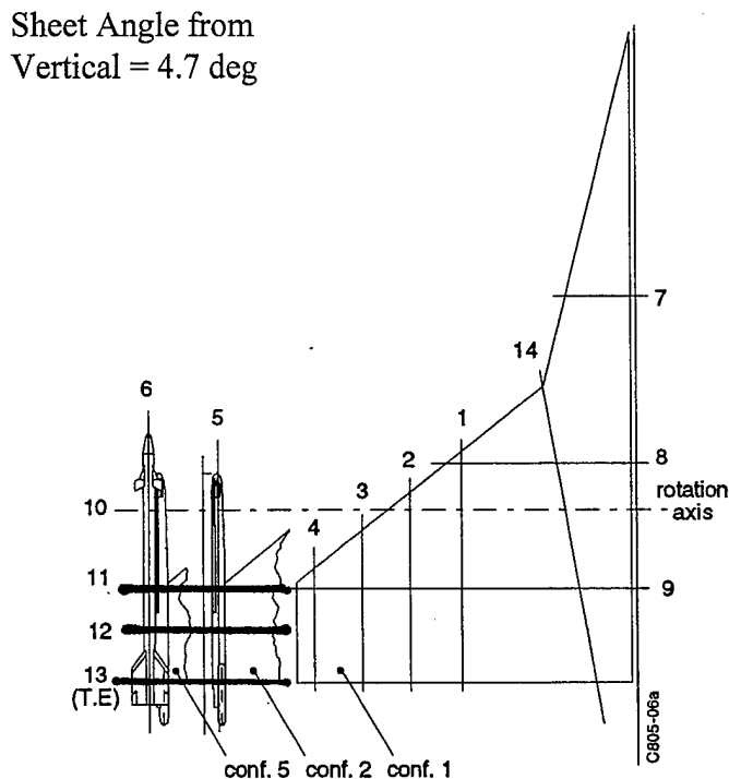
Figure 10 - Flow Visualization Locations for Figures 11, LCO Conditions, Wing With Tip Launcher, M = 0.85 , Oscillating at \pm 0.5 deg
