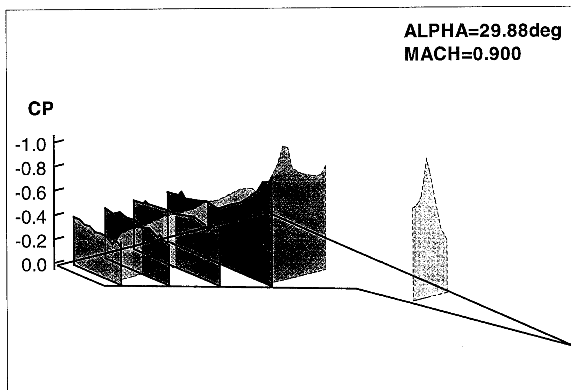
Figure 4.43 - Unsteady Pressure Distributions During Pitching Motion from 7.2 deg to 37.7 deg to 7.1 deg at Phase Angles of 236.25 deg and 241.88 deg
