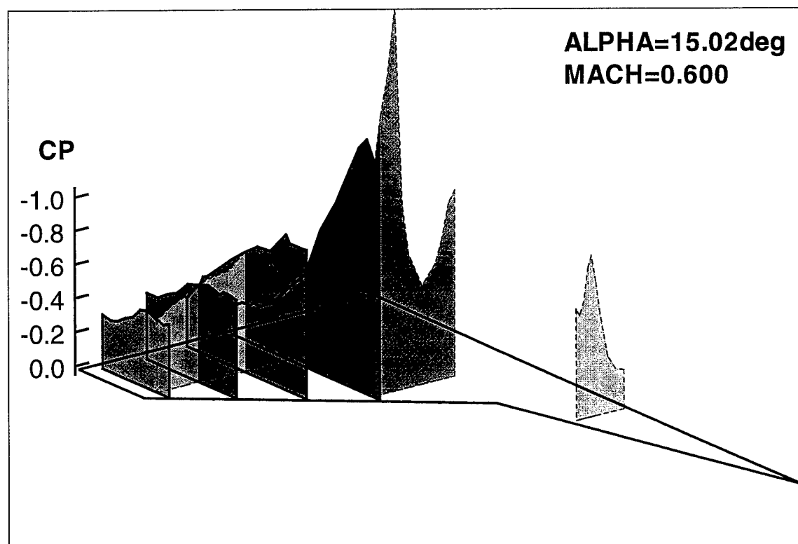
Figure 2.53 - Unsteady Pressure Distributions During Pitching Motion from 7.2 deg to 37.7 deg to 7.1 deg at Phase Angles of 292.50 deg and 298.12 deg
