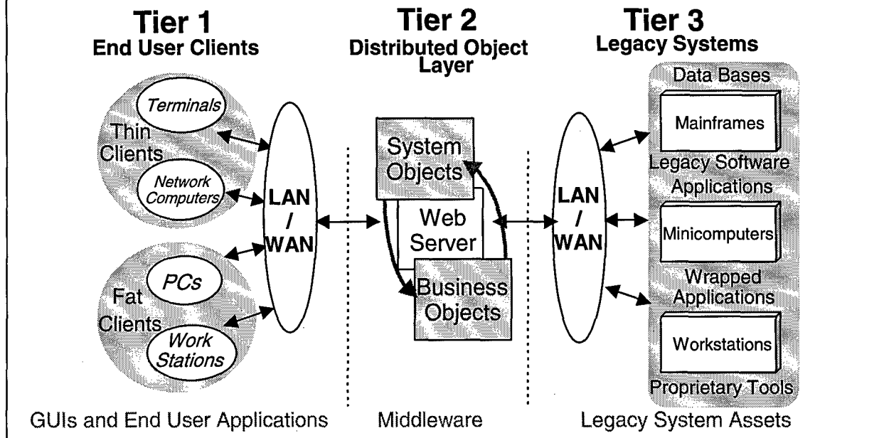
Figure 3: The Distributed Object Computing Paradigm
