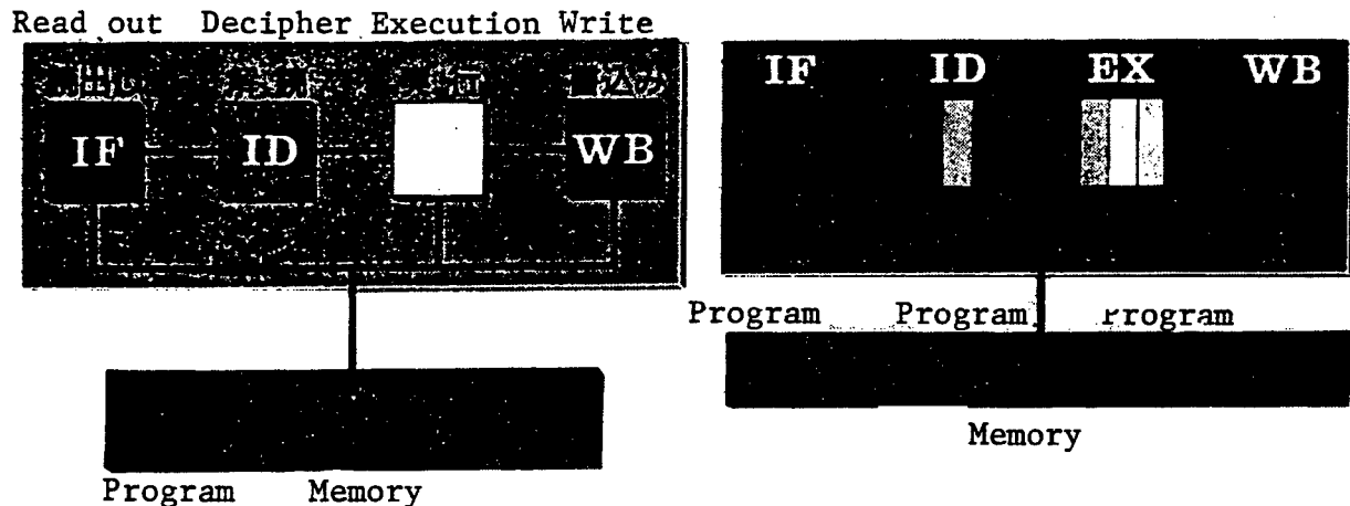
Figure 14. Comparison of a Conventional Pipeline System (left) and Cyclic Pipeline System (right)
