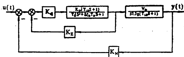
Figure 1. Simplified Block Diagram of Ground-to-Air Missile Autopilot Pitch Channel
