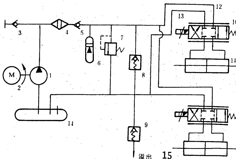
Figure 2. Diagram of Hydraulic Principles of Two-Way Swivelling Servomechanism
