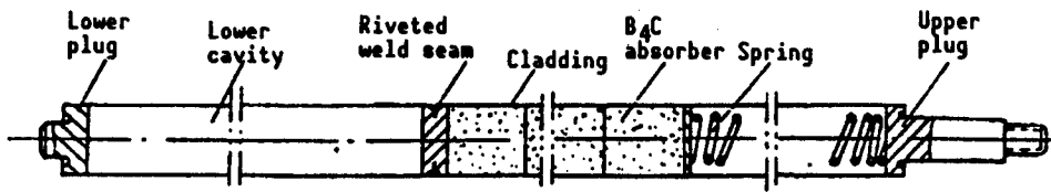
Figure 8. Schematic Diagram of the Pulsing Rod
