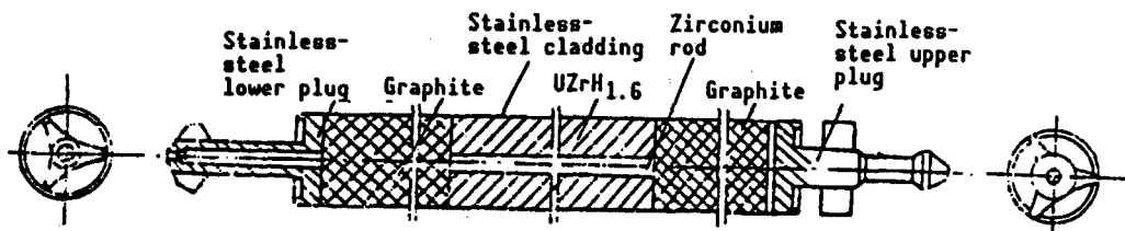
Figure 5. Schematic Diagram of the Pulsed Reactor Fuel Element
