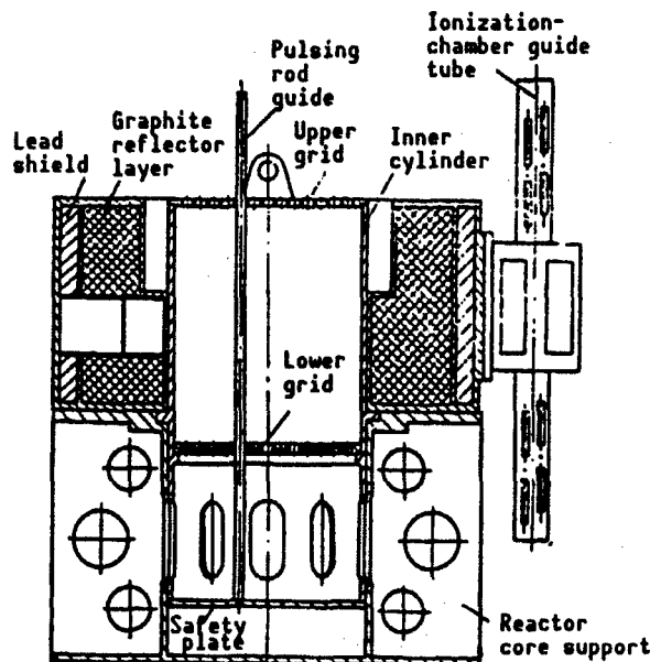
Figure 4. Reactor Internals
