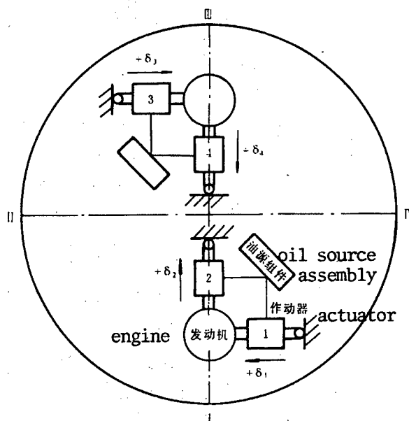
Figure 3. Configuration of Two-Way Swivelling Servomechanism and Engine
