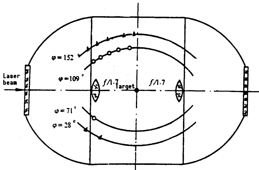
Figure 4. Layout of Harmonic Wave Probes ("Δ" is 3/2\omega_0 probe and "O" is 2\omega_0 probe)
