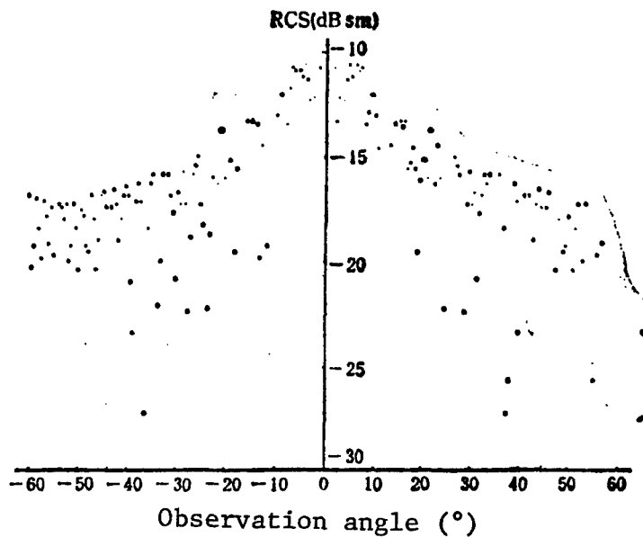
Figure 6. RCS of Model Shown in Figure 3 Under Horizontal Polarization
