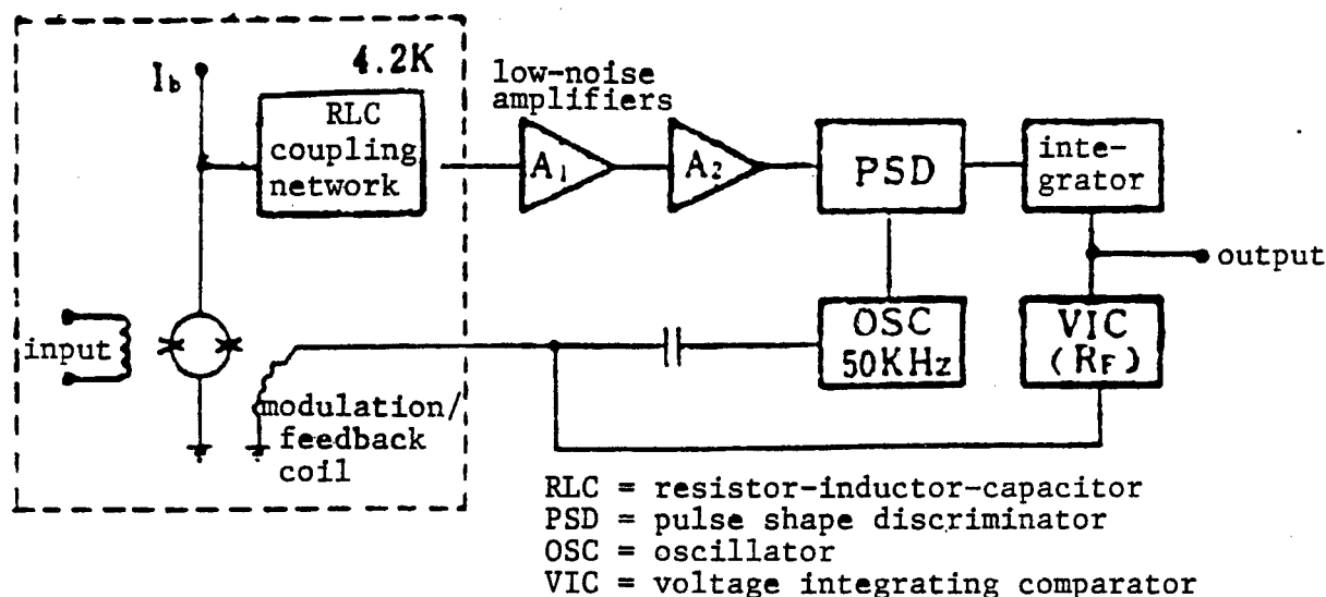
Figure 1. Schematic Diagram of DC SQUID Magnetometer
