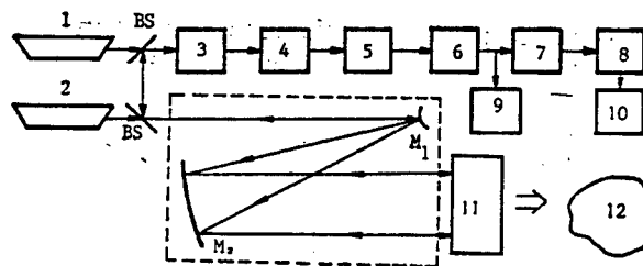
Figure 2. Schematic Diagram of the Experimental Arrangement
