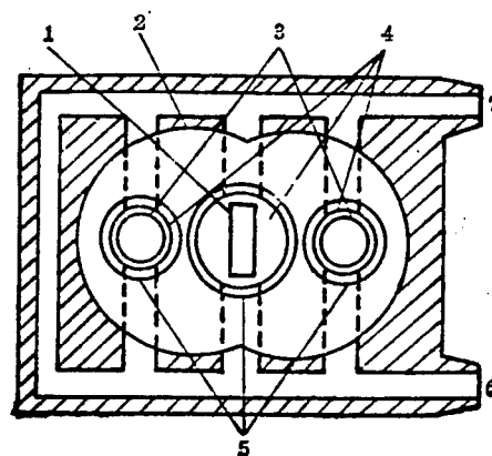
Figure 1. Cross Section of the Slab Laser
