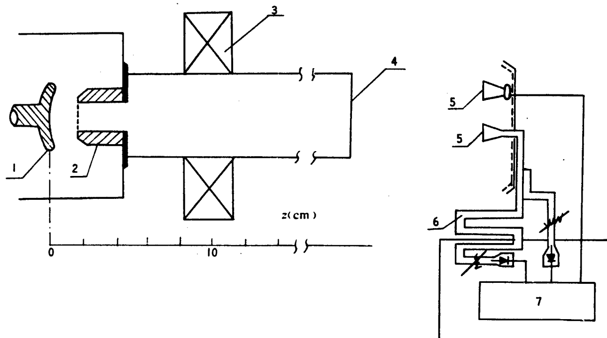
Figure 1. Experimental Apparatus for the Virtual Cathode Radiation Device
