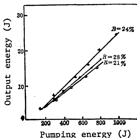
Figure 4. Free-Oscillation Pulse Output
