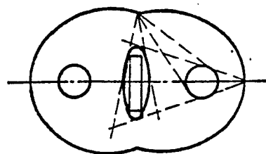
Figure 2. Slab in the Elliptical Focusing Cavity
