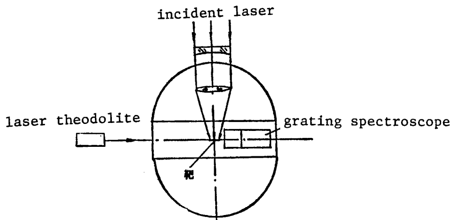
Figure 2. Experimental Apparatus
