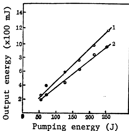
Figure 5. Q-Switched Pulse Output
