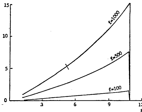
Figure 2. Dependence of the Beam Expansion \eta on the Magnification of Hyperboloid g . Focal length of the paraboloid f is a variable parameter.
