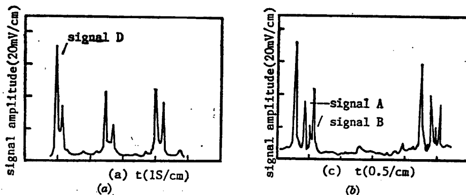
Figure 4. Electrical Signals Recorded by X-Y Recorder
