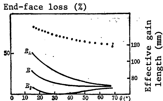
Figure 3. End-Face Loss vs. Effective Gain Length
