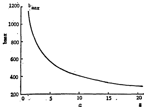
Figure 3. Maximum of Hyperboloid a_1 Short Axis b_{max} Versus g
