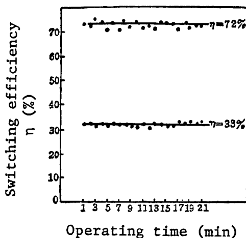
Figure 6. Stability of Q-Switching
