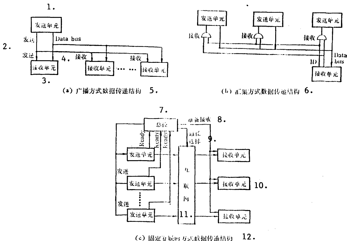
Figure 4. Data Transmission Structures
