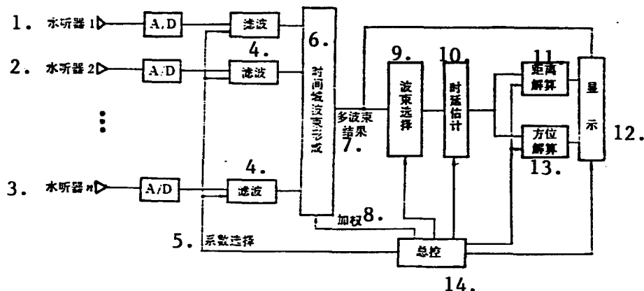
Figure 1. Passive Orientation/Range Sonar
