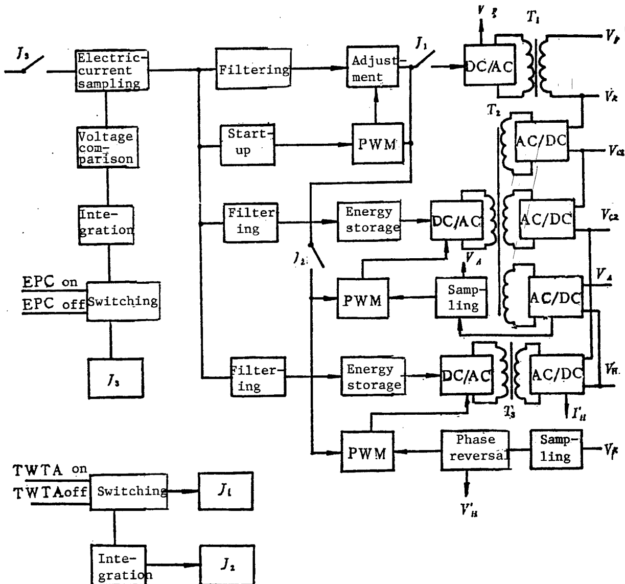
Figure 1. Block Diagram of the Traveling-Wave-Tube Power Supply
