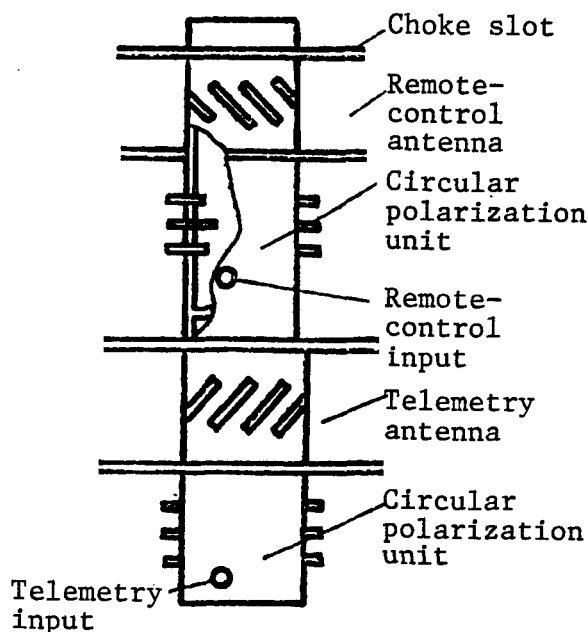
Figure 5. Schematic Diagram of the Telemetry, Command and Control Antenna
