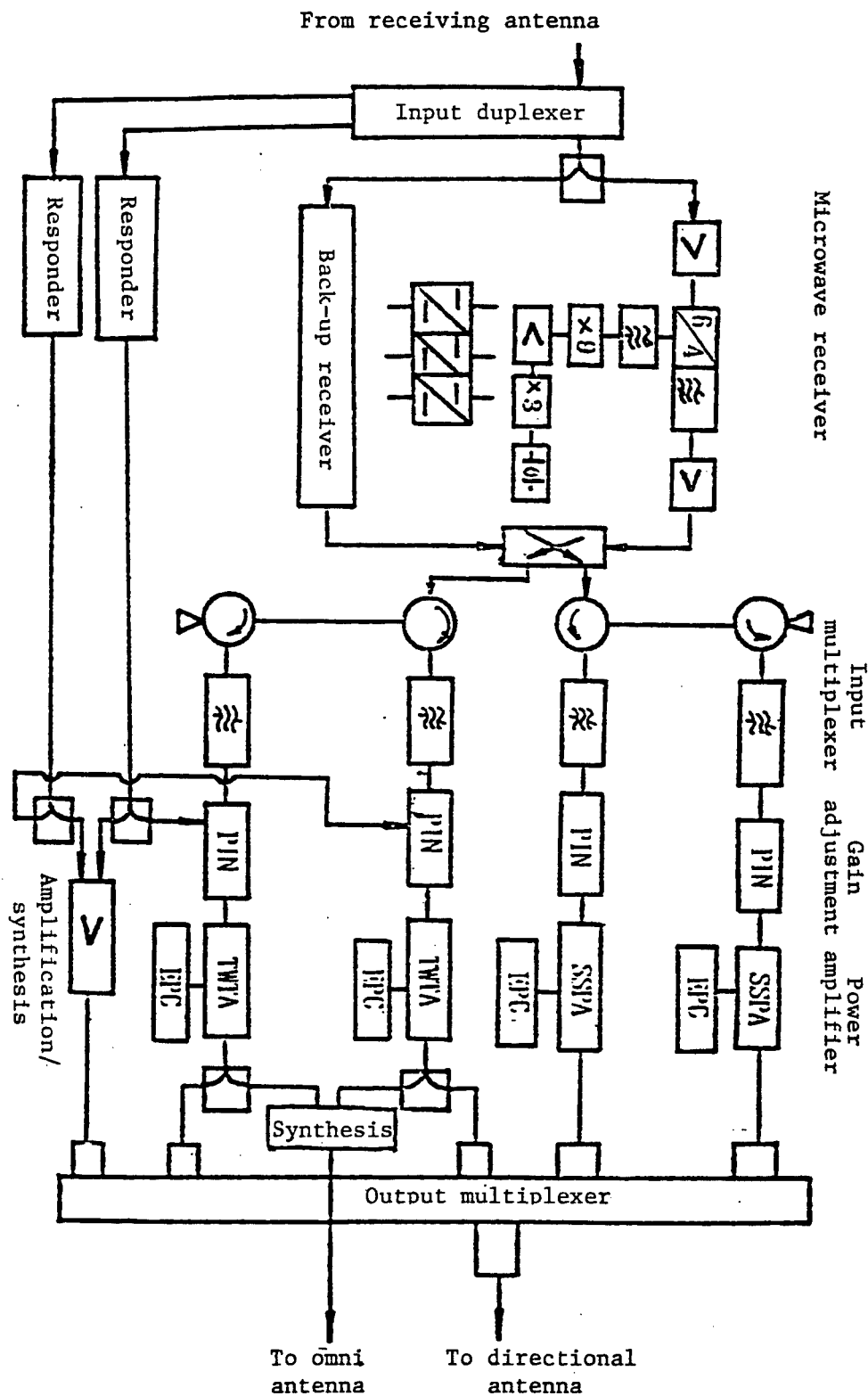
Figure 1. Block Diagram of the Transponder Used by the DFH-2A No. 1 Satellite (Also Shows the Relationship with the TT&C Channel)
