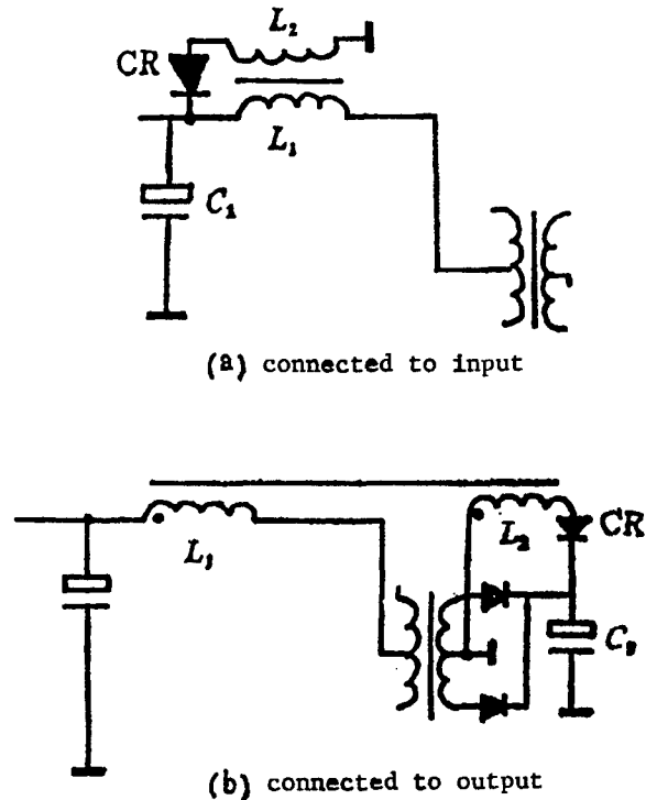
Figure 3. Two Methods of Connecting the Feedback Coil of the Energy-Storage Inductor
