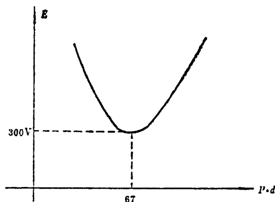
Figure 6. Parson's Curve
