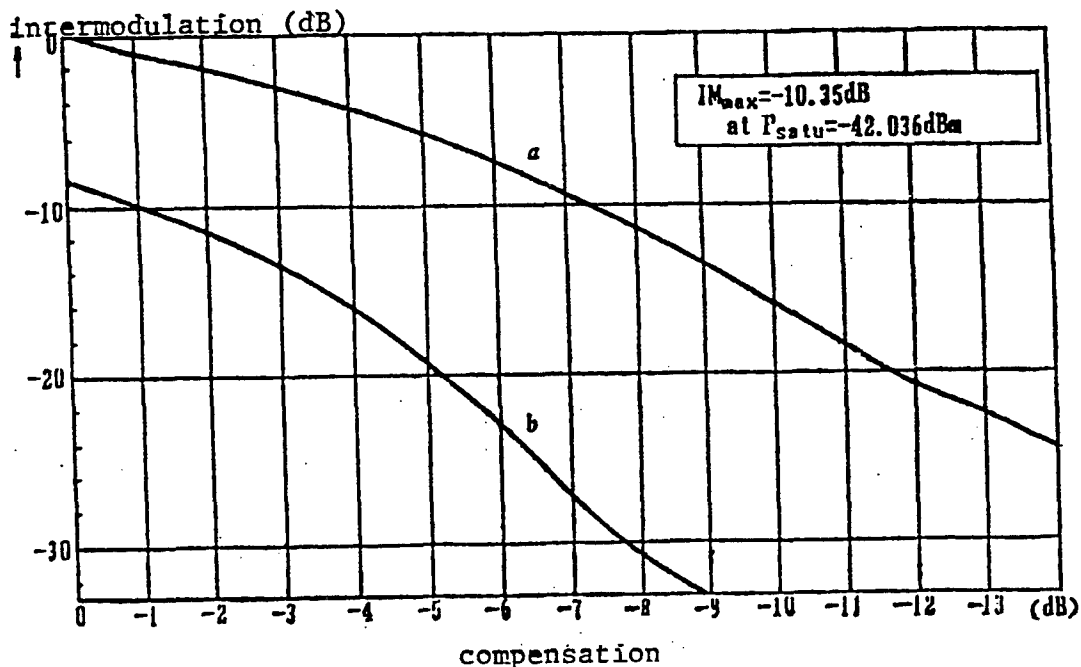
Figure 4. Typical Inter-Modulation Characteristics of the Transponder. a. IM 3; b. IM 5
