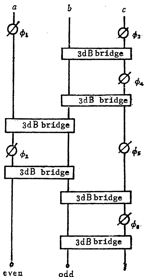
Figure 4. Block Diagram of the 2-3 Odd-Even Synthesizer
