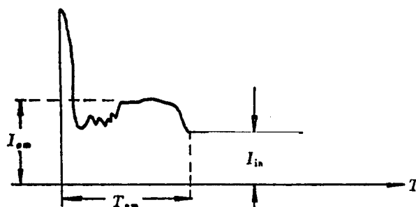
Figure 7. Waveform of the Surge Current of the TWTA
