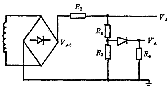
Figure 9. Anode Circuit
