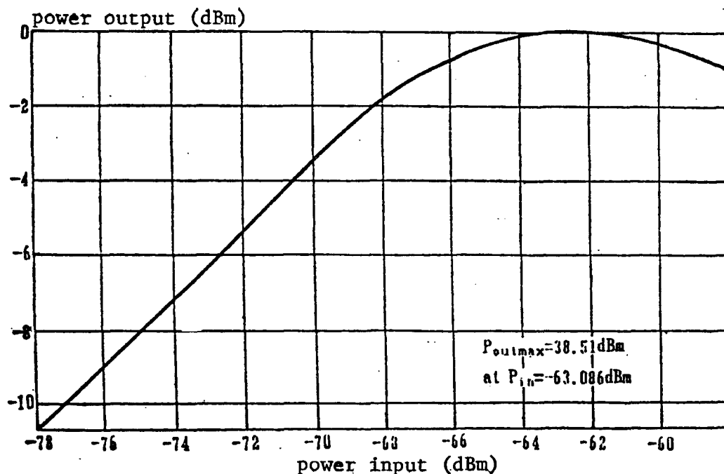
Figure 3. Typical Input-Output Characteristics of the Transponder
