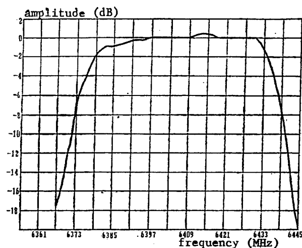
Figure 6. Amplitude-Frequency Characteristics of the Transponder (On-Orbit Test)
