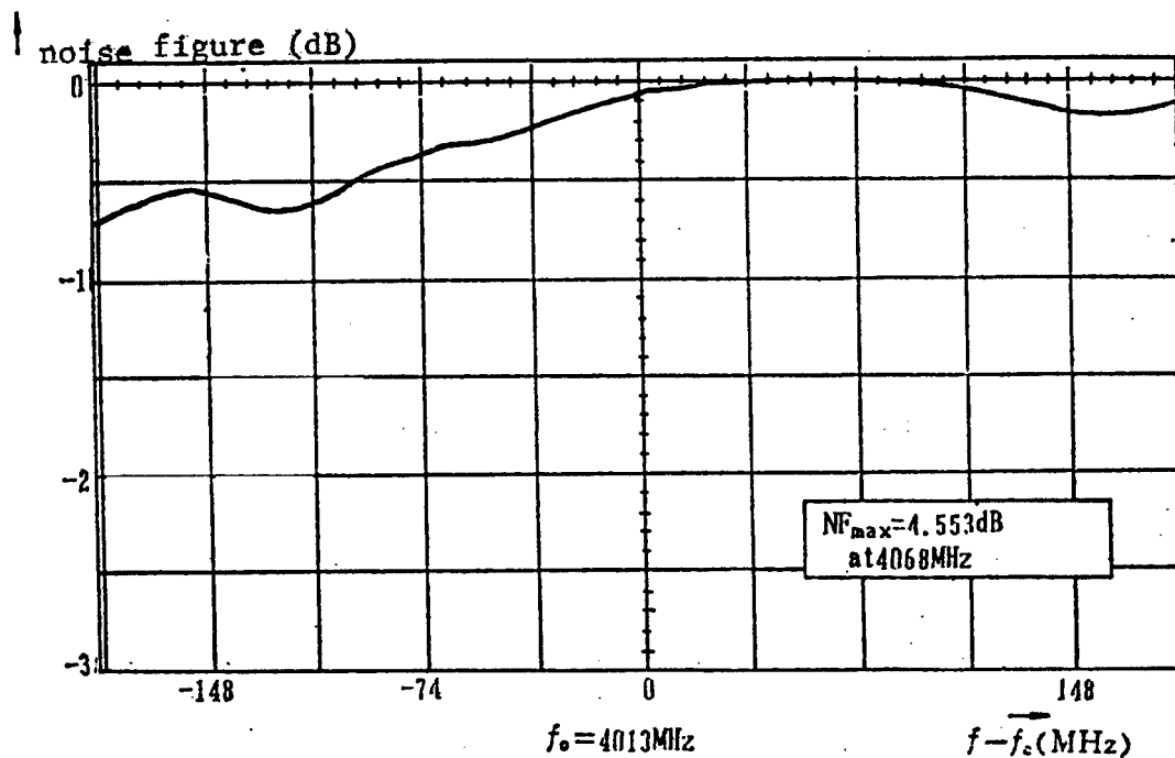
Figure 2. Transponder System Noise Figure
