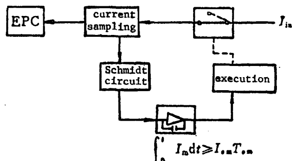
Figure 8. Integral Time-Delay Overcurrent Protection Circuit
