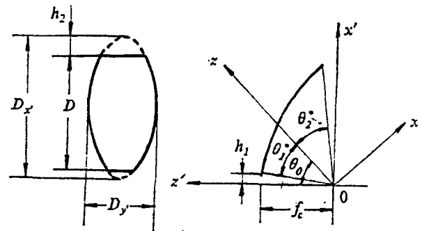
Figure 3. Schematic Diagram of the Truncated Elliptical Paraboloid
