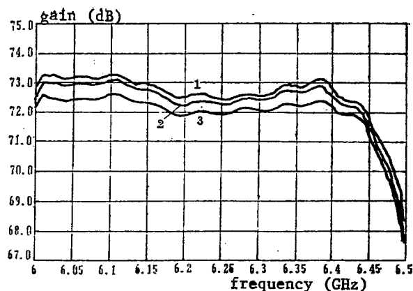
Figure 7. Typical Gain Characteristics of Microwave Receiver; Signal power: 1, -66 dBm; 2, -60 dBm; 3, -54 dBm
