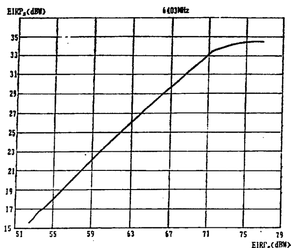
Figure 5. Input-Output Characteristics of the Transponder (On-Orbit Test)
