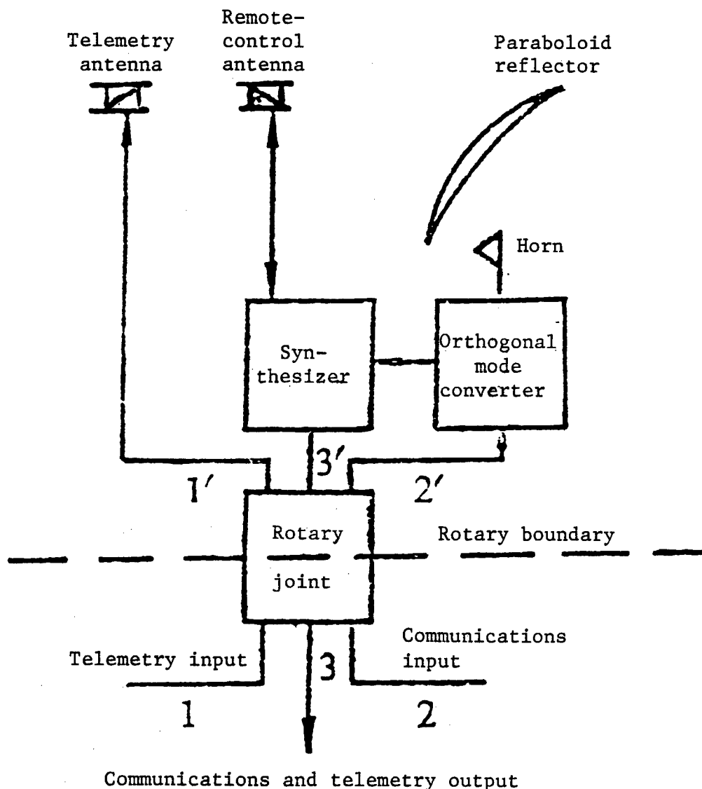
Figure 1. Electrical Block Diagram of the Antenna System
