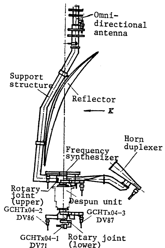
Figure 4. Configuration of the Antenna System
