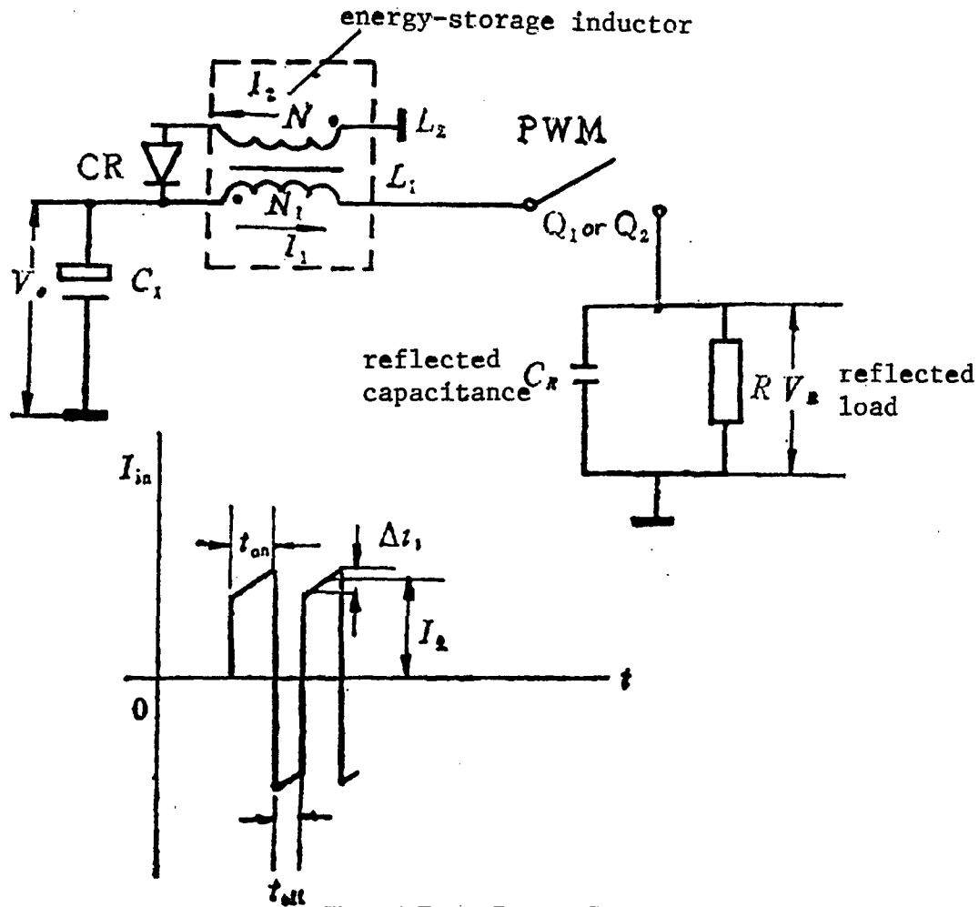
Figure 4. Energy-Recovery System
