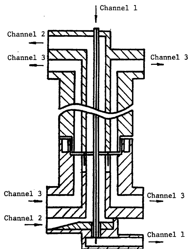
Figure 7. Schematic Diagram of the Three-Channel Rotary Joint
