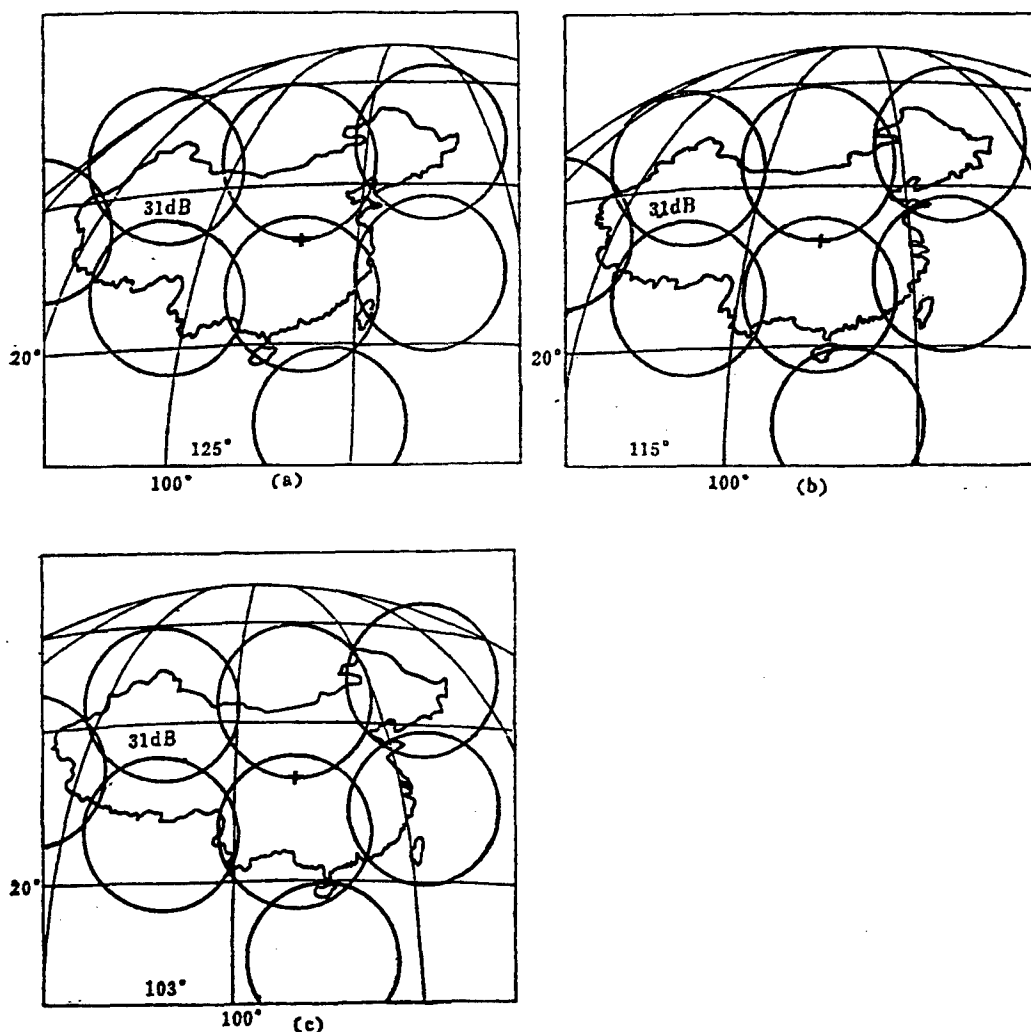
Figure 2. Beamlet Array Diagrams at Three Orbital Positions: 125°, 115°, 103°
