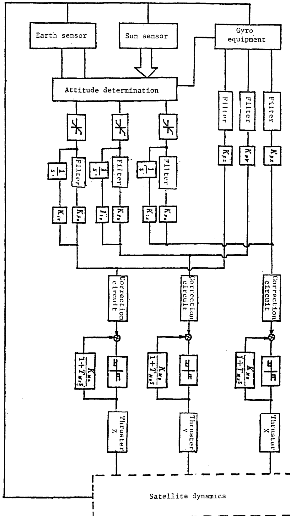
Figure 6. Stability Circuit for Apogee Orbit Change and Station Keeping
