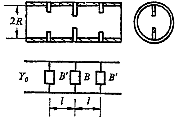
Figure 6. Three-Pin Circular Polarization Unit and Its Equivalent Circuit
