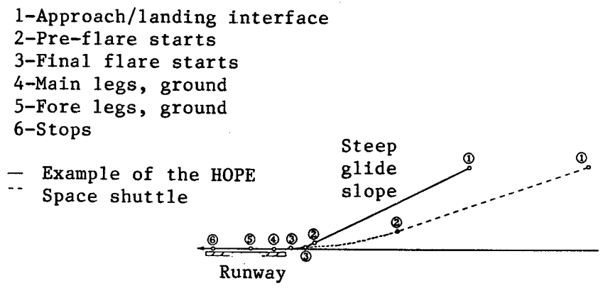
Figure 6. Example of Approach/Landing Phase of Flight Route
