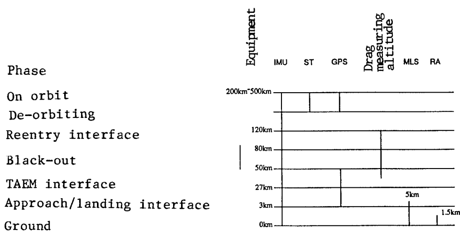
Figure 3. Navigational System Base Line Structure
