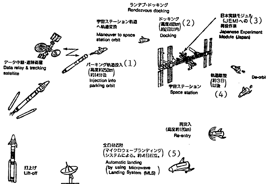
Figure 1. Flight Sequence of HOPE
