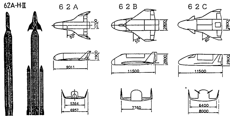
Figure 1. Airframes of Orbiters 62A, 62B, and 62C and the H-II Rocket/Orbiter 62A Combination
