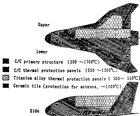
Figure 4. Setup Configuration of Thermal Protection Panels (Example)
