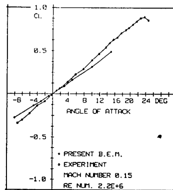
Figure 7. 62C Panel Method: Cl \sim \alpha
