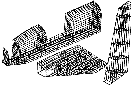
Figure 6. Finite Element Model for Structural Analysis
