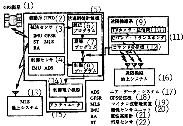
Figure 2. HOPE Guidance Control System Configuration (Suggested)
