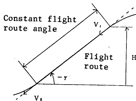
Figure 6. Trajectory of Constant Route Angle Flight
