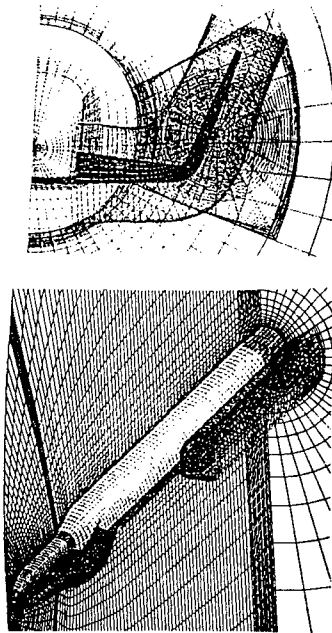
Figure 9. 62A-H-II Rocket: Superimposed Grids
