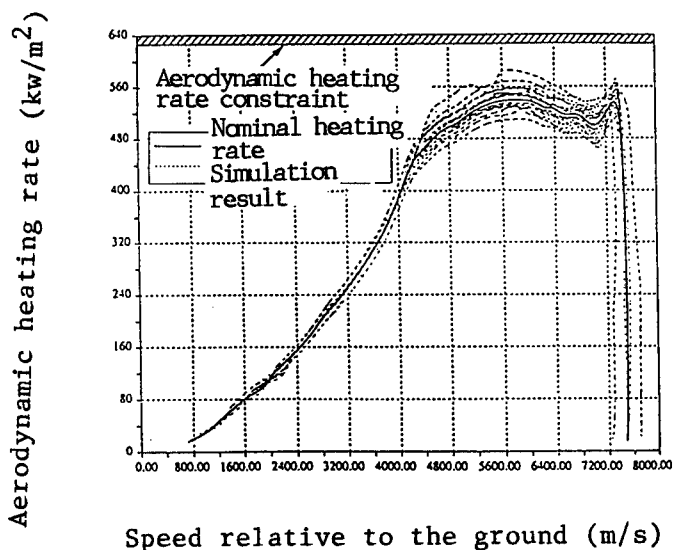
Figure 5. Example of Reentry Simulation (Aerodynamic Heating Rate)
