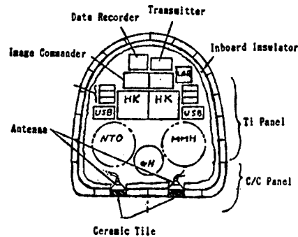
Figure 2. Heat-Resistant Structure of Forward Fuselage
