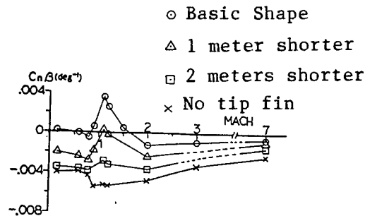
Figure 2. Effectiveness of Tip Fin Size (Schedule Elevation Angle)
