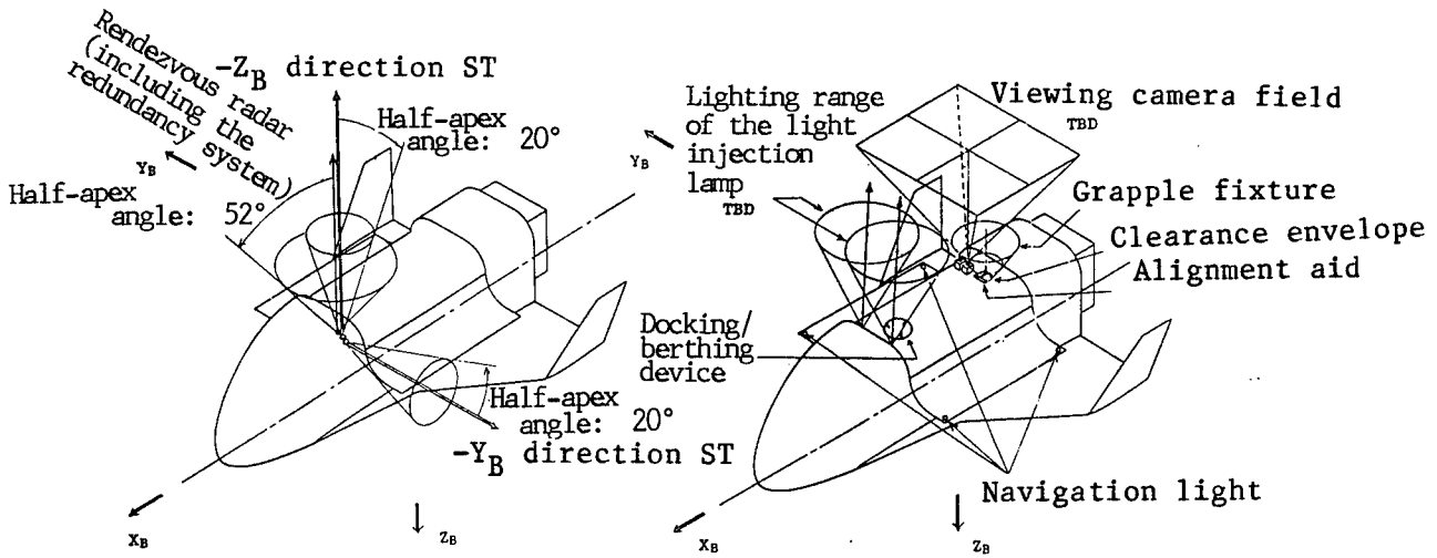
Figure 2. Installation Position of RVD-Mounted Equipment and Visual Field Characteristics
