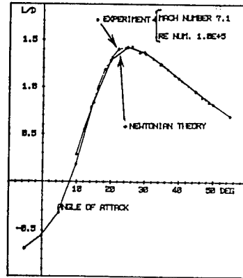
Figure 4. 62B Newtonian Calculation: L/D \sim \alpha
