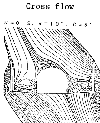
Figure 5. 62B Transonic N - S: Cross Flow
