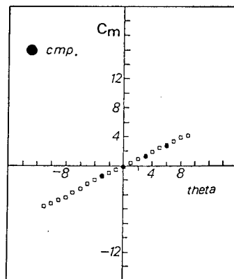
Figure 10. 62A/H-II Euler: C_m \sim \alpha
