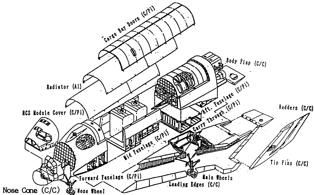
Figure 5. Substructures and Constituent Materials
