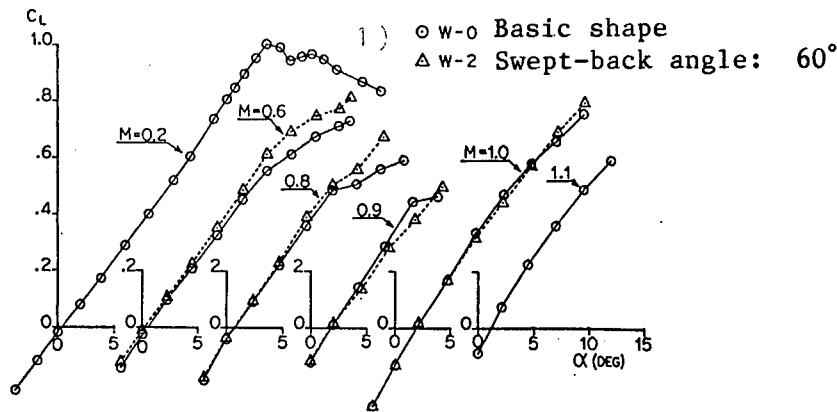
Figure 3. Transonic Lift Characteristics
