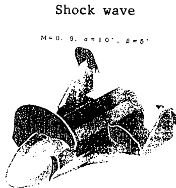
Figure 6. 62B Transonic N - S: Shock Wave
