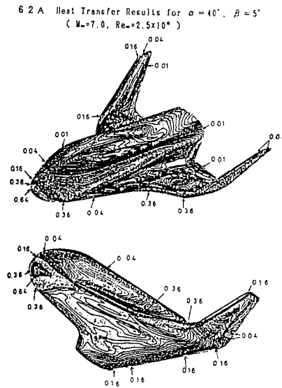
Figure 3. Aerodynamic Heating N - S: Dimensionless
