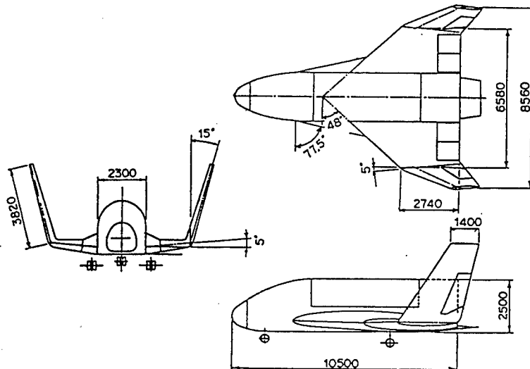
Figure 1. Suggested Aerodynamic Appearance of the HOPE
