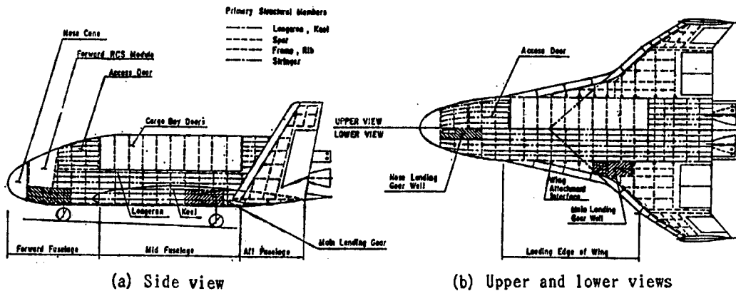
Figure 3. Frame Structure
