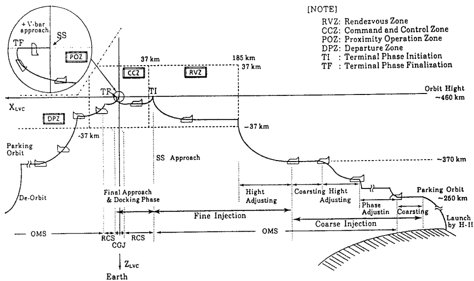
Figure 1. HOPE SS-RVD Mission Profile
