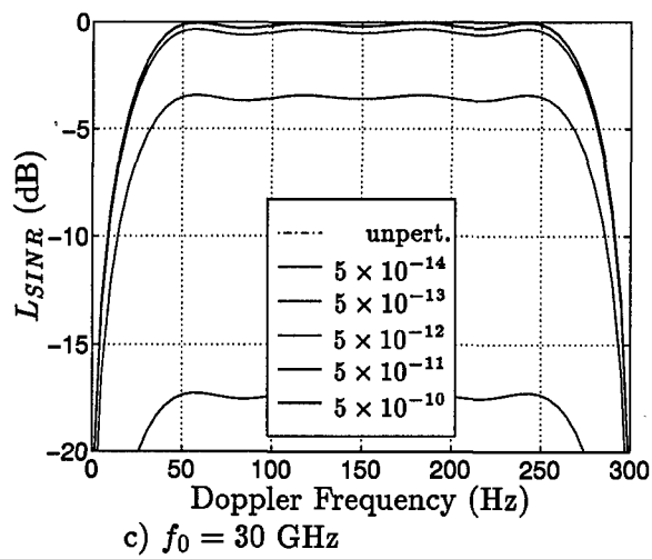
Figure 5.15 L_{SINR} for JDO under case II turbulence. Processing performed on 64 antenna elements and 5 pulses.
