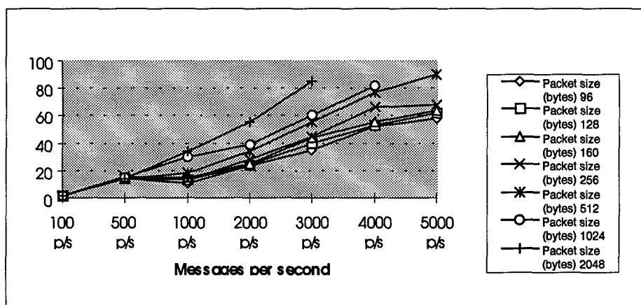
Figure 4-3: CPU utilization, Indigo2 ATM
