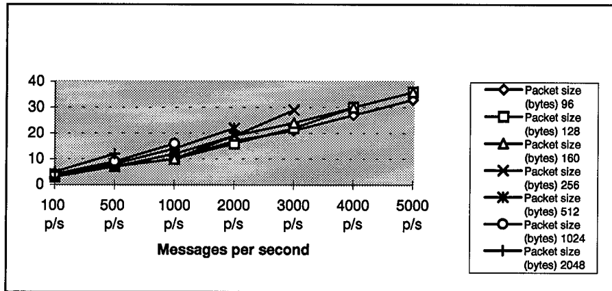
Figure 4-14: CPU utilization, Onyx2 Ethernet
