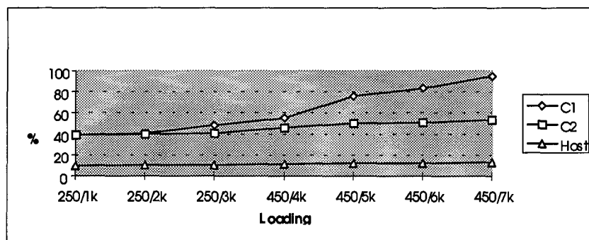
Figure 4-23: 100/100Mbps CPU use
