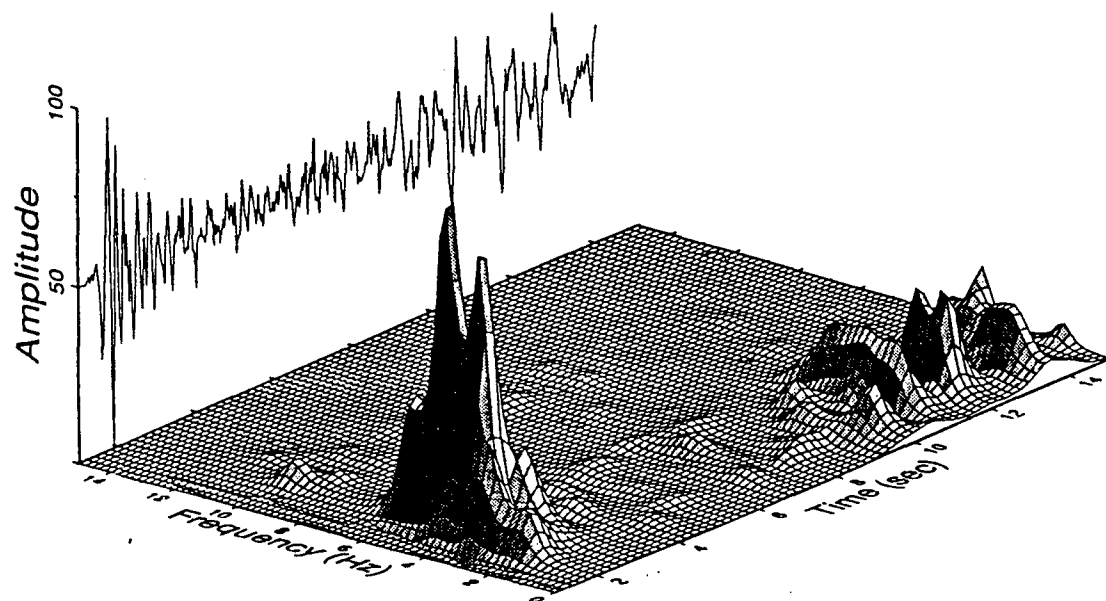
Figure 9. Spectrograms for four events that locate at the Disputada mine recorded at stations FCH and PCH. (a) event 01/04/94, (b) event 09/25/94, (c) event 09/26/94, (d) event 10/13/94.
