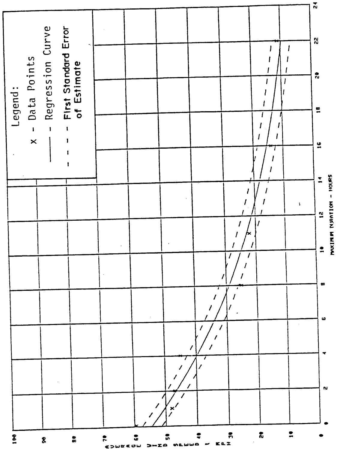
WIND PERSISTENCE MEASURED AT BOSTON, MA HYD. & W.Q. SECT. JUNE 1981
