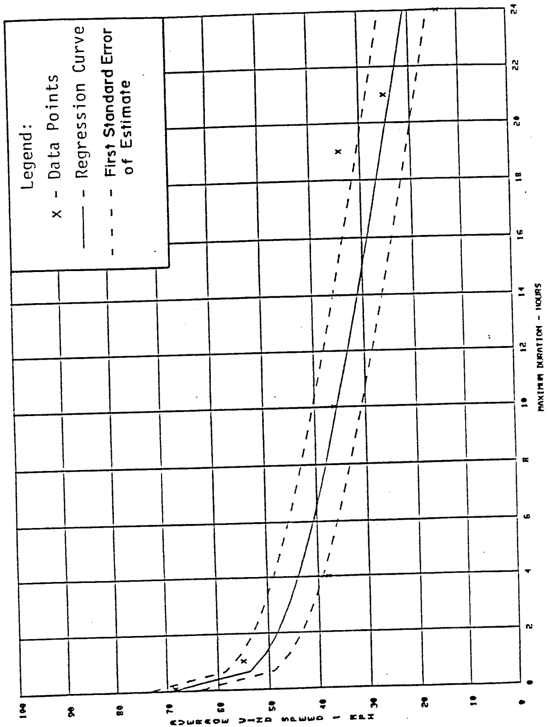
WIND PERSISTENCE MEASURED AT BOSTON, MA. HYD. & W.Q. SECT. JUNE 1988
