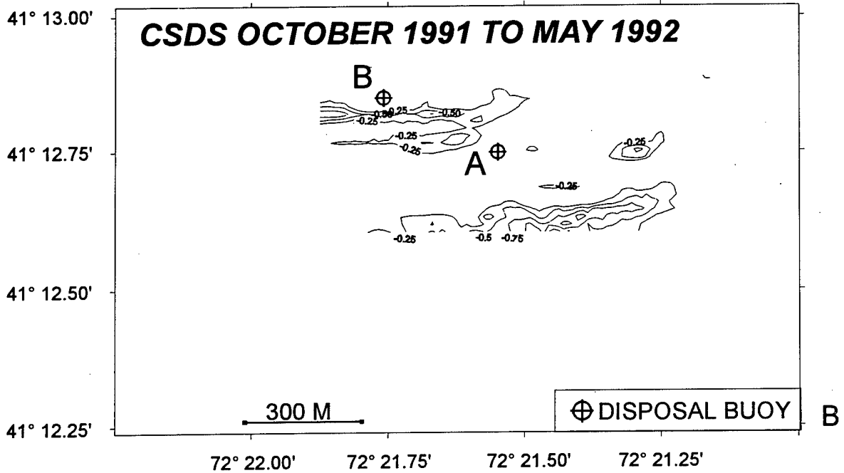
Figure 3-9. Accumulation (A) and erosion (B) at CSDS, October 18 and 19, 1991 to May 12, 1992 (depth in meters)
