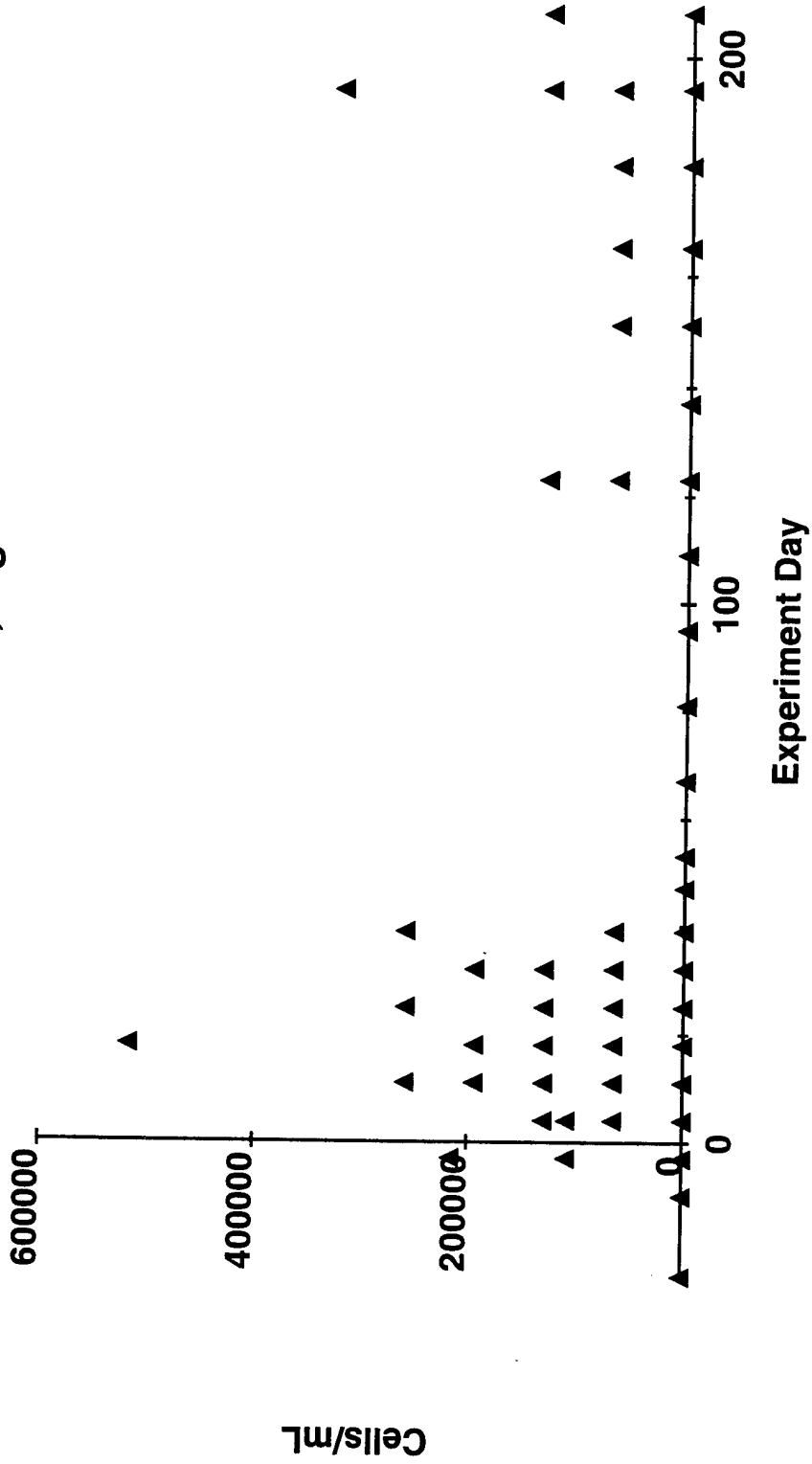
Figure 21a. Periphyton - Green Algae Selenastrum, High Dose
