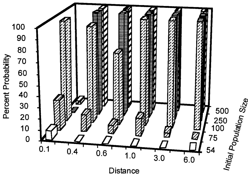
Probability of Subpopulation 1 being alive after 300 generations
