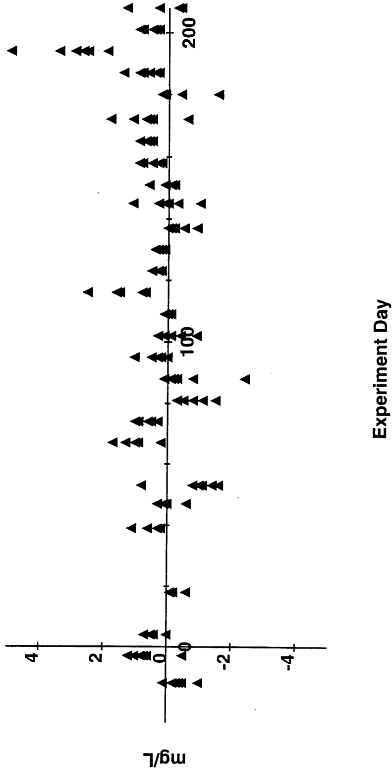
Figure 93a. Water Quality Photosynthesis (Derived from DO) - High Dose
