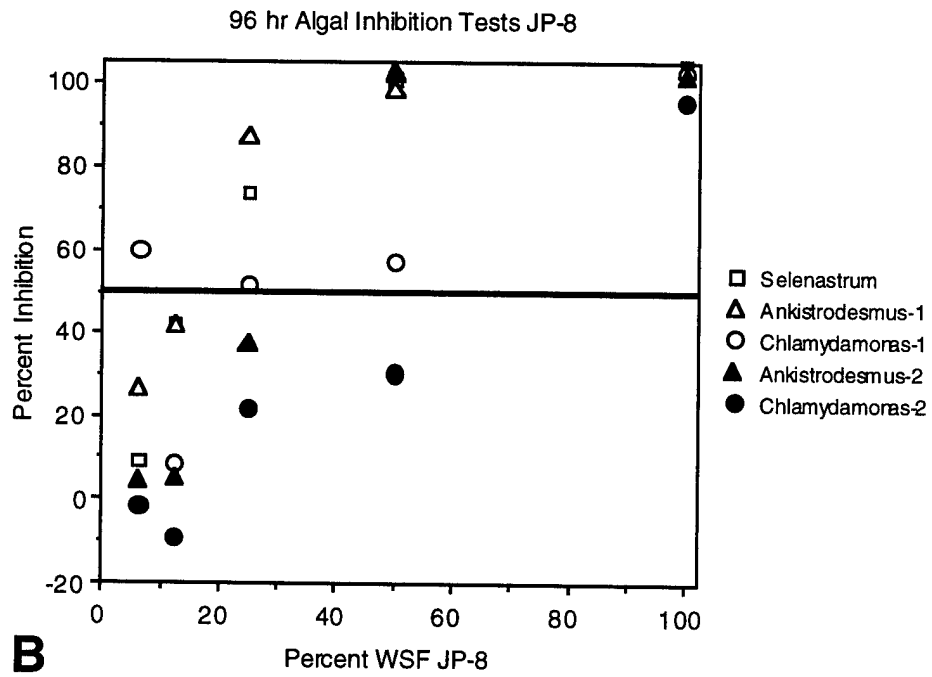
Figure 1. The results of the single species toxicity test results.
