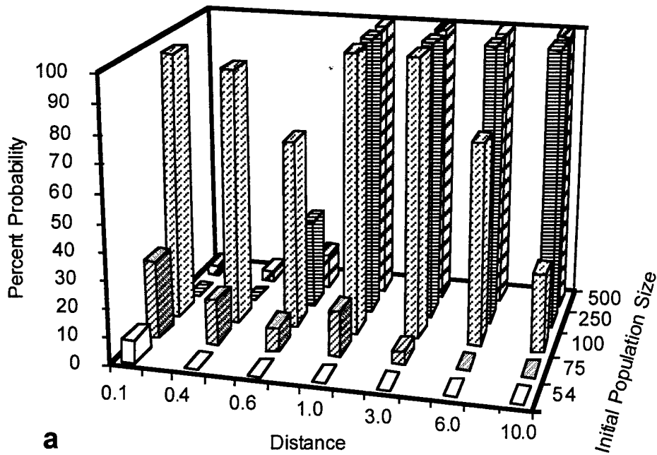
Probability that Subpopulation 1 is not extinct at any time
