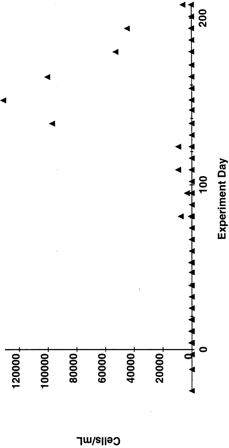
Figure 72b. Phytoplankton - Green Algae Scenedesmus - Mid-dose
