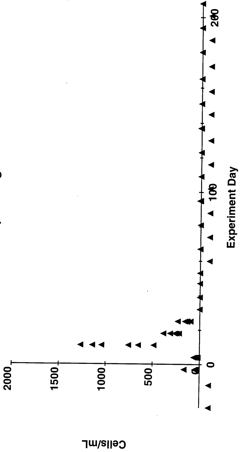
Figure 67a. Phytoplankton - Flagellates Heterotrophs - High Dose
