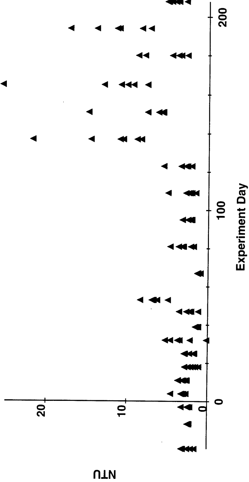
Figure 95a. Water Quality Turbidity - High Dose
