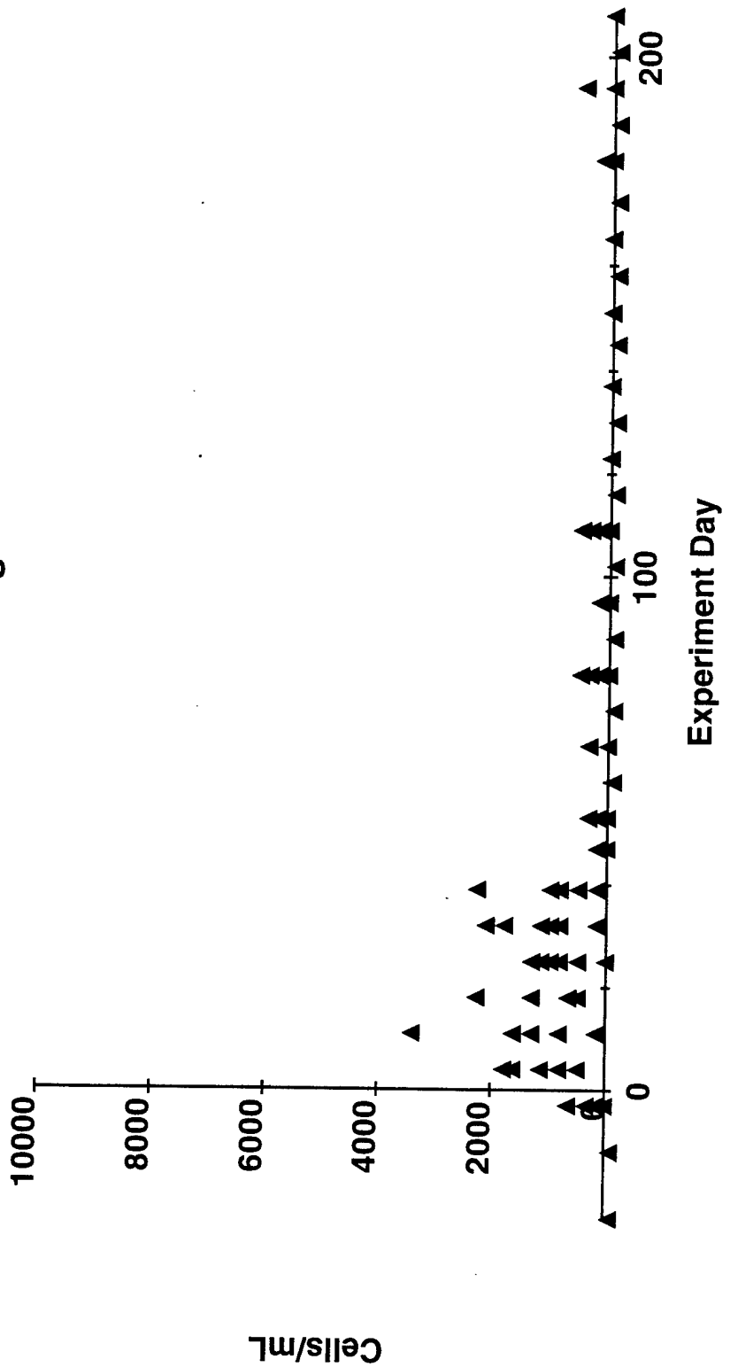
Figure 65a. Phytoplankton - Diatoms Pennate - High Dose
