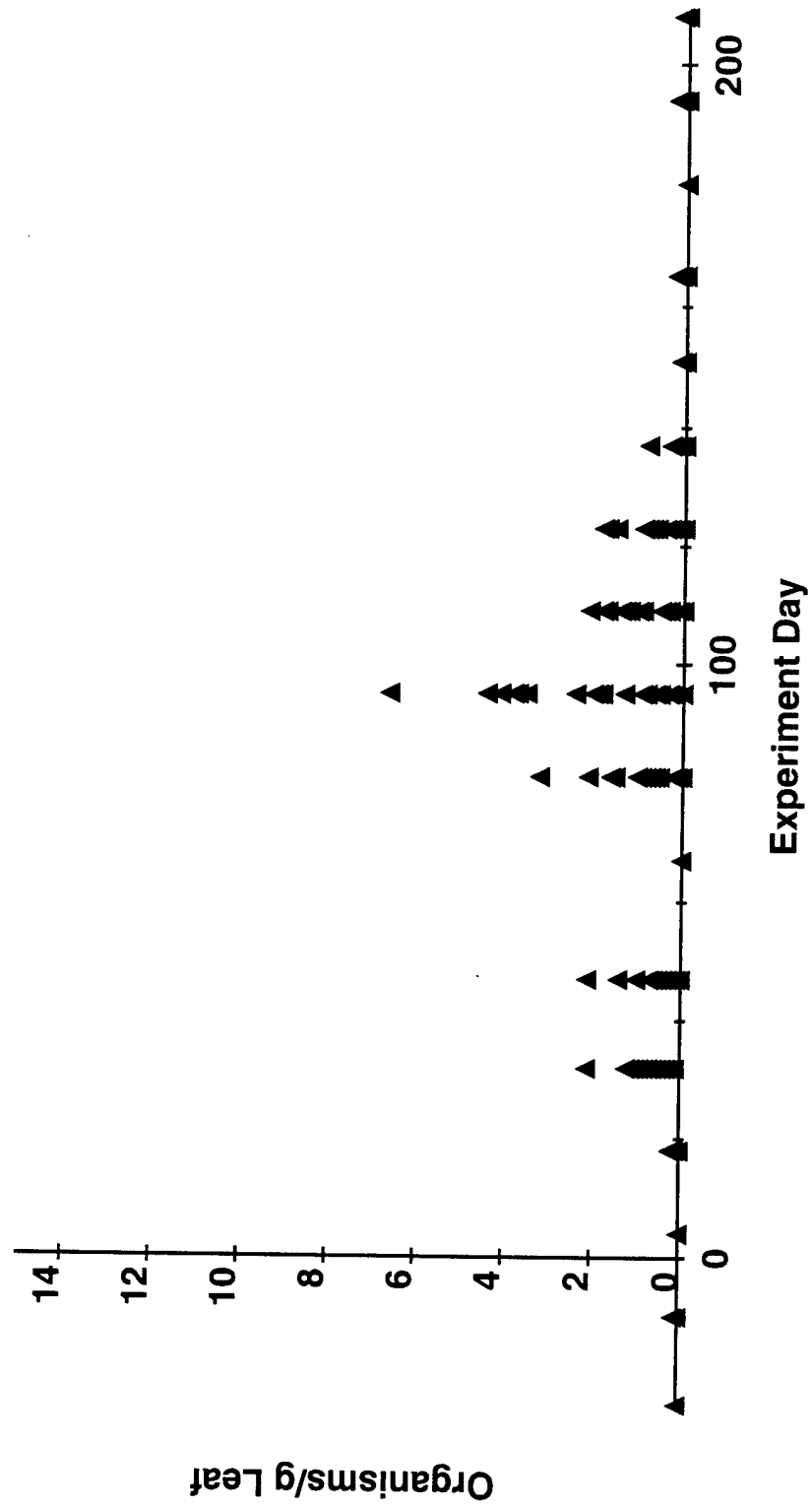
Figure 33c. Crustaceae Daphnia - Low Dose
