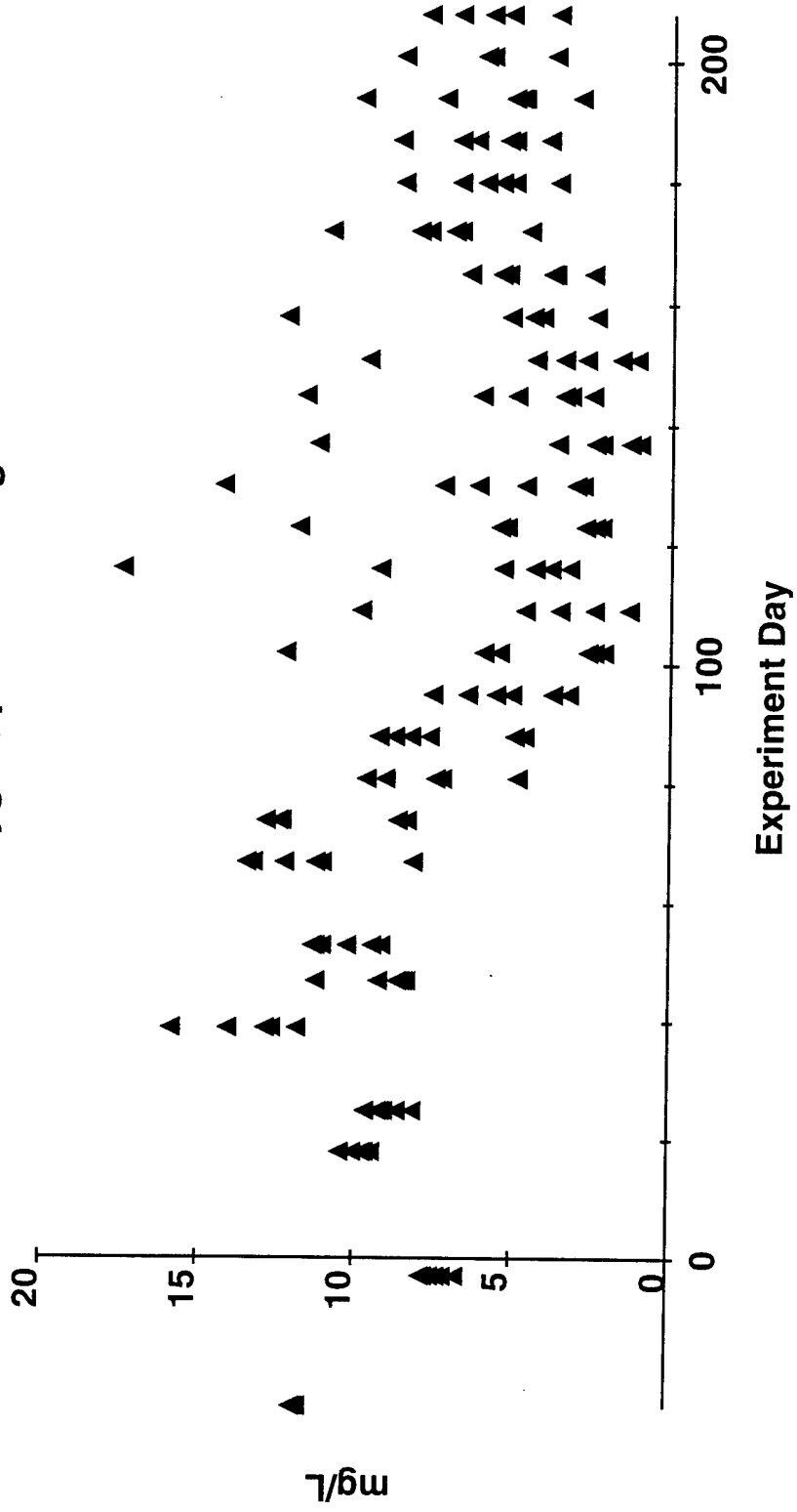
Figure 87a. Water Quality Dissolved Oxygen, pmDO2 - High Dose
