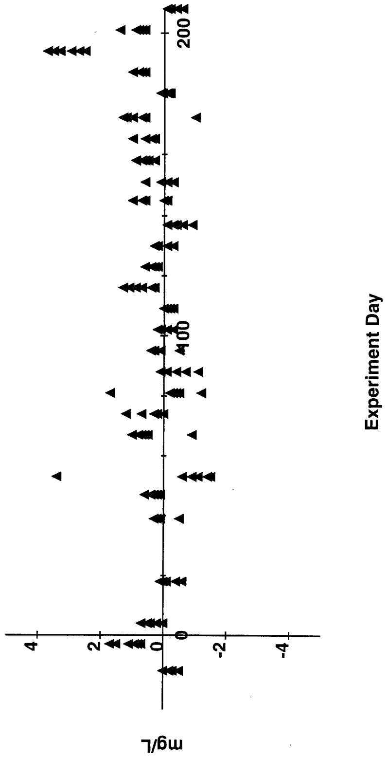
Figure 93c. Water Quality Photosynthesis (Derived from DO) - Low Dose
