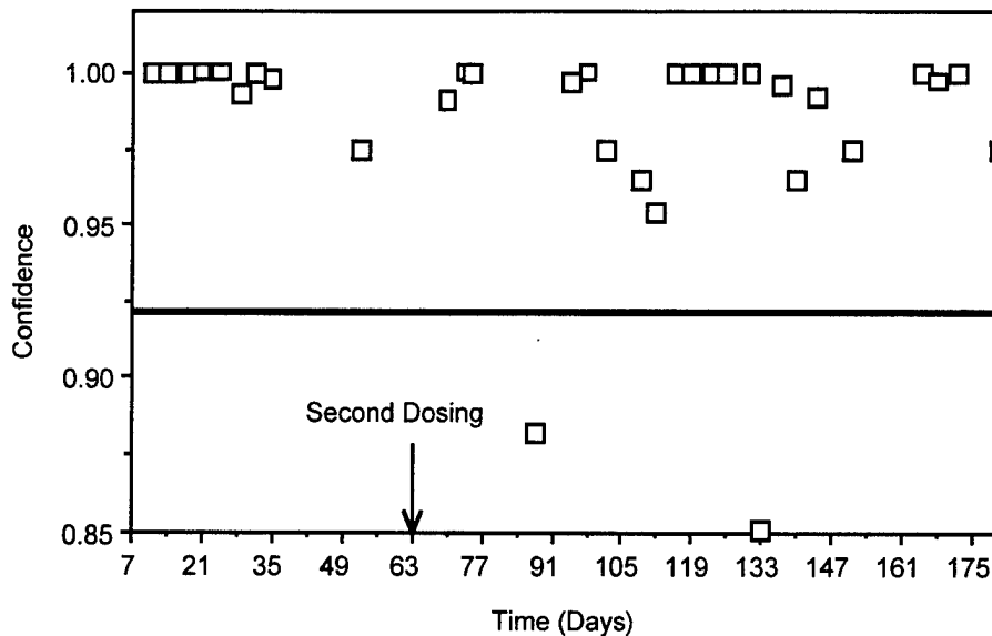
Figure 27. NCAA results for the JP-8/JP-8 experiment. In the initial stages of the experiment the clustering (2 groups) was highly significant with good cluster quality. The pattern was not apparent from day 35 until after the second dosing on day 63. After day 63 the clustering was significant and with good quality until the end of the experiment.
