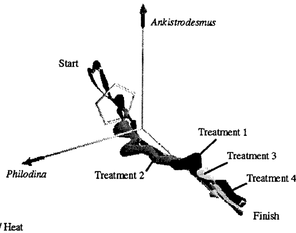
Figure 24. Space-time worm projection of A. falcatus and Philodina populations. Two groups are distinct after dosing with JP-8 showing the algal bloom in the treated microcosms [JP-8 (yellow) and JP-8/heat (red)]. Philodina populations also show a dose effect with the reference (blue) and heat only (green) treatments showing similar dynamics as do the JP-8 dosed treatments. The torus marks day 35.
