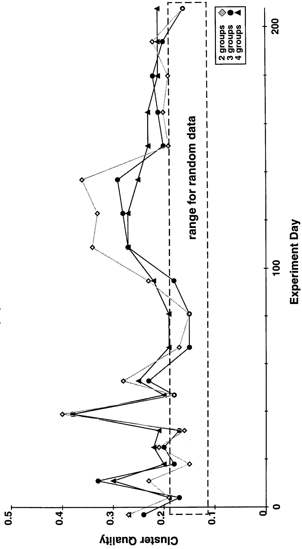
Figure 124. Rifle Cluster Quality Periphyton and Leaf Pack Data
