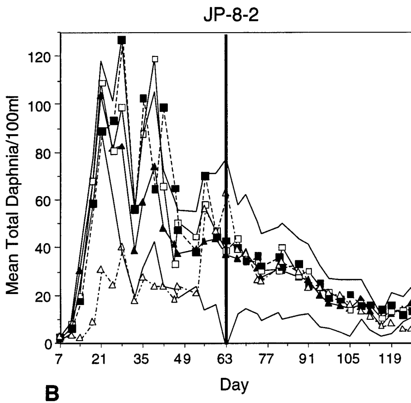
Figure 7. Total Daphnia JP-8-1 and JP-8-2
