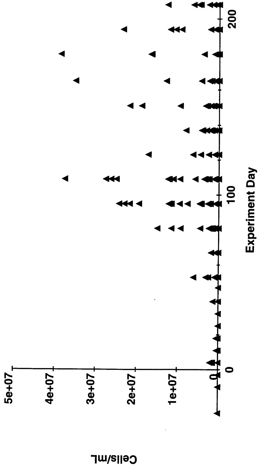
Figure 8c. Periphyton - Cyanophytes Oscillatoria - Low Dose
