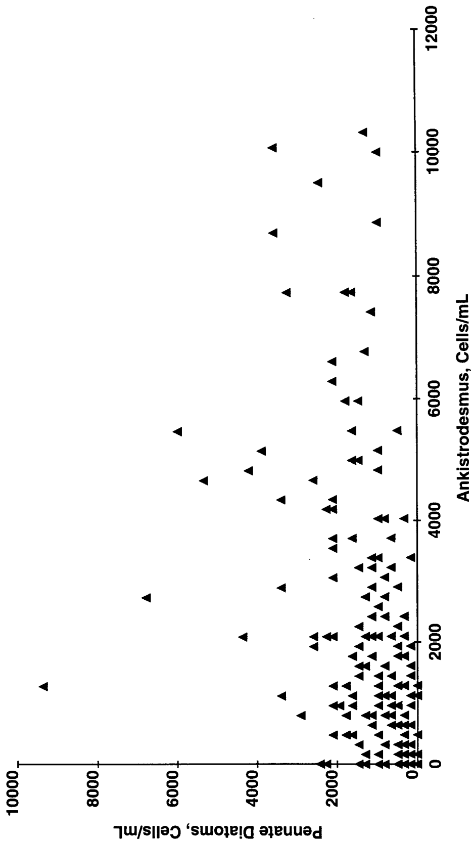
Figure 98. Phytoplankton and Water Quality Correlations Ankistrodesmus vs. Pennate Diatoms
