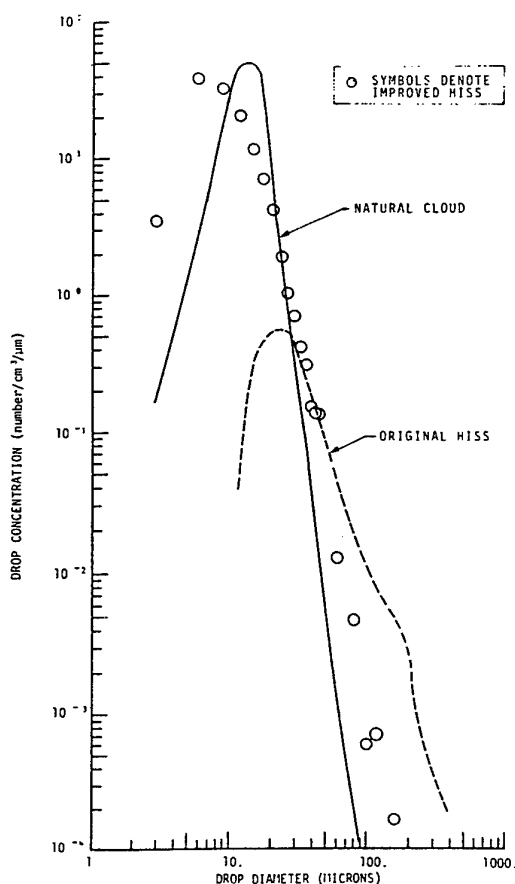
Figure 4.3-8 Drop Size Spectra
