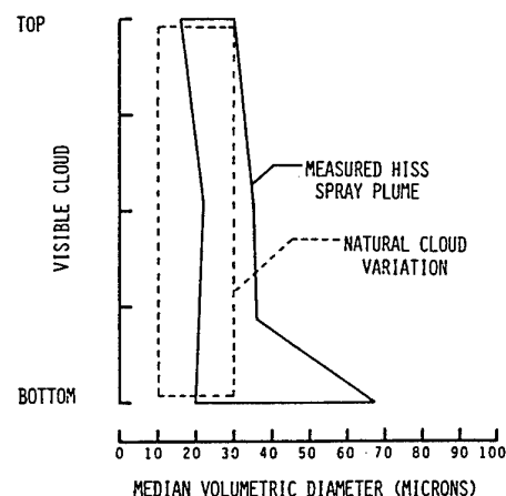
Figure 4.3-6 Vertical Variation-Droplet MVD
