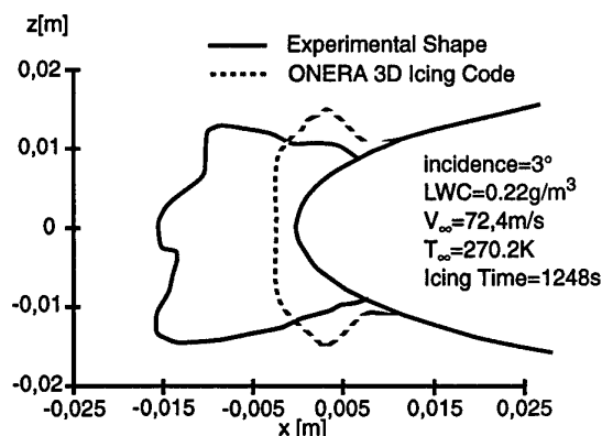
Figure 5-14. Lobster tail effect on an actual ice shape.
