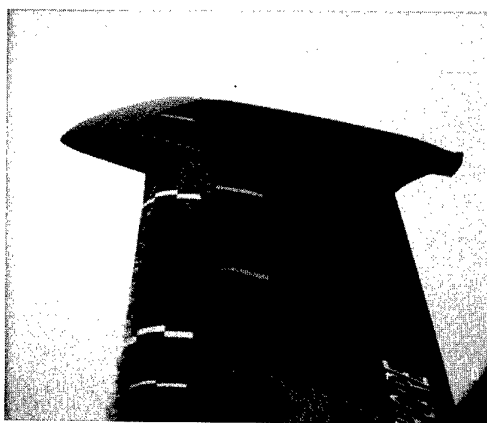
Fig. 3.1-33 Beak ice formation on a rotating main rotor of the EH101 helicopter
