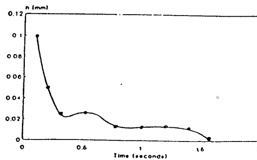
FIG. 29. UPPER SURFACE TIME-DEPENDENT FILM THICKNESS. v_\infty=52 m/s; RR=482 mm/hr; \alpha=7.5^\circ
