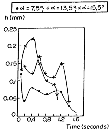
FIG. 28. UPPER SURFACE TIME-DEPENDENT FILM THICKNESS. v_\infty=82 m/s; RR=482 mm/hr
