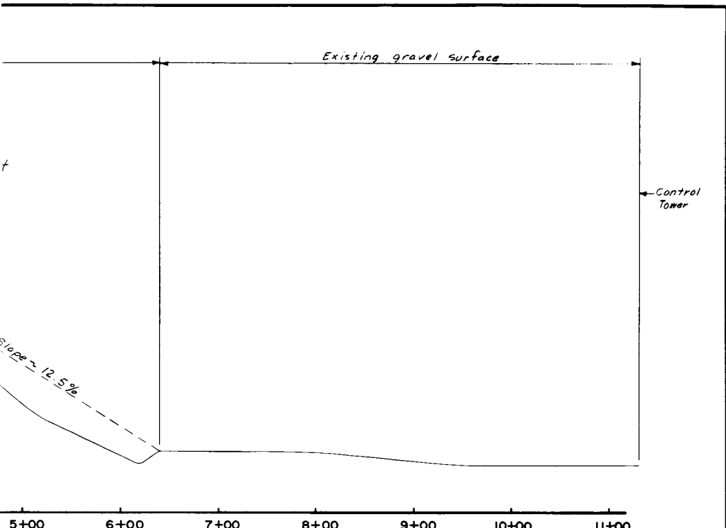
PROFILES TO ACCESS ROAD "H" PROFILE SCALES: HOR. 1" = 50' VERT. 1" = 10'
