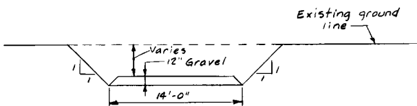
SECTION FOR PROPOSED IMPROVEMENTS TO ACCESS ROADS "C" AND "D" SCALE: 1" = 5'
