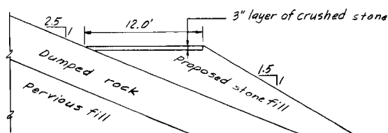
TYPICAL ROCK FILL SECTION FOR PROPOSED DAM ACCESS ROAD "E" SCALE: 1" = 5'
