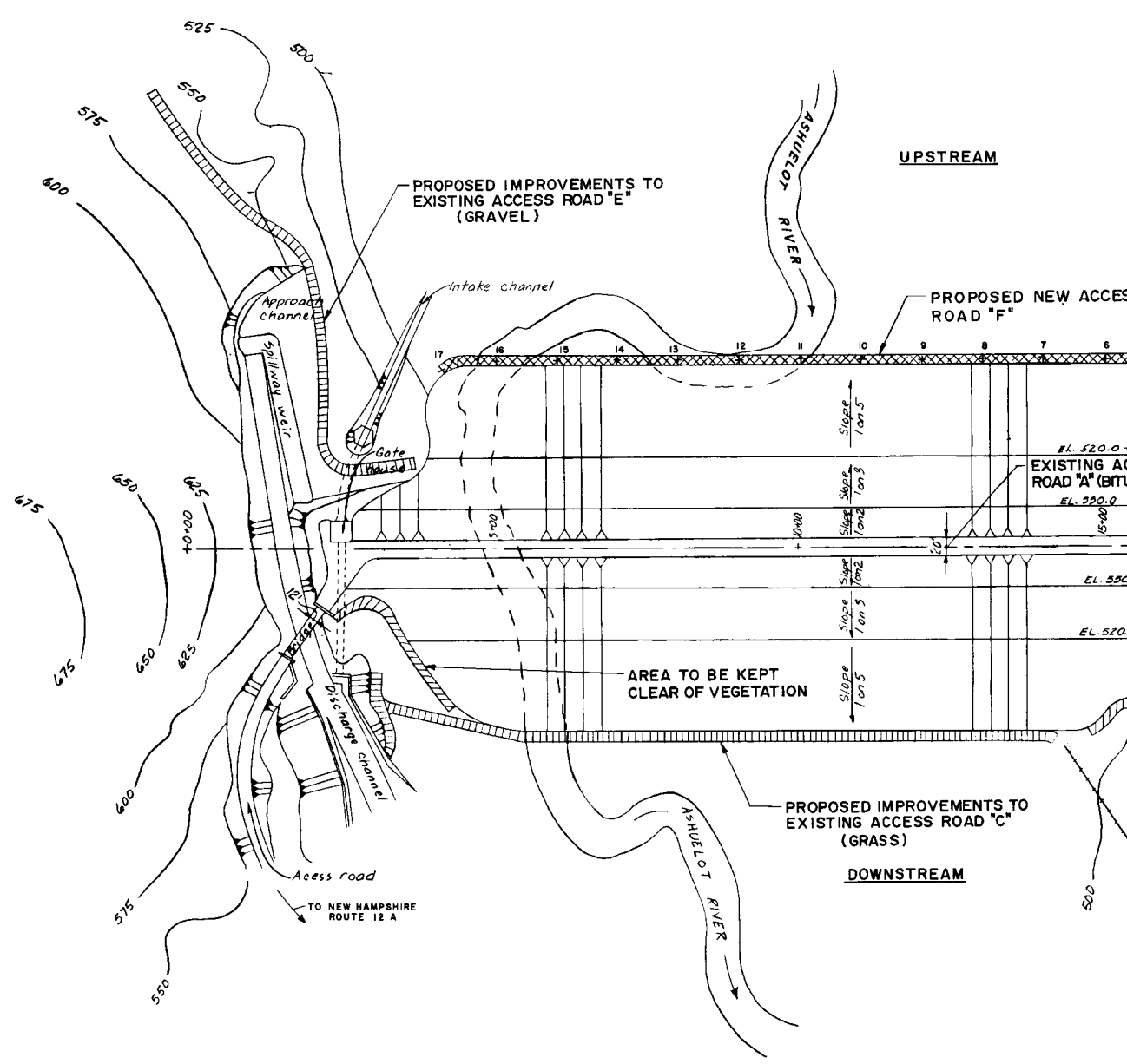
GENERAL PLAN SCALE: 1" = 100'
