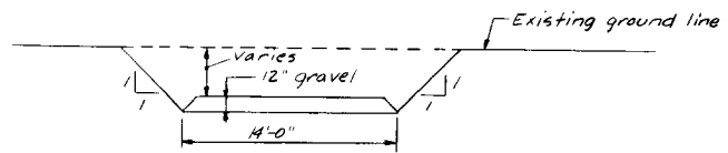
TYPICAL CUT SECTION FOR PROPOSED ACCESS ROADS "G", "H", "N", "I", "L" SCALE: 1" = 5'
