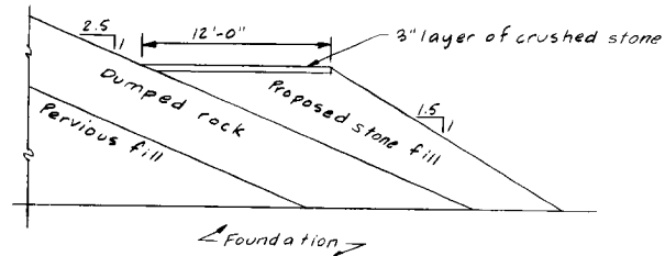
TYPICAL ROCK FILL SECTION FOR PROPOSED DAM ACCESS ROAD "N" SCALE: 1" = 5'
