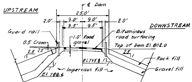
TYPICAL SECTION FOR EXISTING ACCESS ROAD "A" SCALE: 1" = 10'
