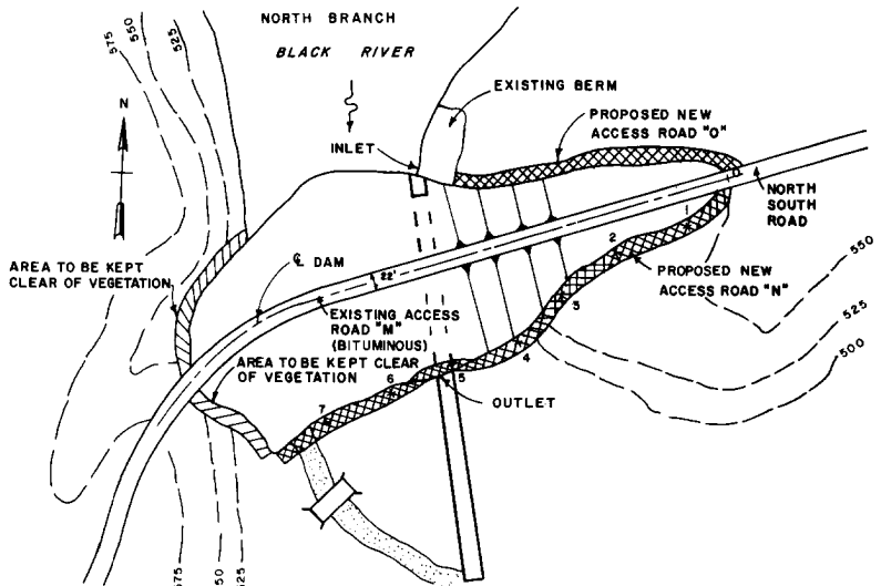
NORTH BRANCH DAM PLAN N.T.S.
