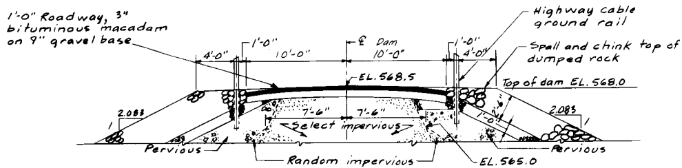
TYPICAL SECTION FOR ACCESS ROAD "A"
