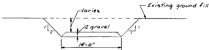
TYPICAL CUT SECTION FOR PROPOSED ACCESS ROADS "C" AND "F" SCALE: 1" = 5'
