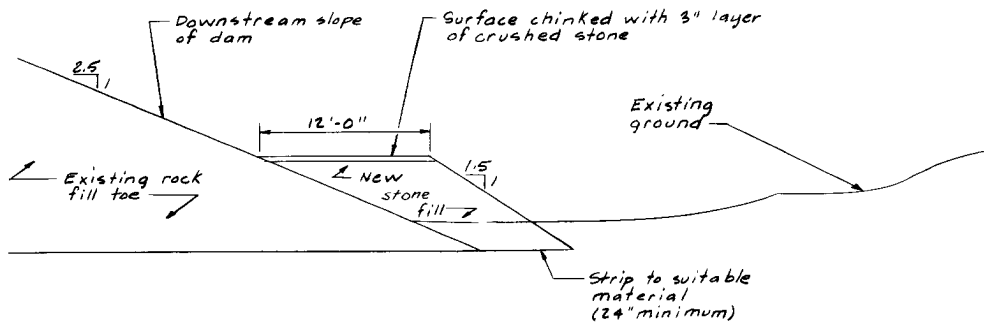
TYPICAL ROCK FILL SECTION FOR PROPOSED ACCESS ROADS "C" AND "F"
