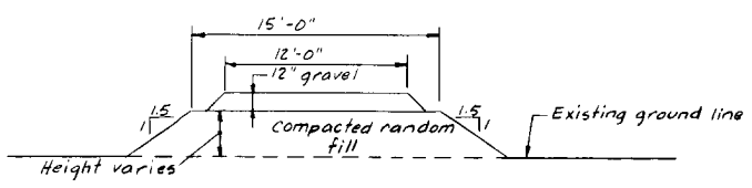
TYPICAL FILL SECTION FOR PROPOSED ACCESS ROADS "H" SCALE: 1" = 5'
