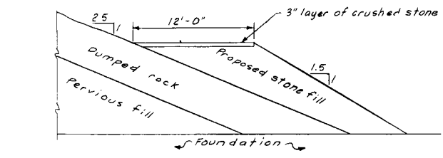
TYPICAL FILL SECTION FOR PROPOSED DAM ACCESS ROAD "F" SCALE: 1" = 5'
