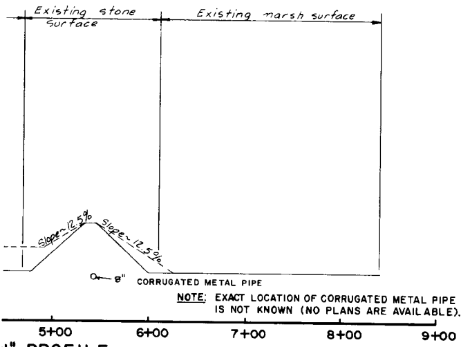
1" PROFILE 1" 1"
