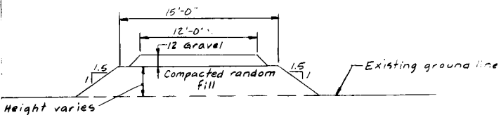
SECTION FOR PROPOSED IMPROVEMENTS TO ACCESS ROADS "C" AND "D" SCALE: 1" = 5'
