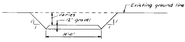
CUT SECTION FOR PROPOSED ACCESS ROADS "G", "H", "N", "I", "L", "K", AND "O" SCALE: 1" = 5'
