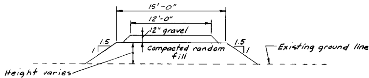
TYPICAL FILL SECTION FOR PROPOSED ACCESS ROADS "C" SCALE: 1" = 5'
