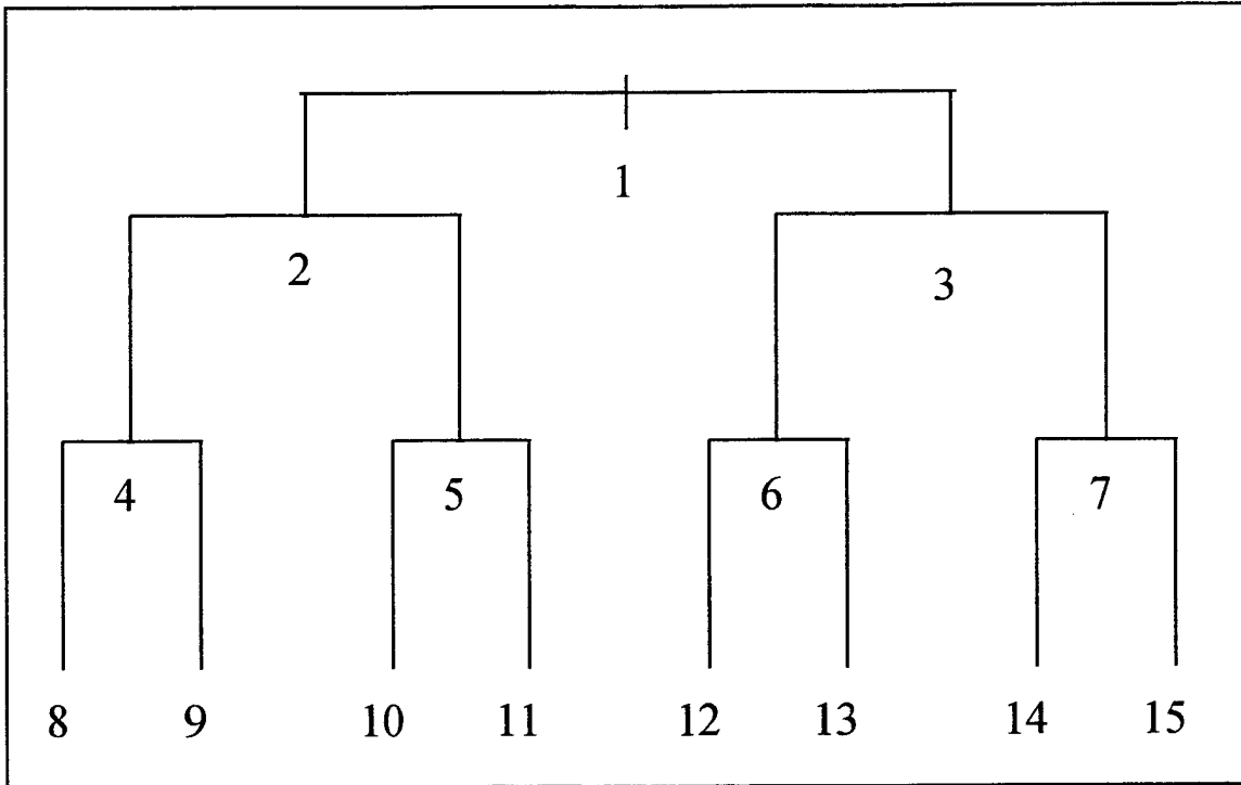
Figure 3.1 Full Binary Tree With Numbered Nodes
