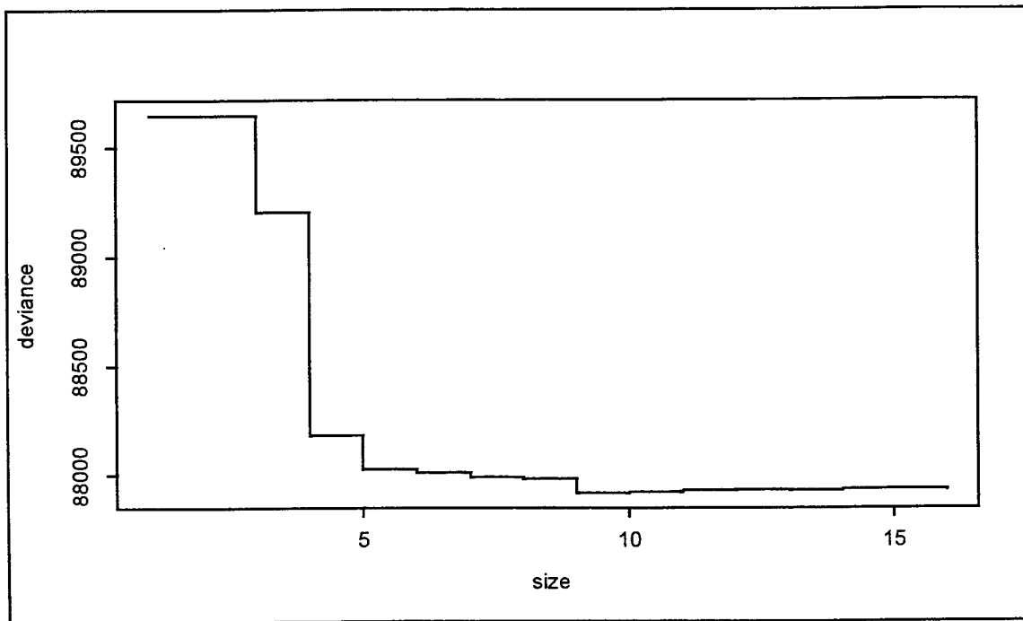
Figure 4.3 Cross-Validation Plot When 4 Attributes Included Using C*-Group Data
