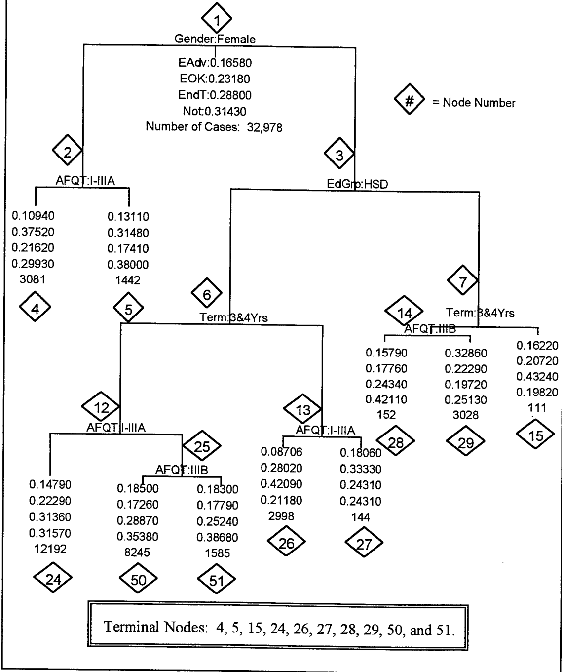
Figure 4.4 Pruned Classification Tree Using C*-Group Data With 4 Attributes
