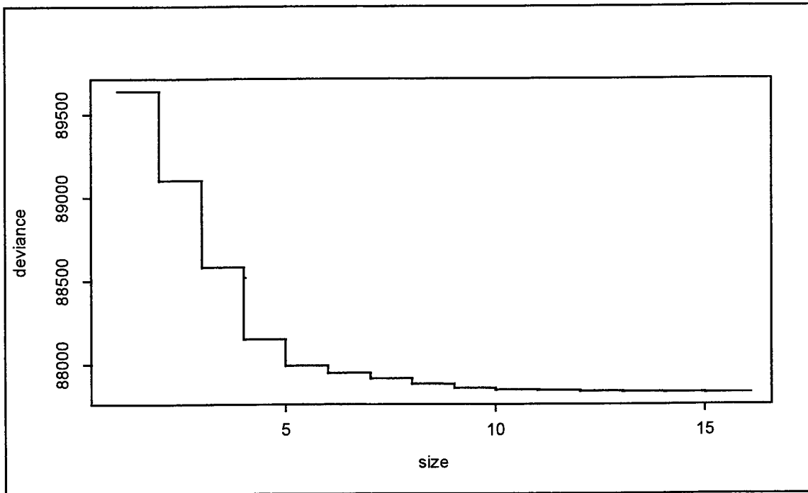
Figure 4.2 Pruning Plot When 4 Attributes Included Using C*-Group Data
