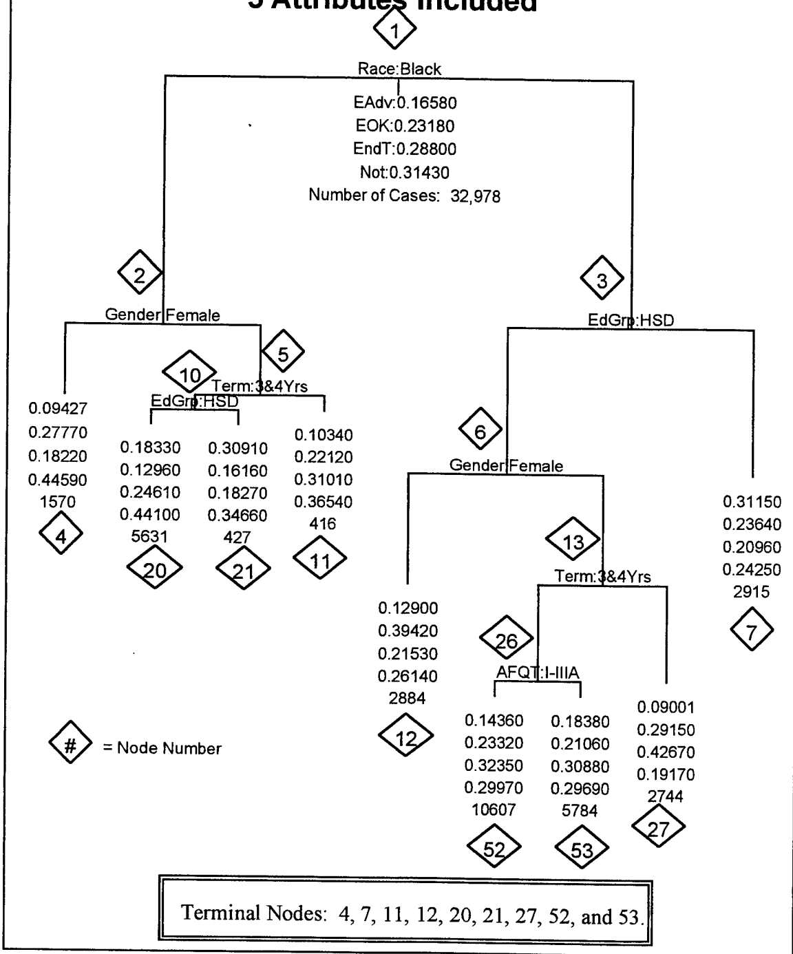
Figure 4.8 Pruned Classification Tree Using C*-Group Data With 5 Attributes
