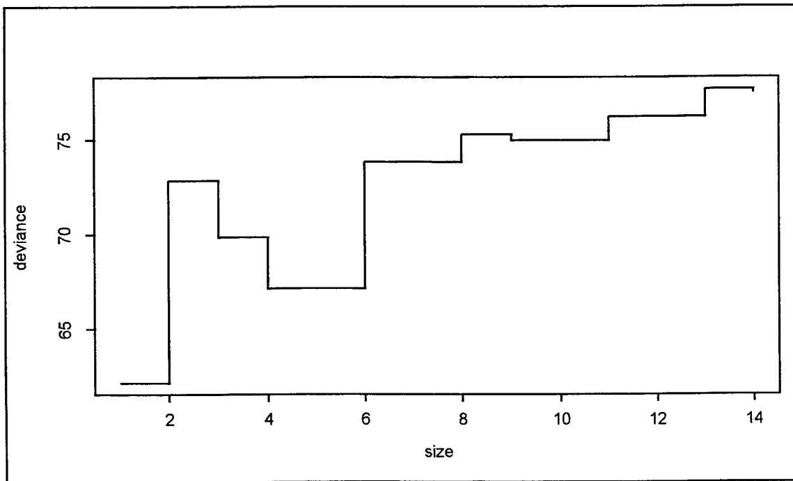
Figure 3.6 Cross-Validation Plot for Example
