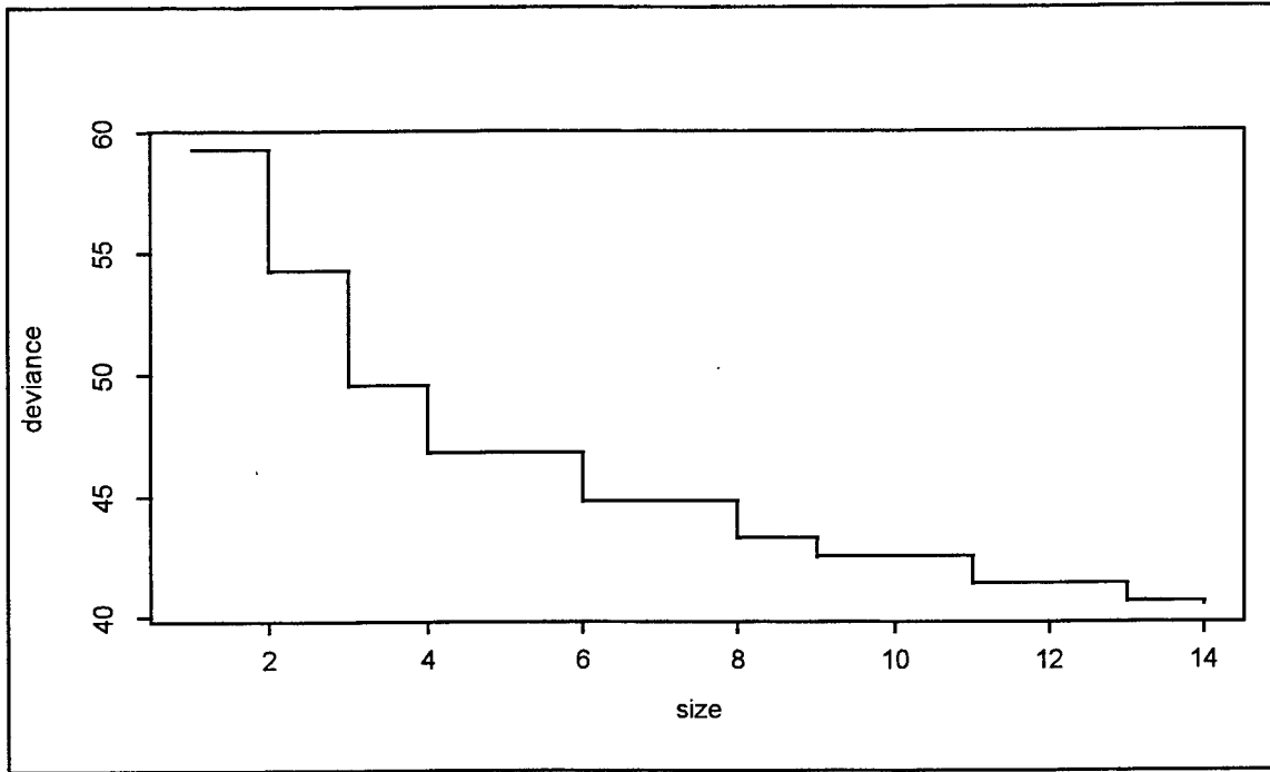
Figure 3.5 Pruning Plot for Example
