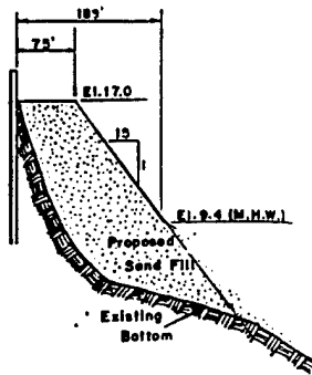
TYPICAL SECTION BEACH FILL
