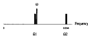
(d) Atom is slightly detuned from the first mode.
