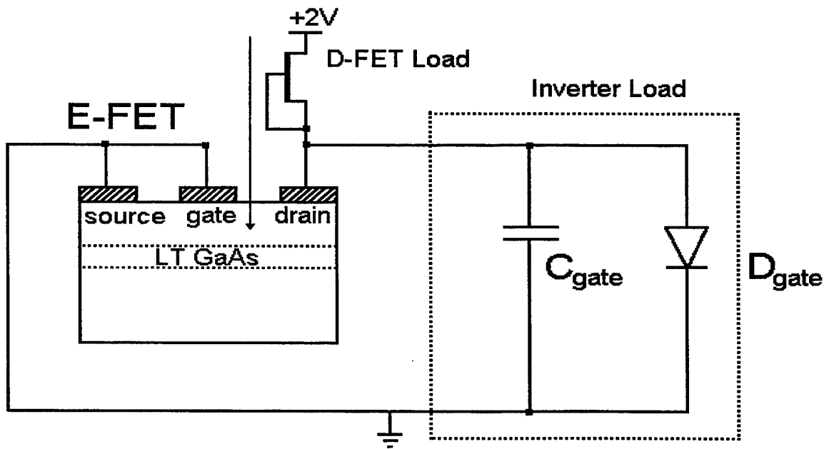
Figure 3.3 Circuit Layout for Inverter Simulation. The ion strike occurs between the gate and the drain of the MESFET.
