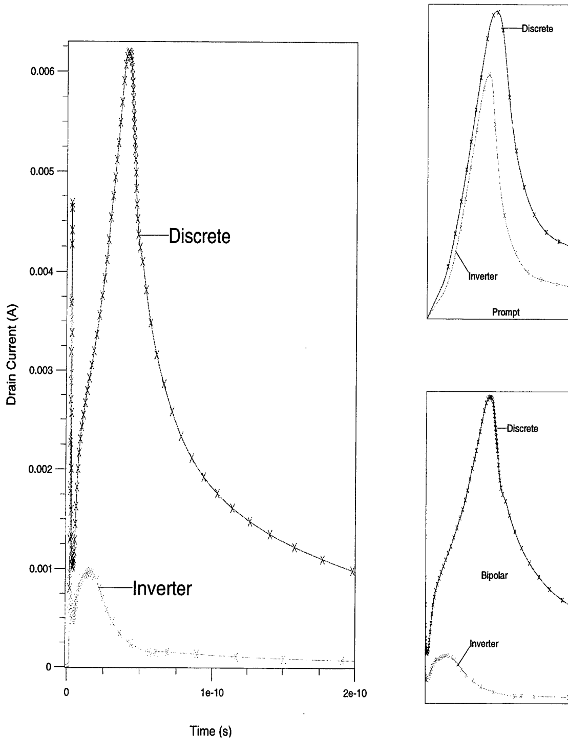
Figure 4.2 EFET drain current of a discrete and inverter SEU simulations. The graph on the left shows the form of the entire event and the smaller graphs give better resolution of the first two peaks. The prompt peak goes from 2 to 3 ps, and the bipolar peak goes from 3 to 30 ps.
