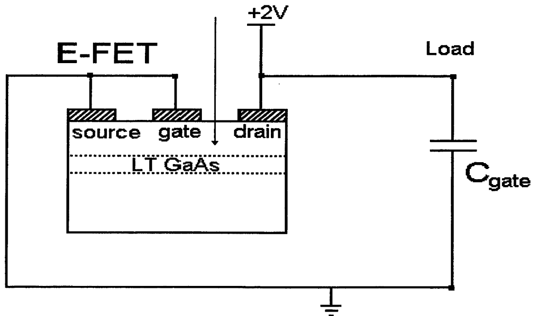
Figure 3.2 Circuit Layout for Discrete Transistor Simulation. The ion strike occurs between the gate and the drain of the MESFET.
