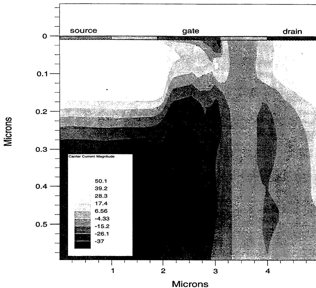
Figure 4.5 Cross-section of the conventional E-FET current densities. Positive values in the plot are regions of high electron current density, negative values are regions of high hole current density. Notice electron current dominates along the surface of the transistor due to photo-conductivity.
