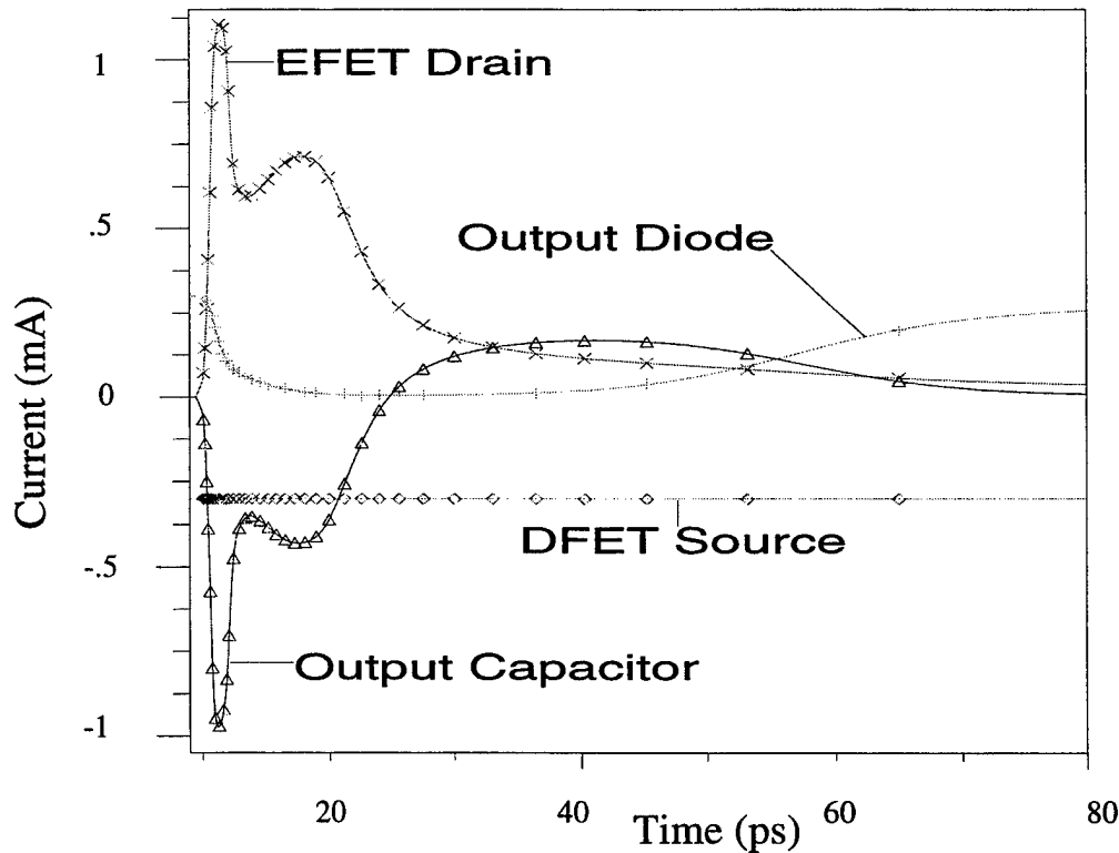
Figure 4.3 . Currents of the E-FET drain, gate diode, capacitor and active load.
