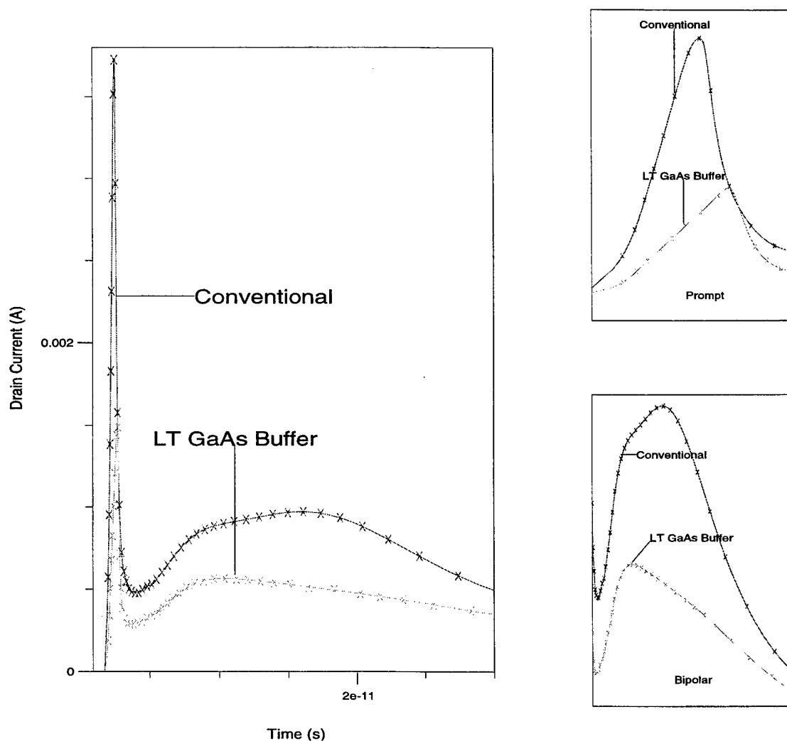
Figure 4.7 EFET drain current of an inverter SEU simulations, one with a conventional EFET and the other with LT GaAs Buffered EFET. The graph on the left shows the form of the entire event and the smaller graphs give better resolution of the first two peaks. The prompt peak goes from 2 to 3 ps, and the bipolar peak goes from 3 to 30 ps.
