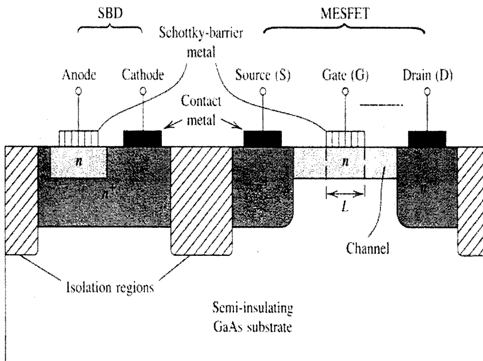
Figure 2.1 Generic representation of the fabrication of GaAs Metal-Semiconductor devices: Schottky-Barrier Diode (SBD) on the left and a MESFET on the right. From [1]
