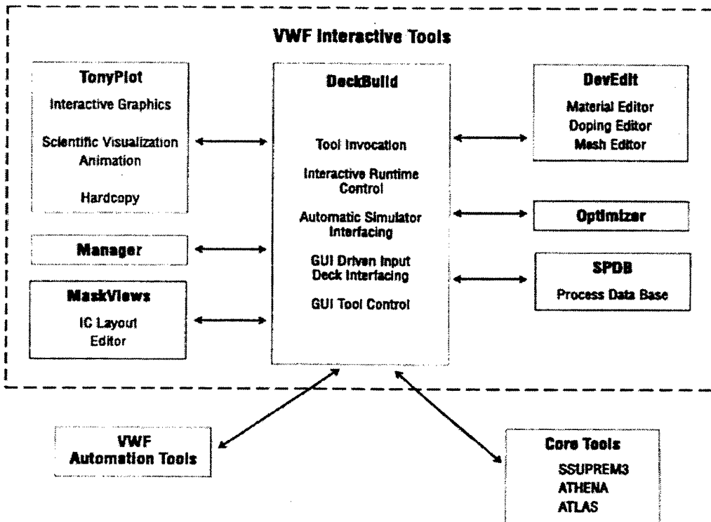
Figure 3.1 Silvaco VWF Framework from Ref. [10]
