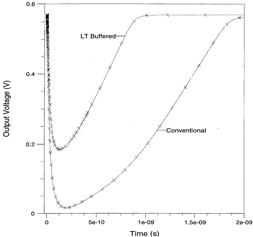
Figure 4.8 EFET drain voltage of an inverter SEU simulations, one with a conventional EFET and the other with LT GaAs Buffered EFET.
