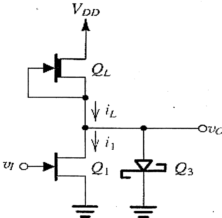
Figure 2.3 Schematic diagram of a GaAs DCFL Inverter. An EFET with DFET active load, driving a SBD that models the gate of the next EFET/DFET inverter. From [1]
