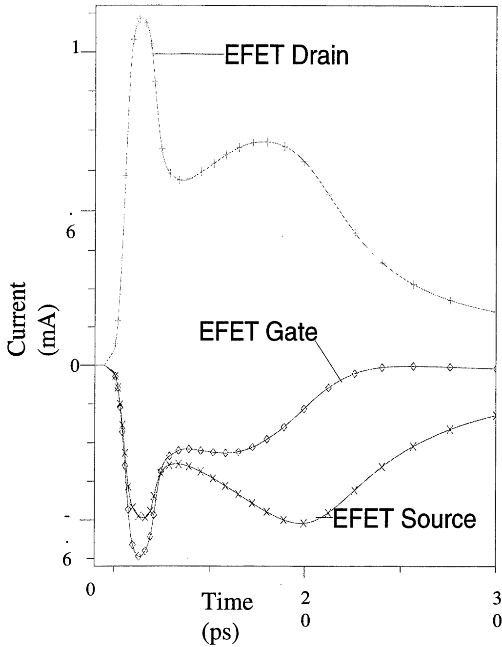
Figure 4.4 Terminal currents of the E-FET.
