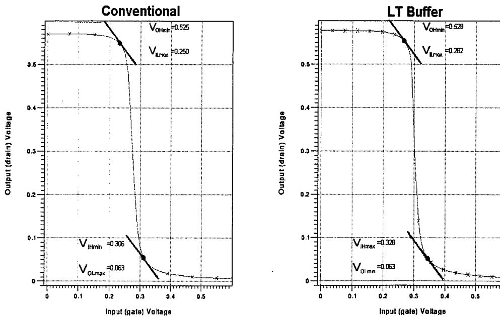
Figure 4.1 Inverter DC transfer characteristics using standard (left) and LT buffered (right) EFETs.
