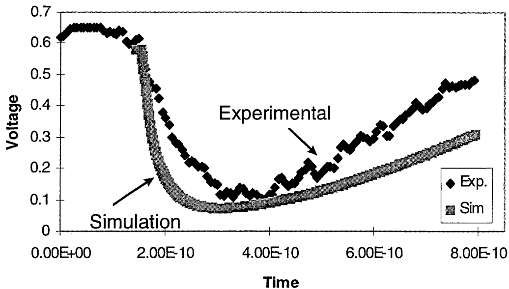
Figure 4.11 Output voltage of an inverter during an SEU. Experimental measurement and computer simulation results presented.
