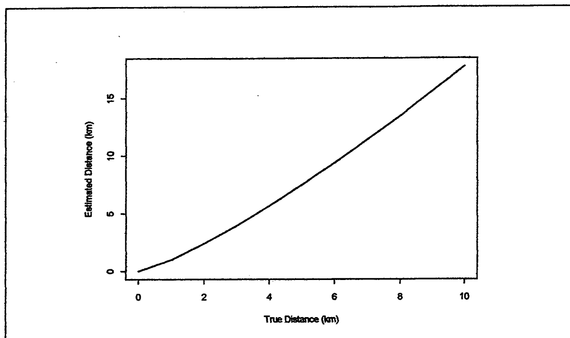
Figure 2. Estimated Distance v. True Distance, \text{Estimated distance} = (\text{true distance})^{1.25}
