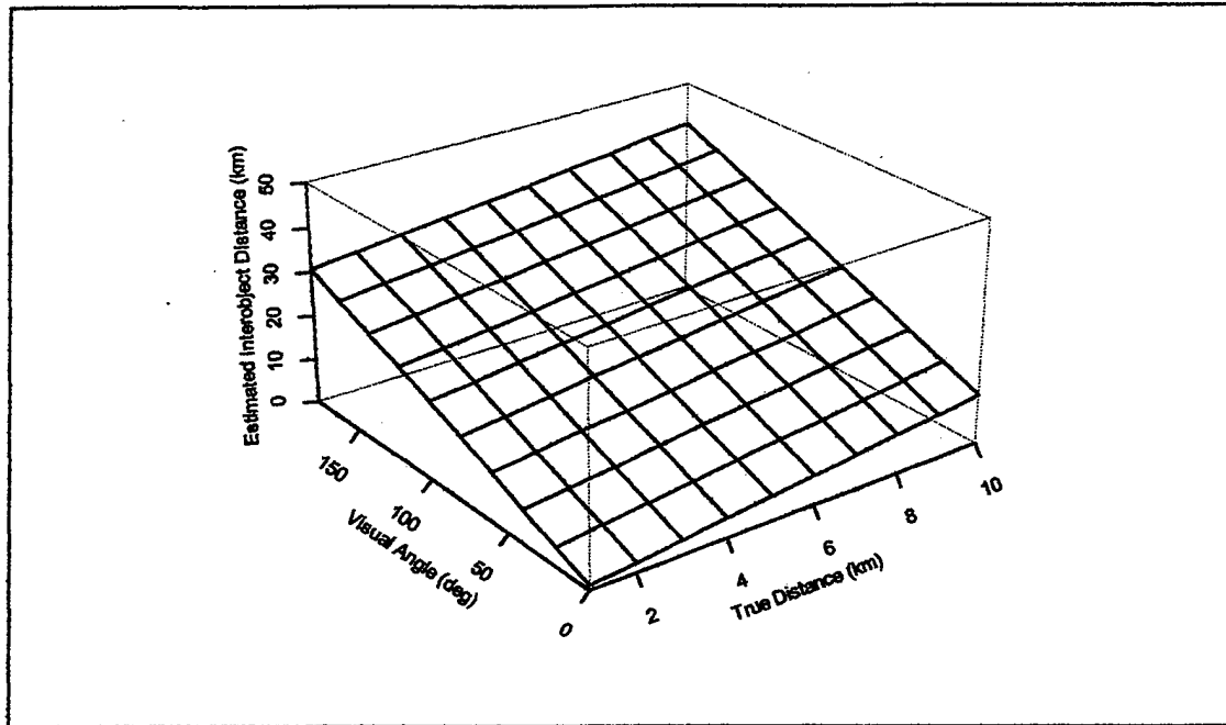
Figure 5. Estimated Interobject Distance (eid) v. Visual Angle (va) and True Interobject Distance (tid), \text{eid} = (1.108 * \text{tid}) + (0.164 * \text{va}).
