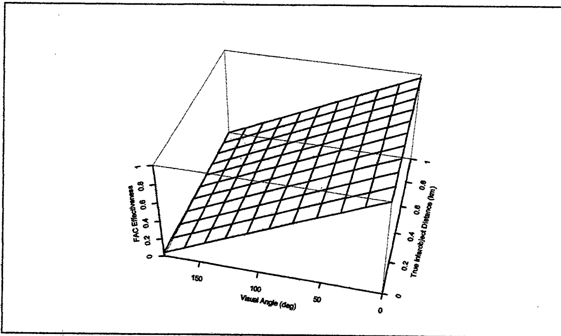
Figure 7. Second View of FAC Effectiveness v. True Interobject Distance (km) and Visual Angle (degrees), A_F = \text{FAC Effectiveness} = 1 - \left[ \frac{1}{30.63} * (1.108 * tid + 0.164 * va) \right] .
