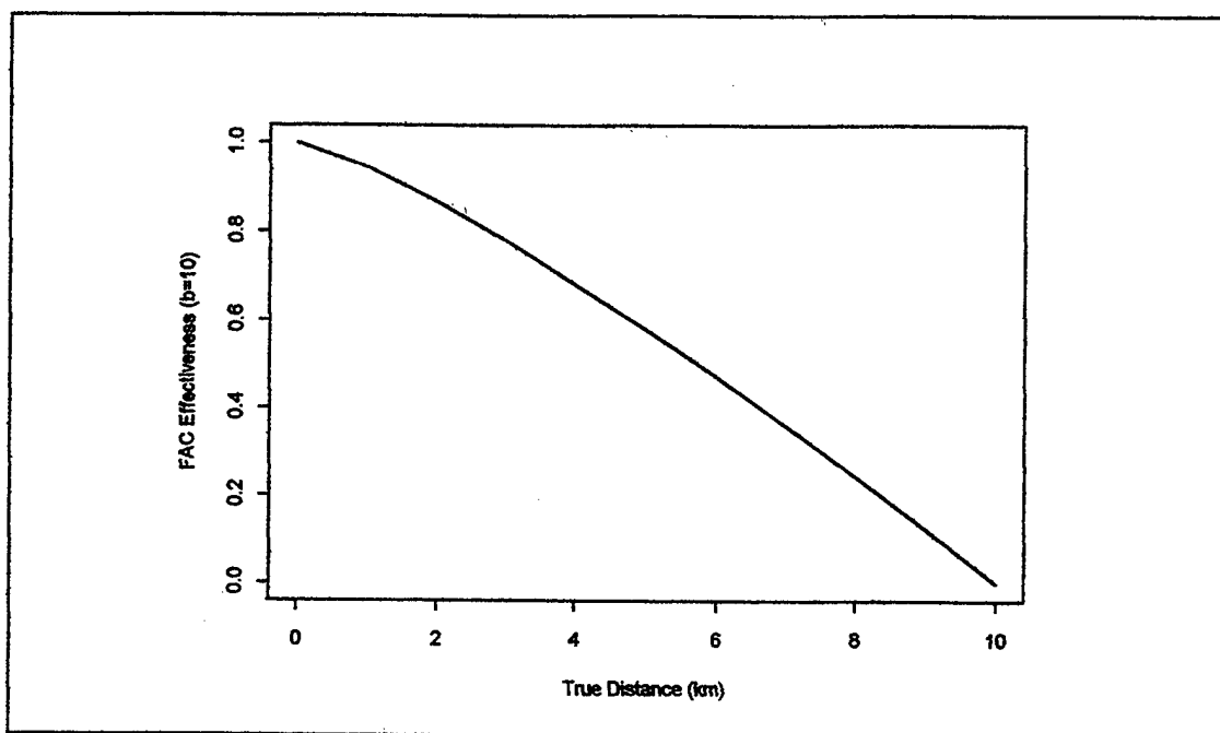
Figure 3. FAC Effectiveness v. True Distance, A_H = \text{FAC Effectiveness} = 1 - \left( \frac{\text{true distance}}{b} \right)^{1.25} , b = 10 .
